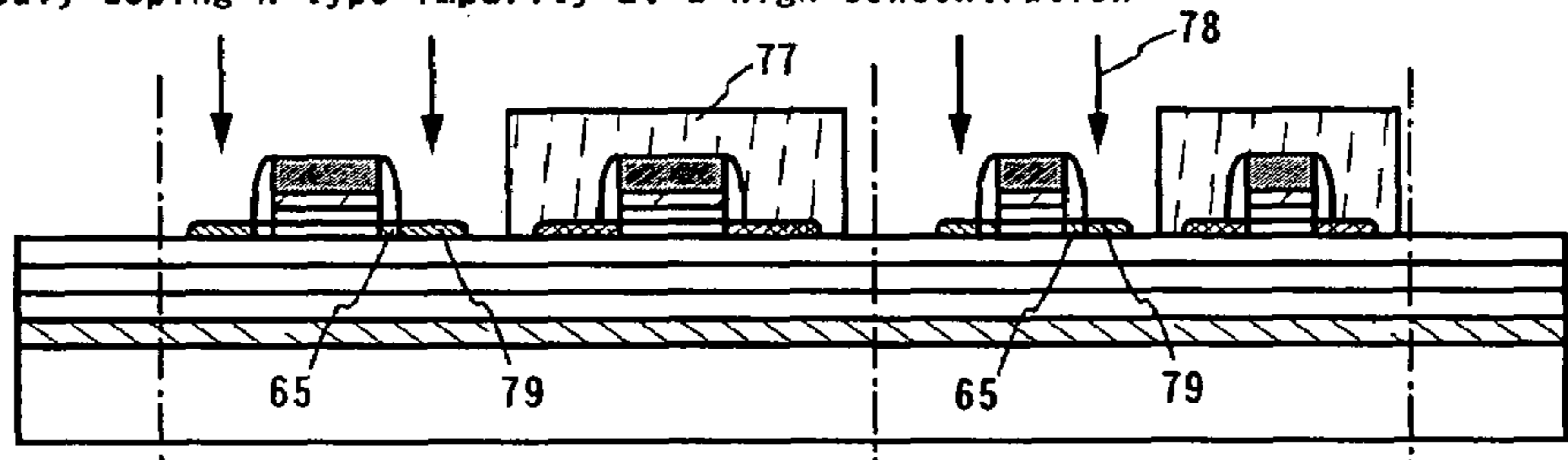
FIG. 23H heavy doping N-type impurity at a high concentration
