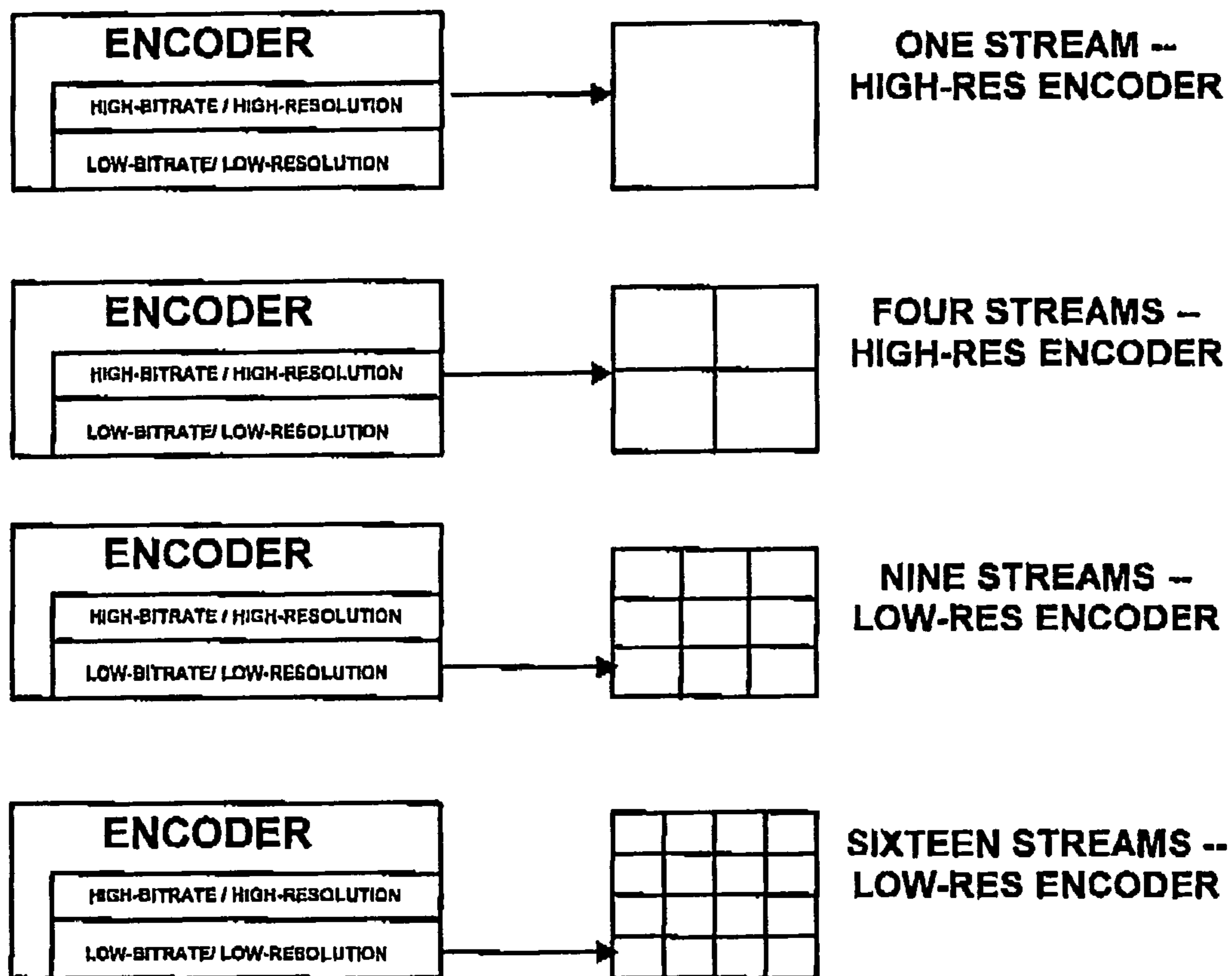
FIG. 4 -- BANDWIDTH CONSERVATION
