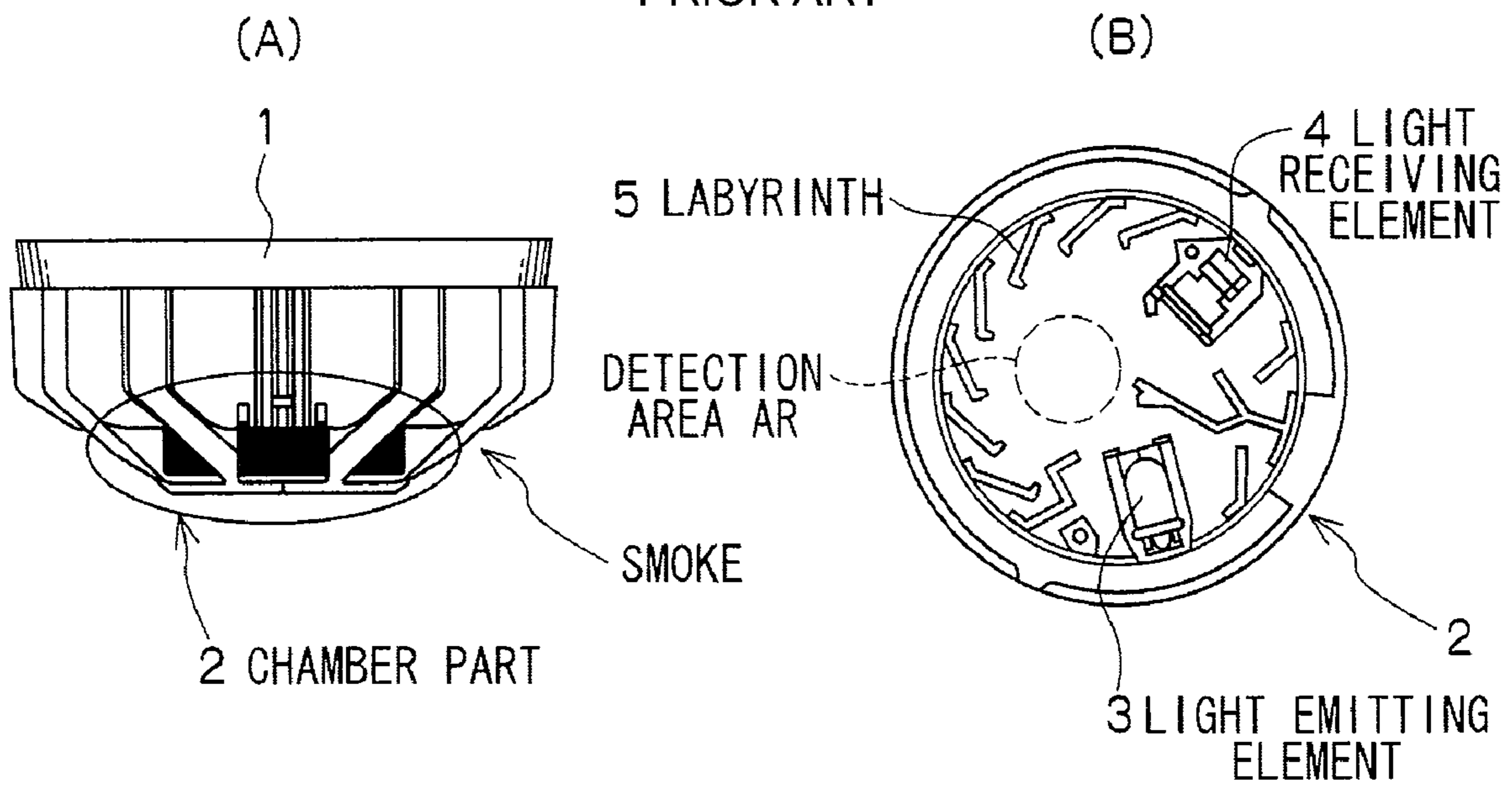
FIG.4 PRIOR ART
