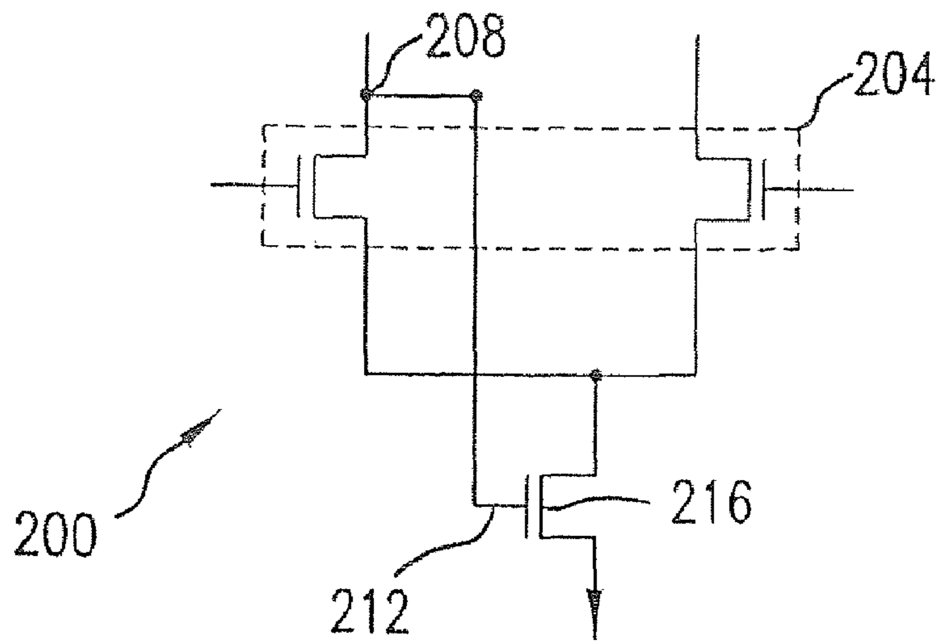
FIG. 2 PRIOR ART
