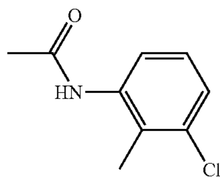
1A. 3-Chloro-2-methylphenylacetamide
