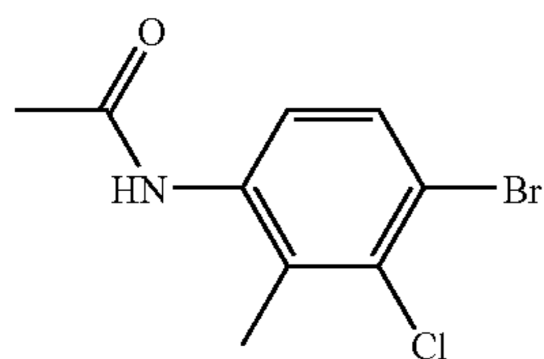
1B. 4-Bromo-3-chloro-2-methylphenylacetamide
