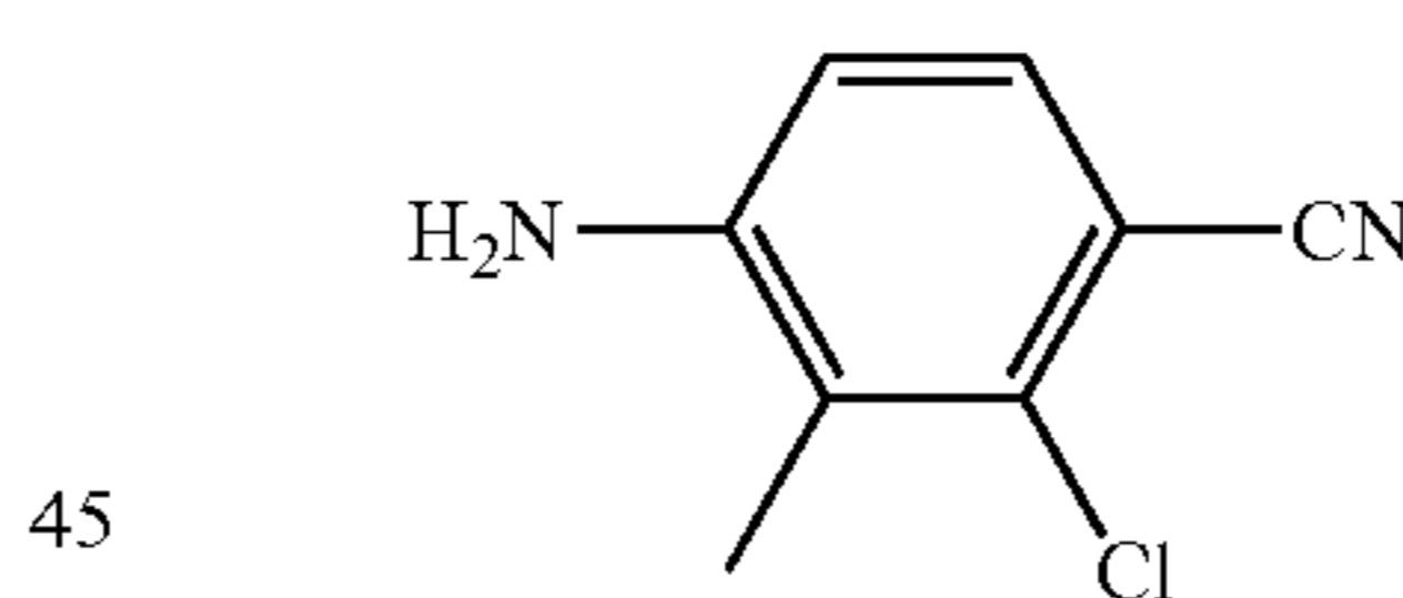
1D. 3-Chloro-4-cyano-2-methylphenylaniline
