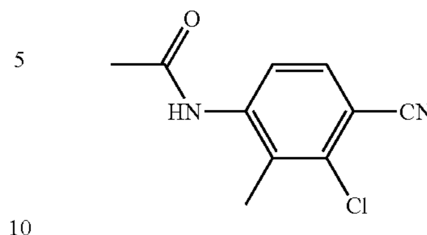
1C. 3-Chloro-4-cyano-2-methylphenylacetamide
