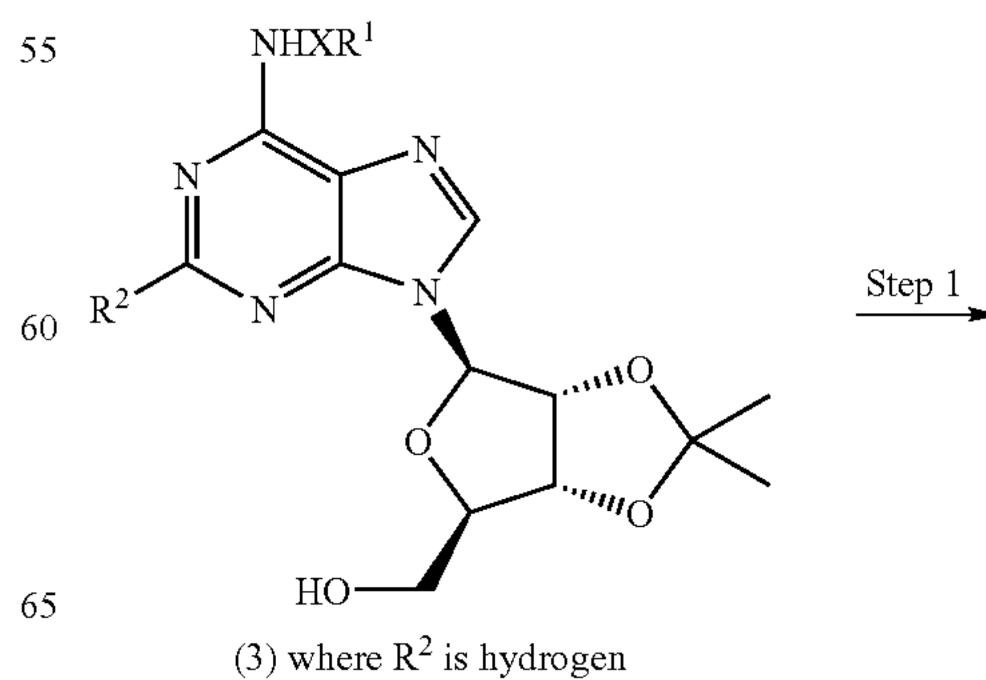
REACTION SCHEME V
