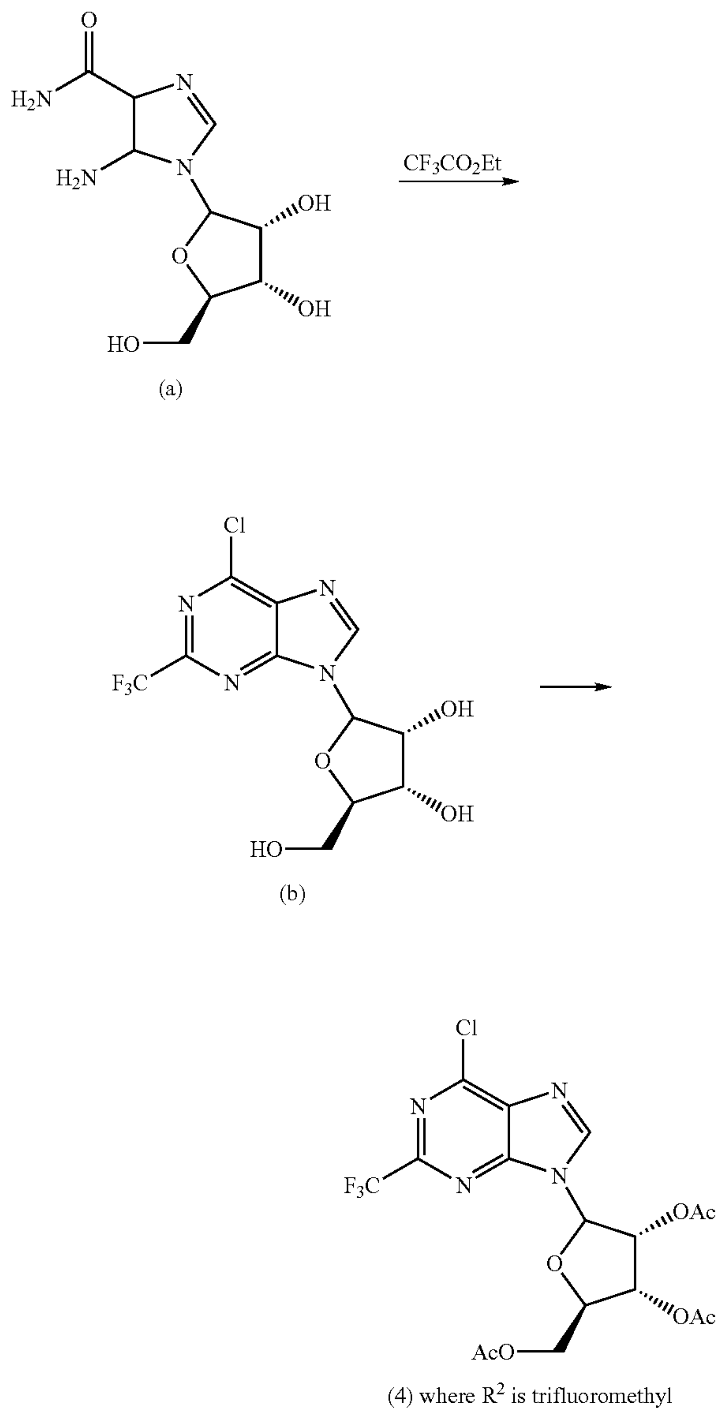
REACTION SCHEME III
