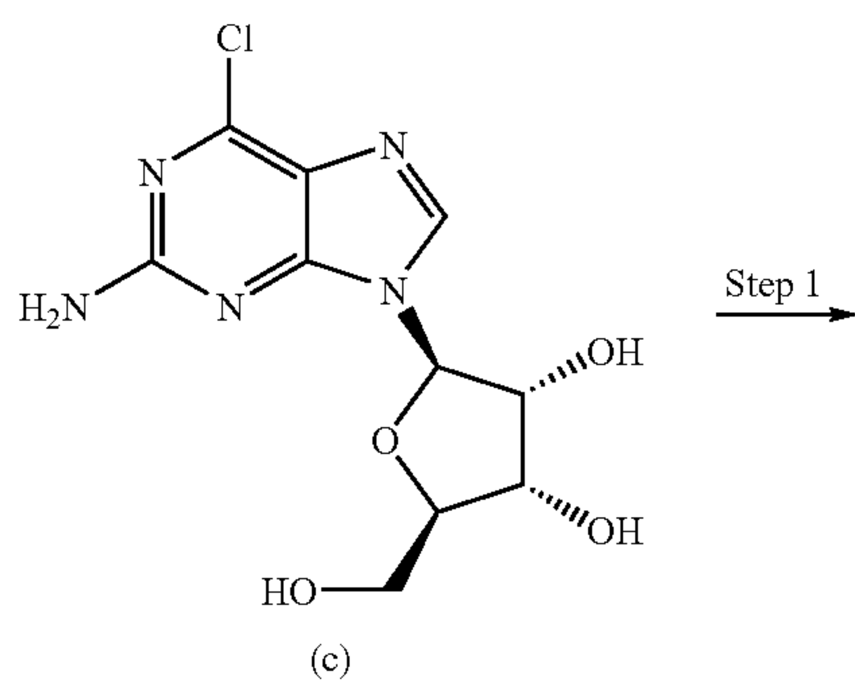
REACTION SCHEME IV
