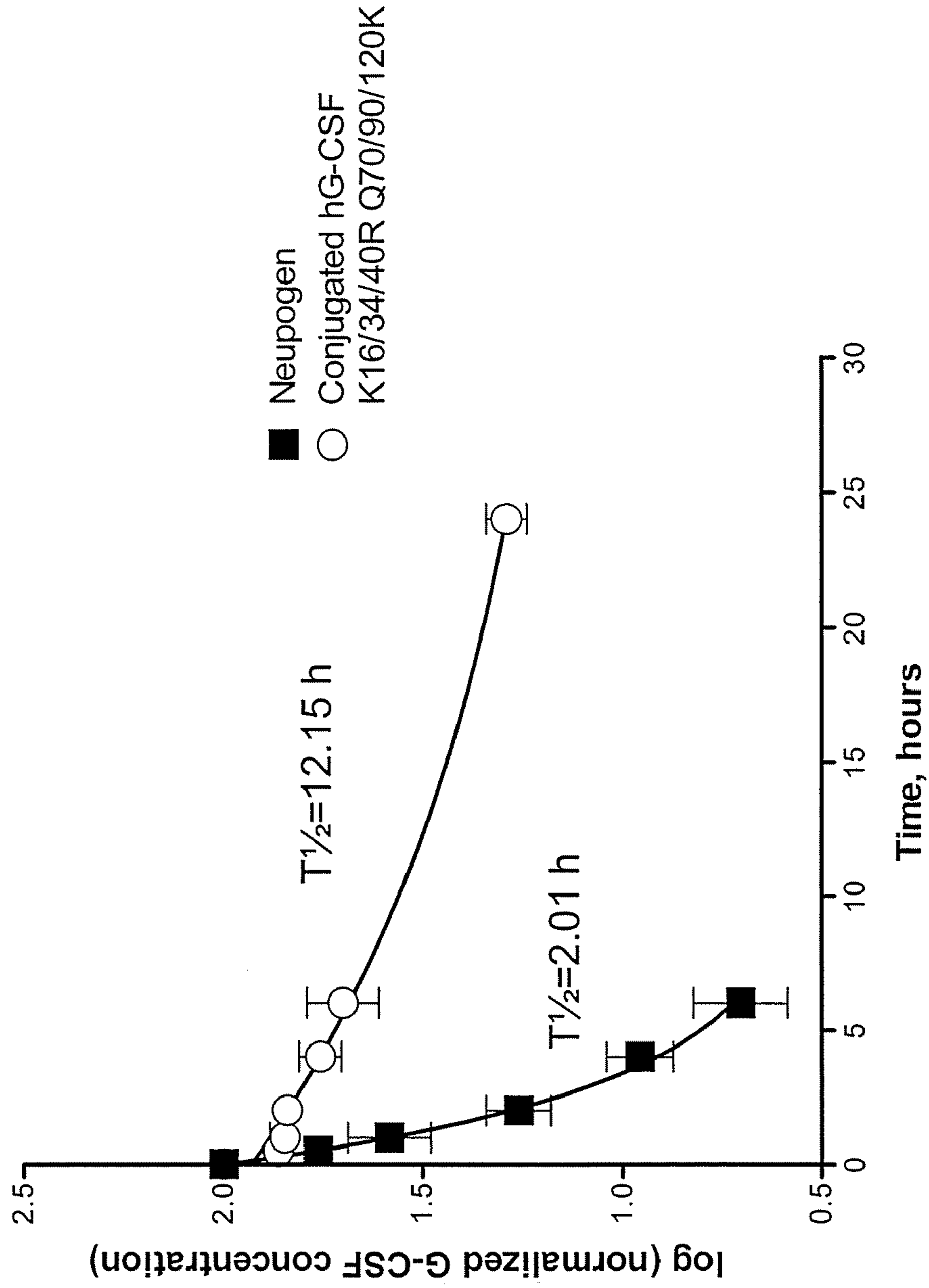
Figure 1 Serum concentrations of Neupogen and conjugated hG-CSF K16R K34R K40R Q70K Q90K Q120K in rats
