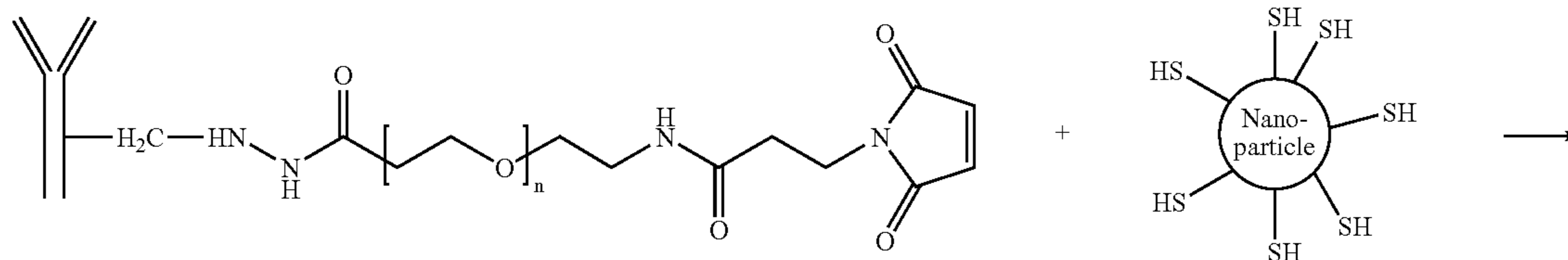
Scheme 23
