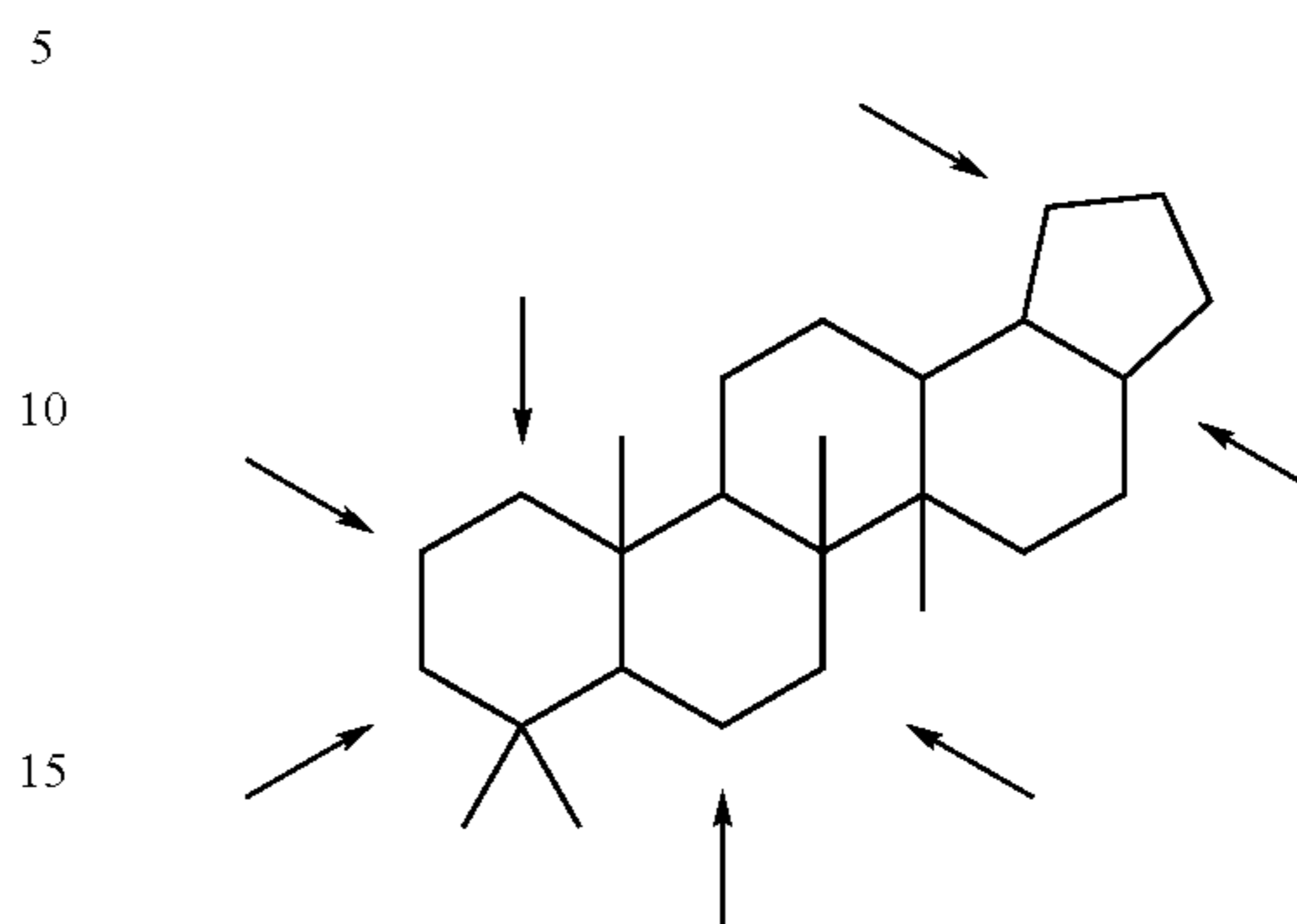
20 Betulinic, Ursolic and Echinocystic Acid Core Structures
