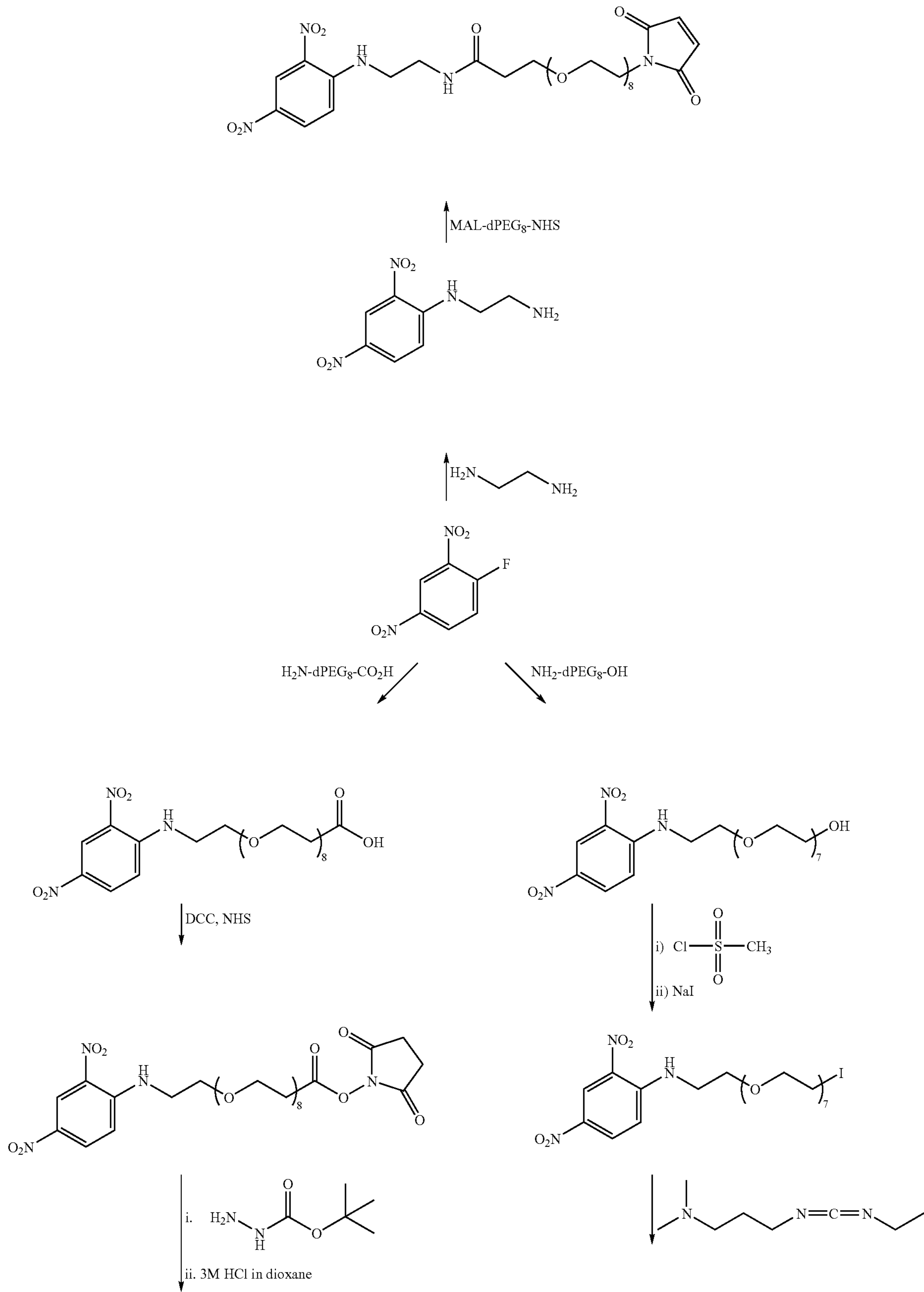
Scheme 2
