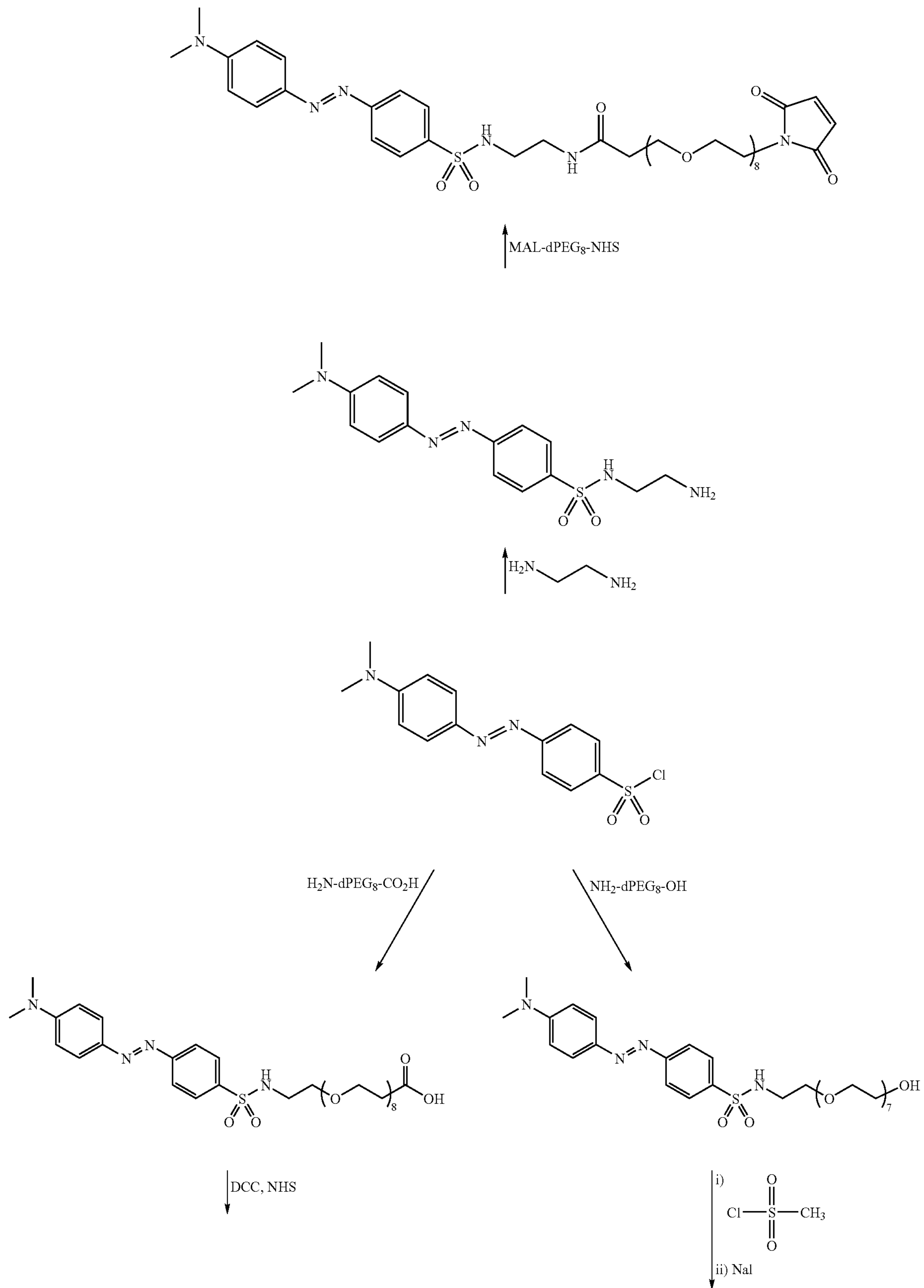
Scheme 15
