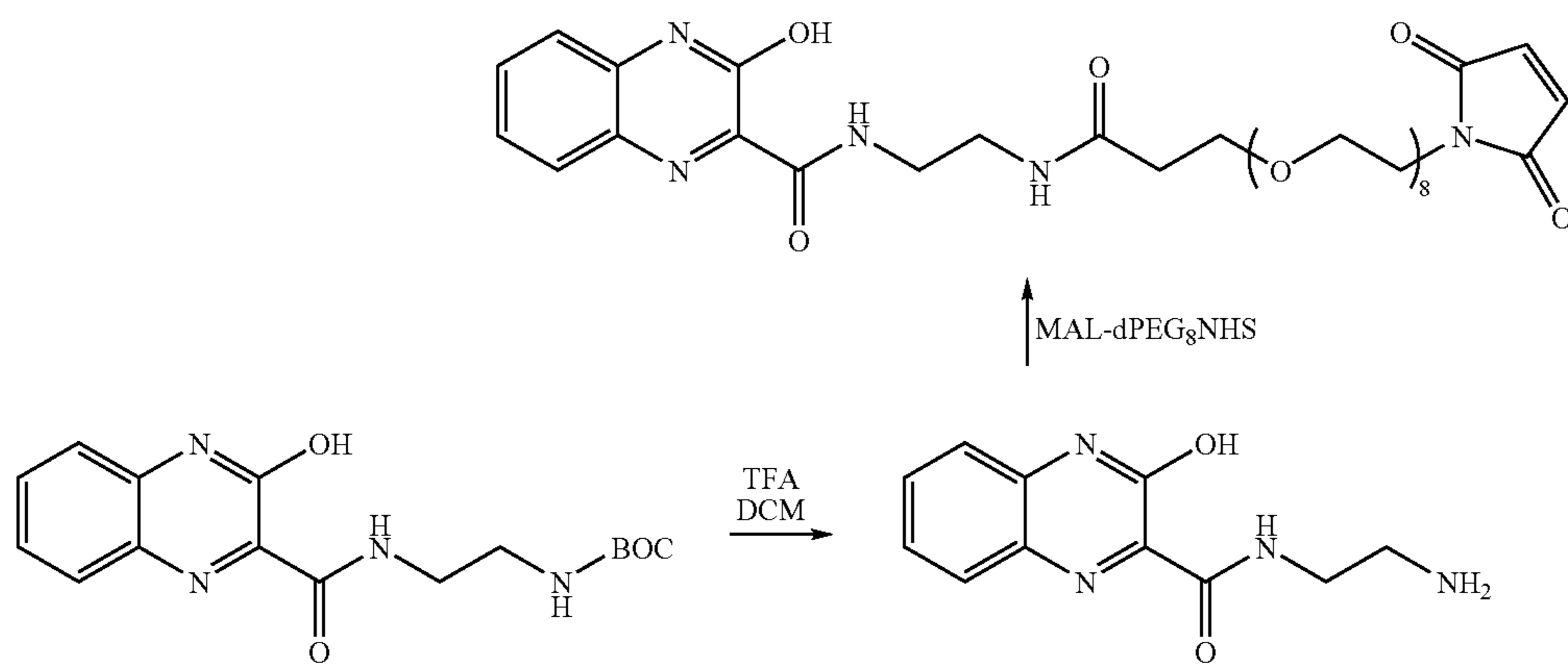
Scheme 14
