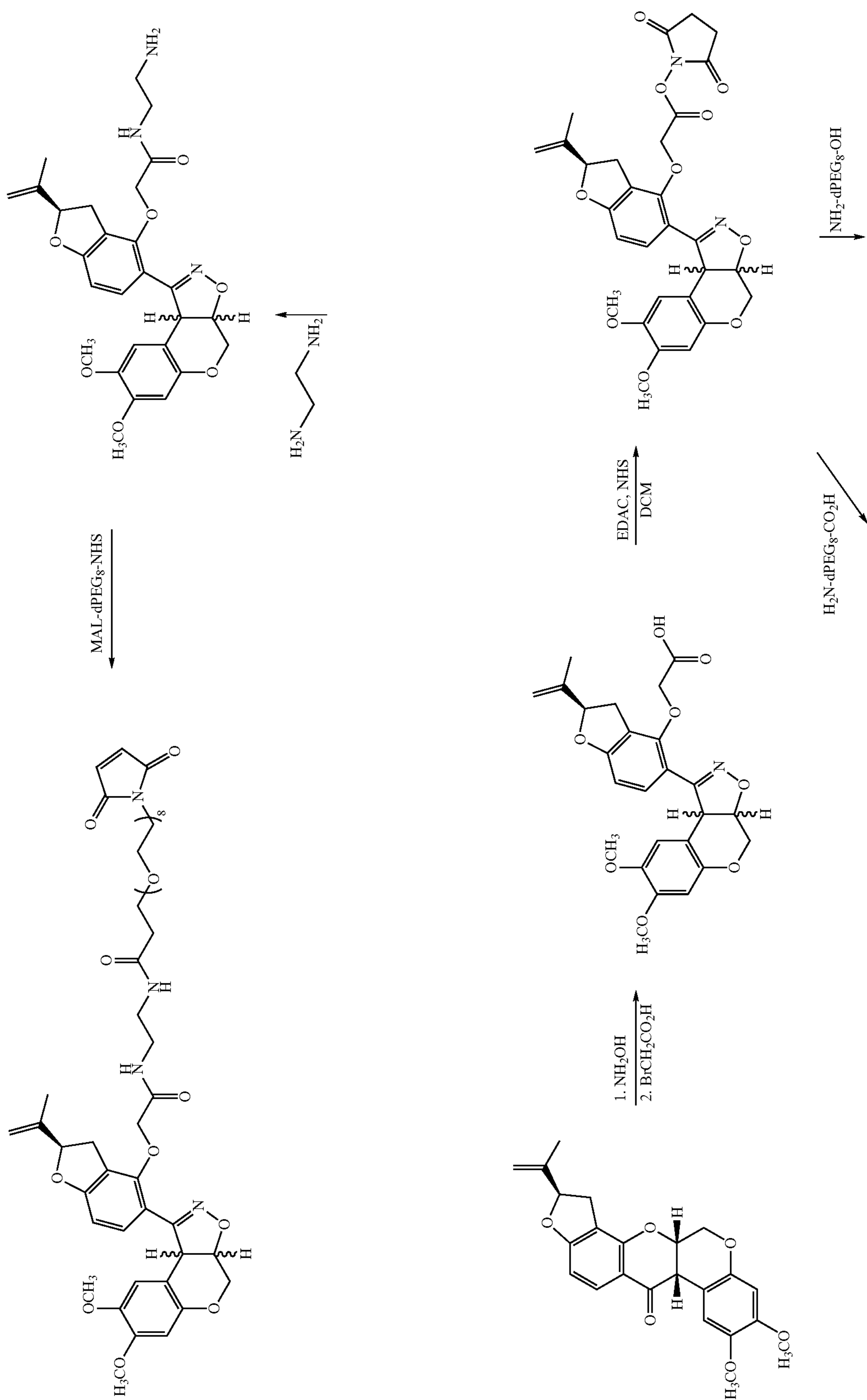
Scheme 9
