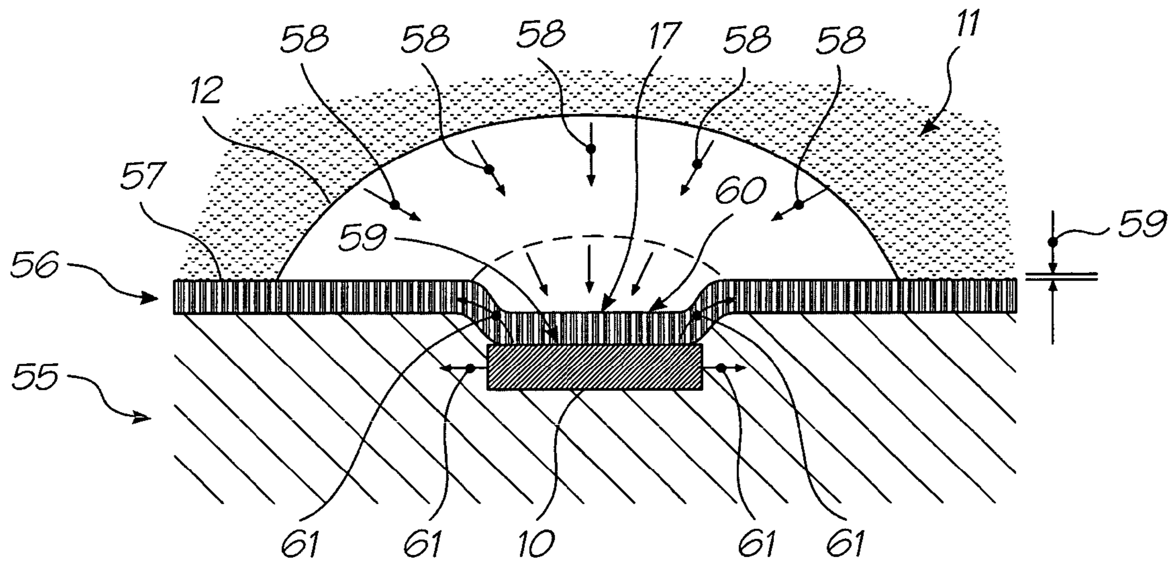
FIG. 47 (PRIOR ART)
