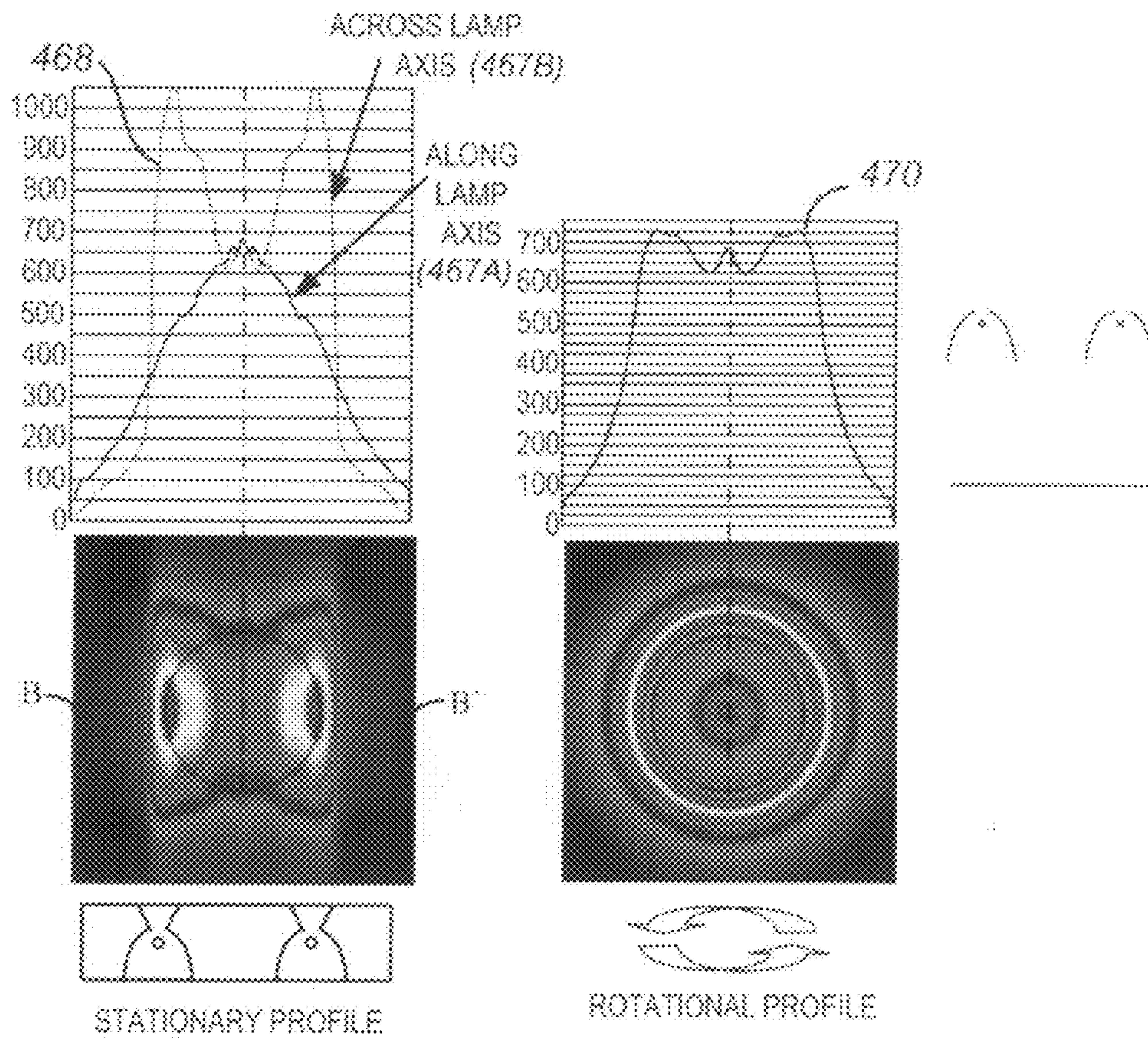
Primary Reflector (asymmetric) - dual lamp
