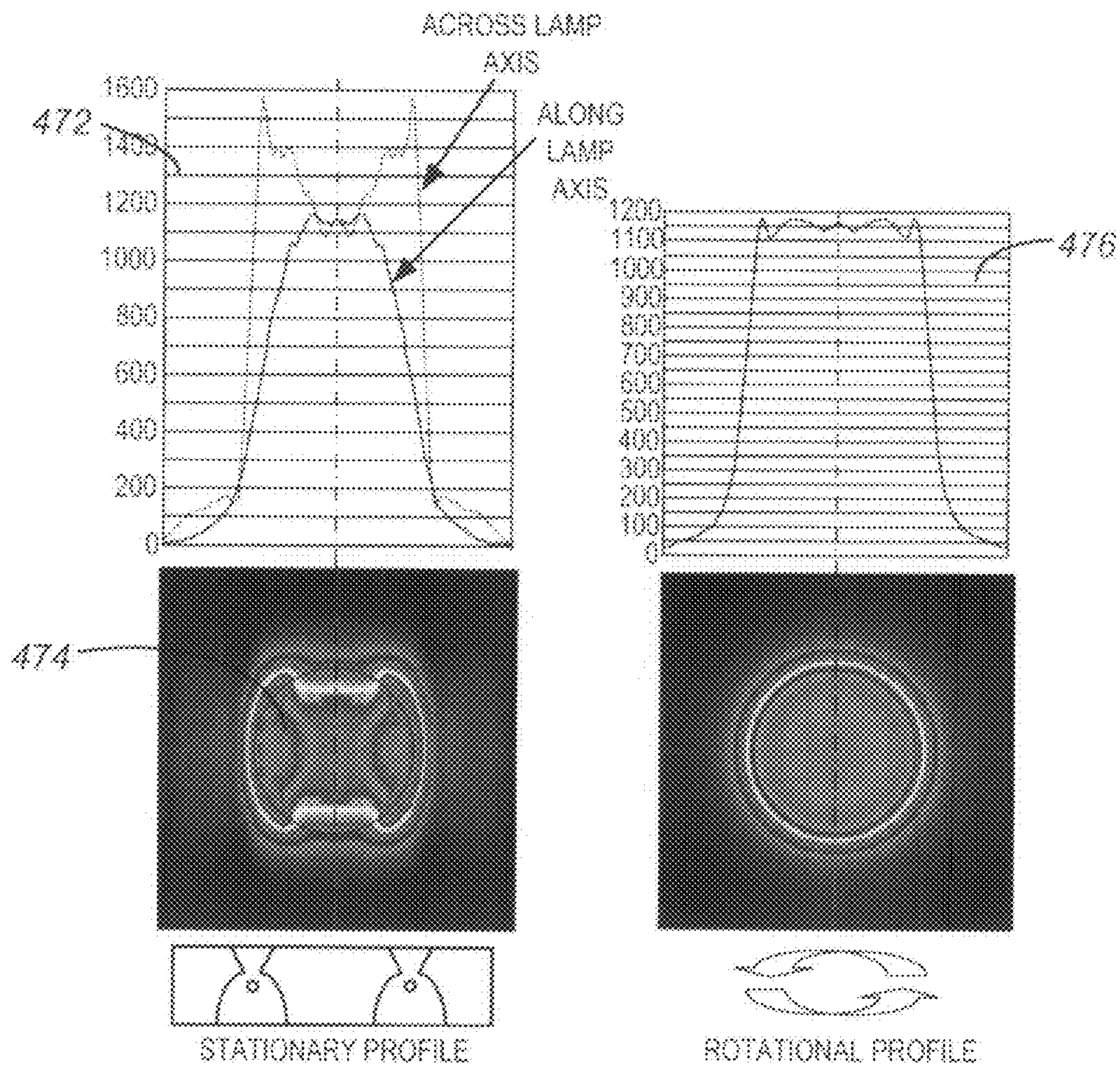
Primary (asymmetric) + Secondary Reflector - dual lamp
