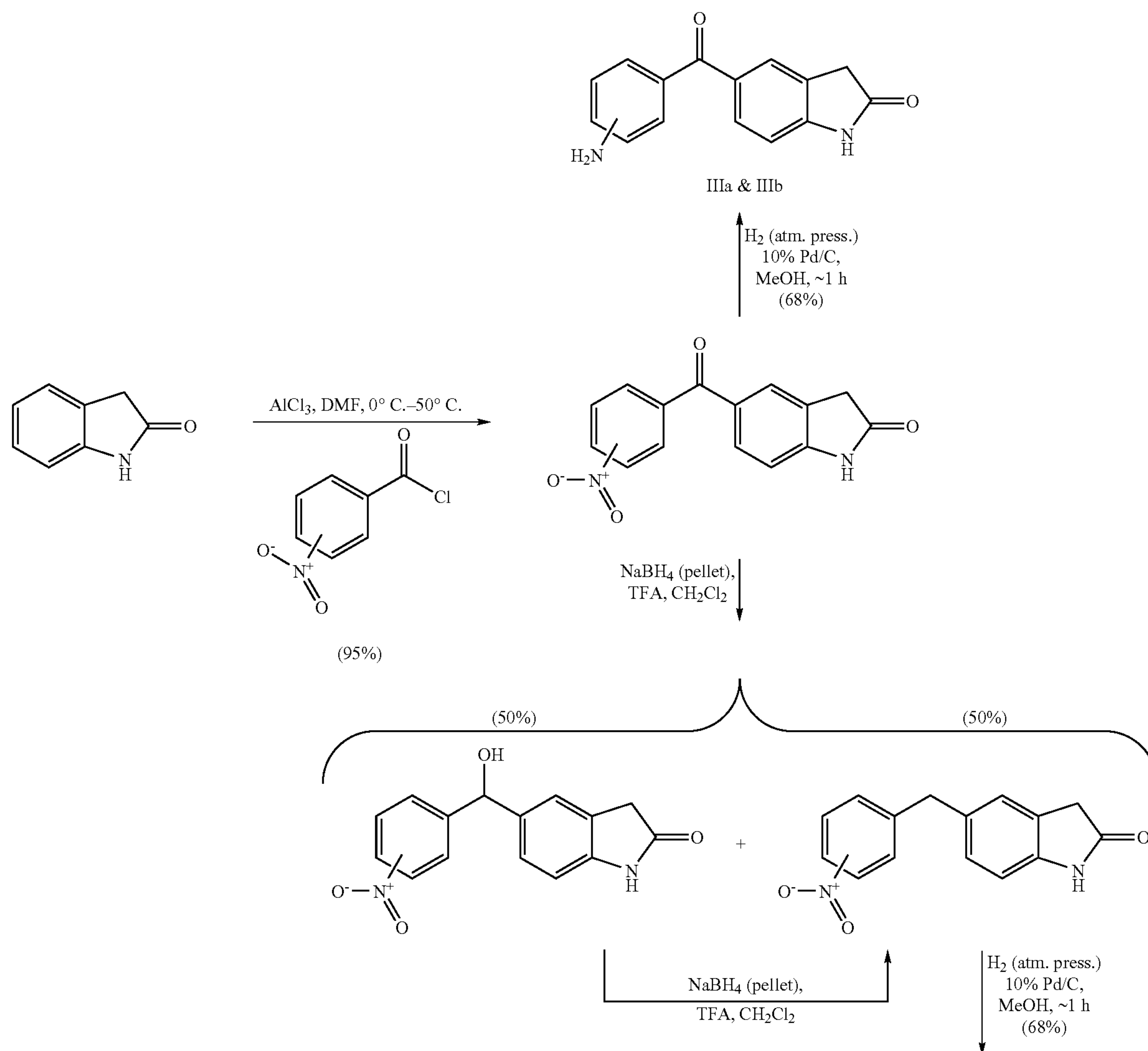
Scheme I: Preparation of IIIa & IIIb (5-(3, and 4-Amino-benzoyl)-1,3-dihydro-indol-2-one) and IVa & IVb (5-(3, and 4-Amino-benzoyl)-1,3-dihydro-indol-2-one).
