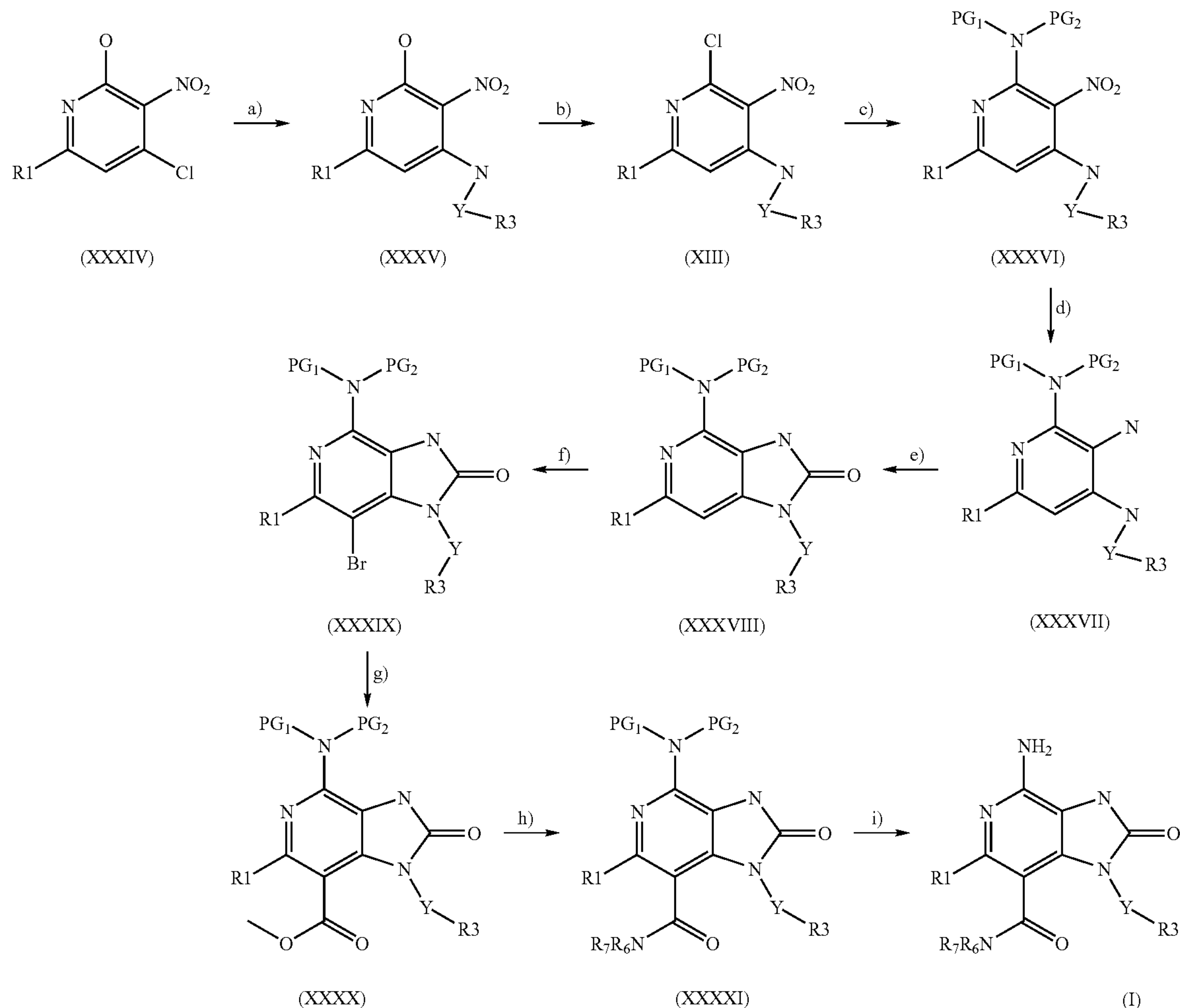
Scheme 3
