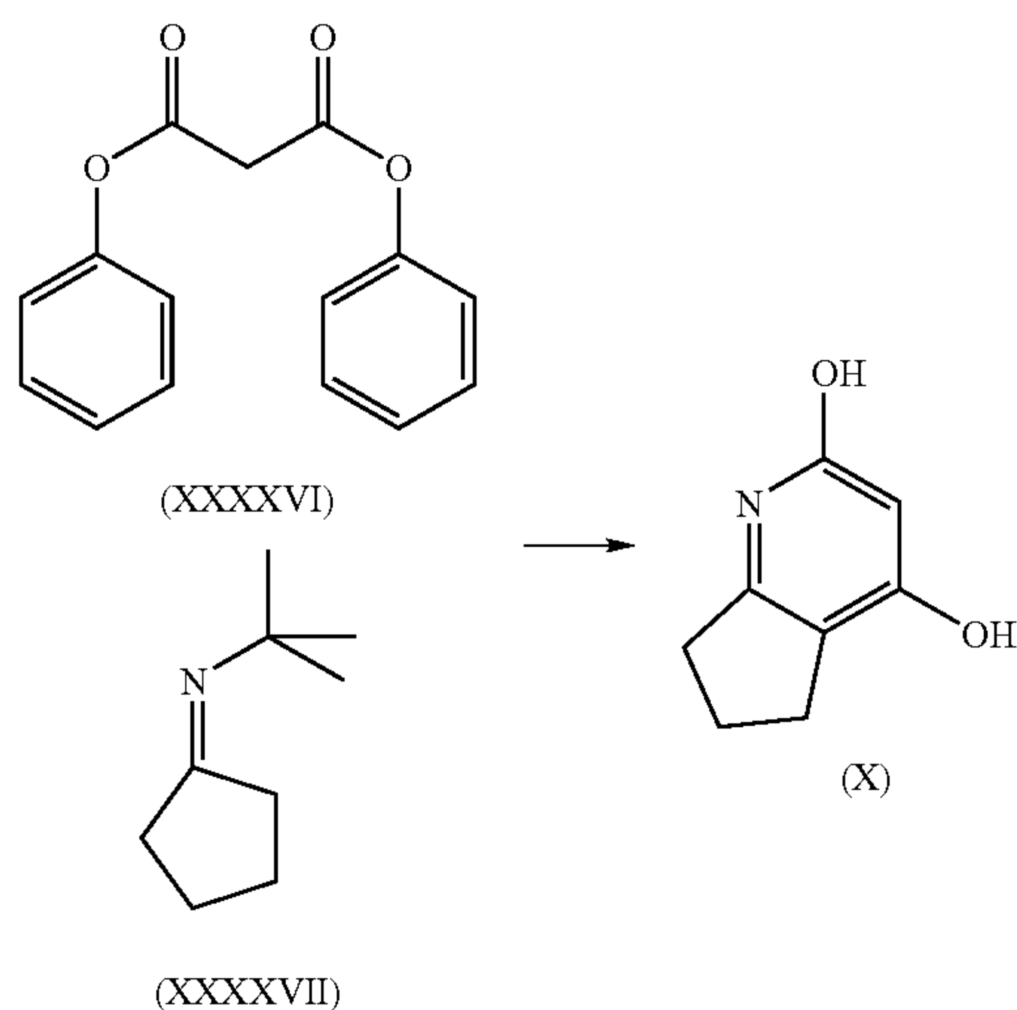
Scheme 5
