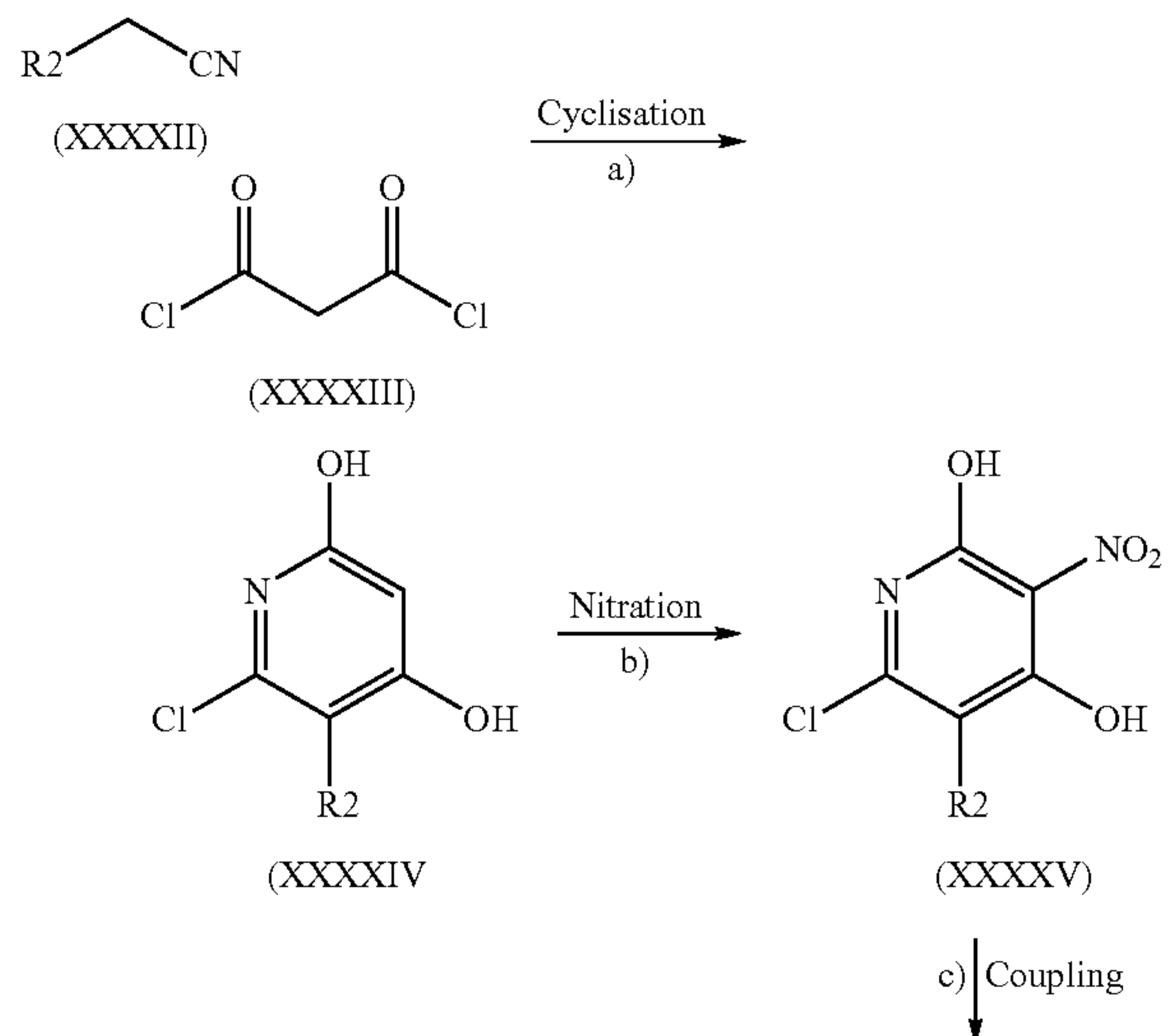
Scheme 4
