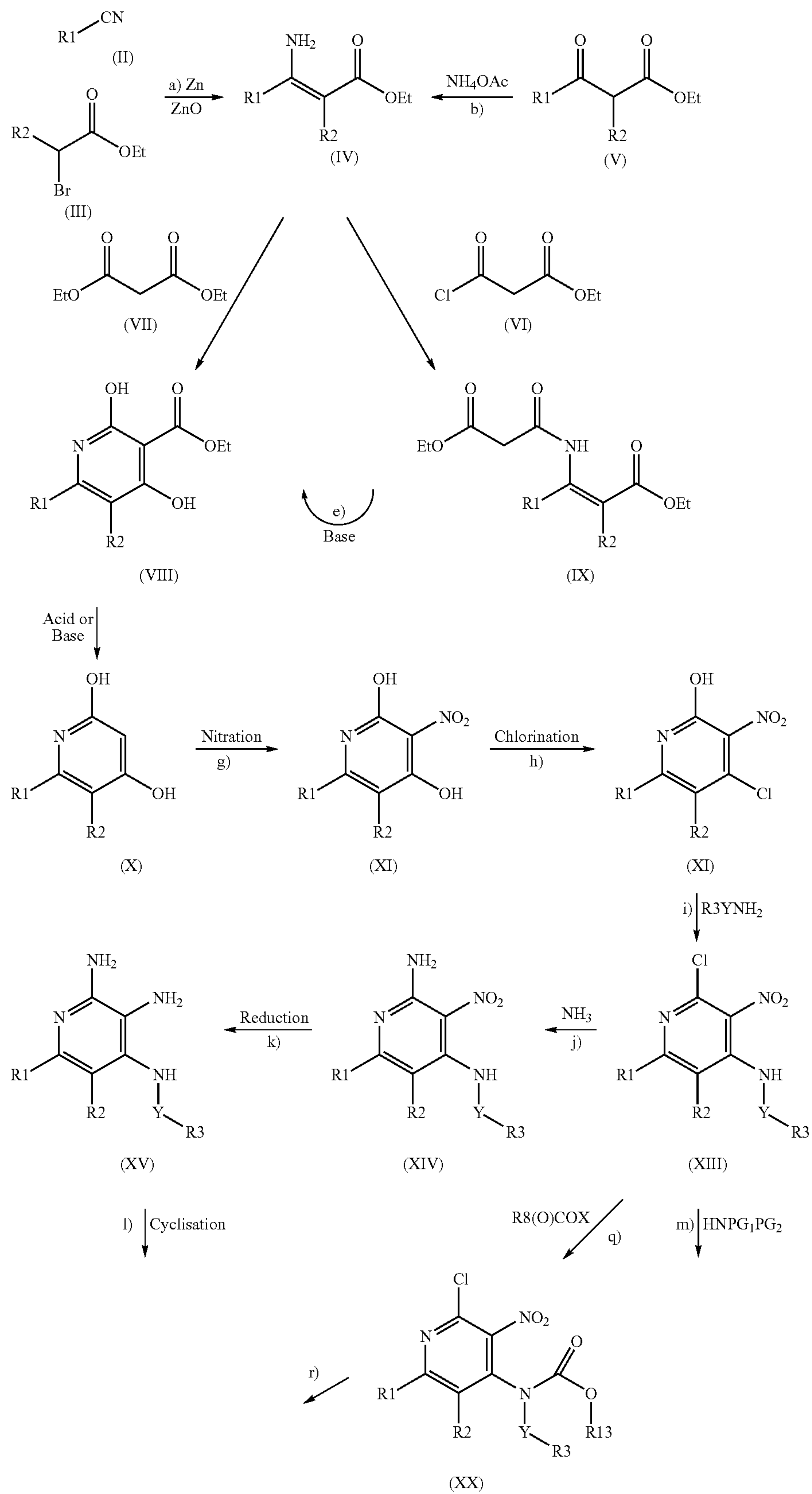
Scheme 1
