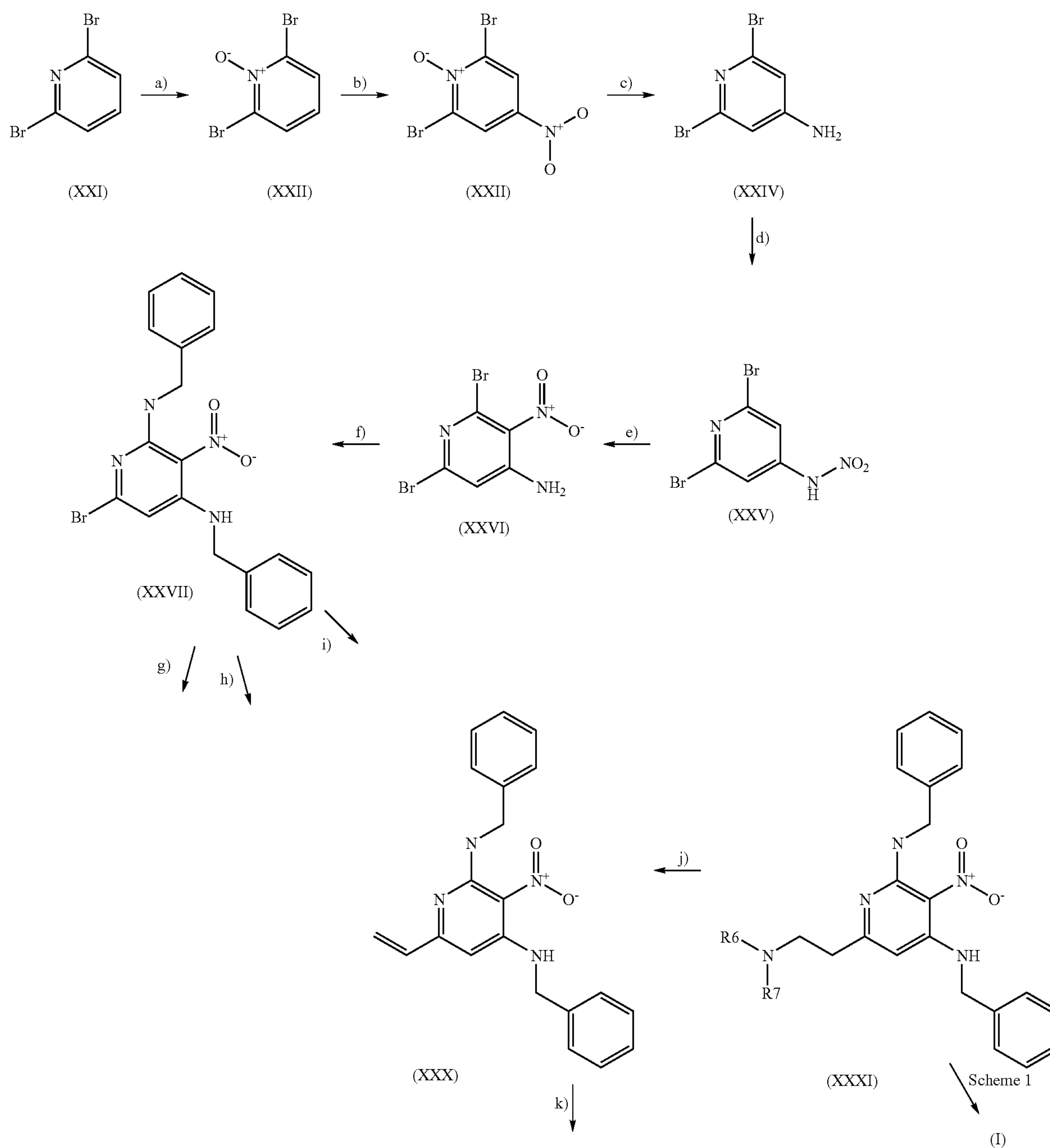
Scheme 2
