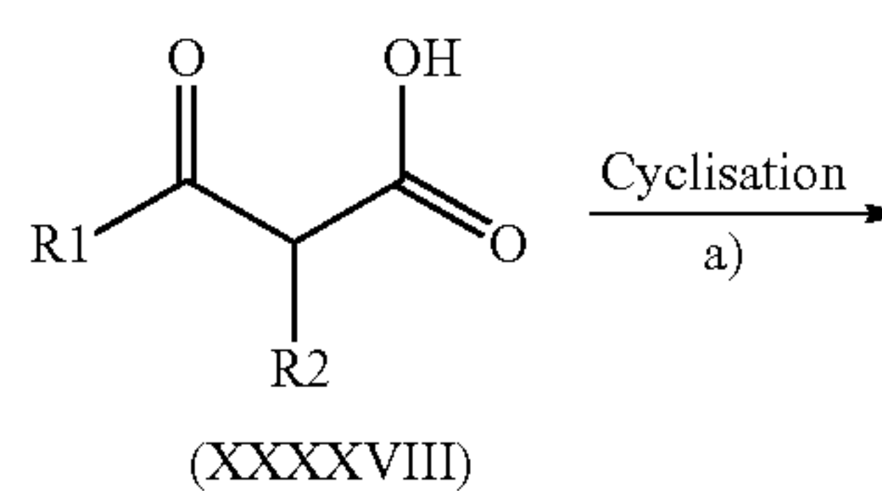
Scheme 6
