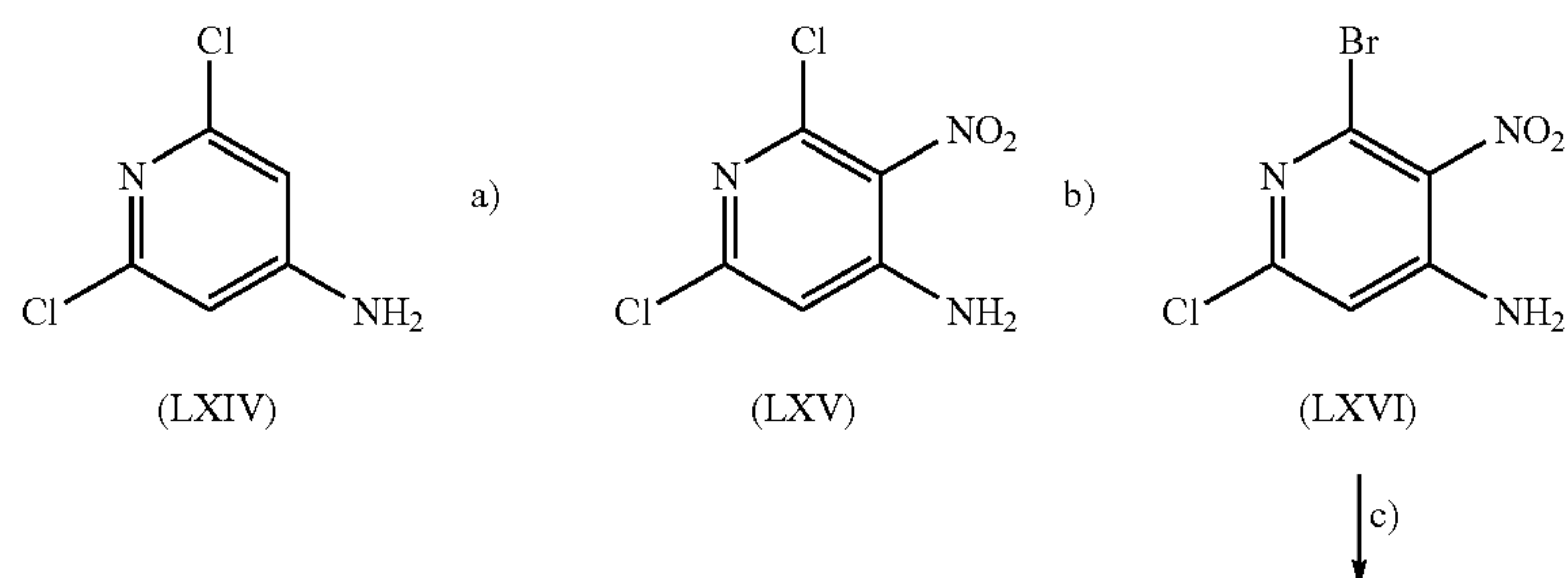
Scheme 10
