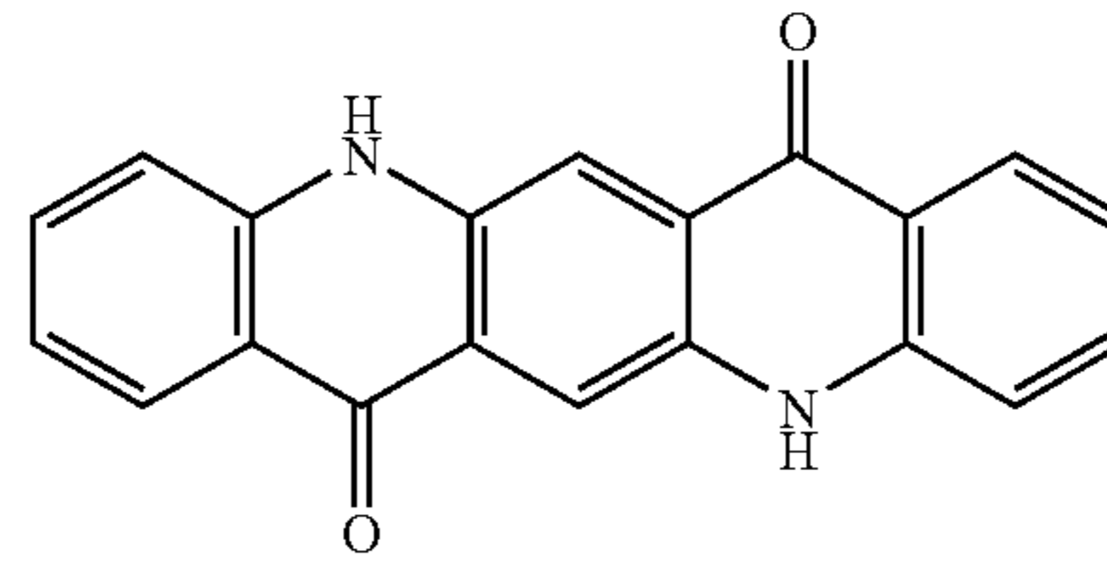
Quinacridone
