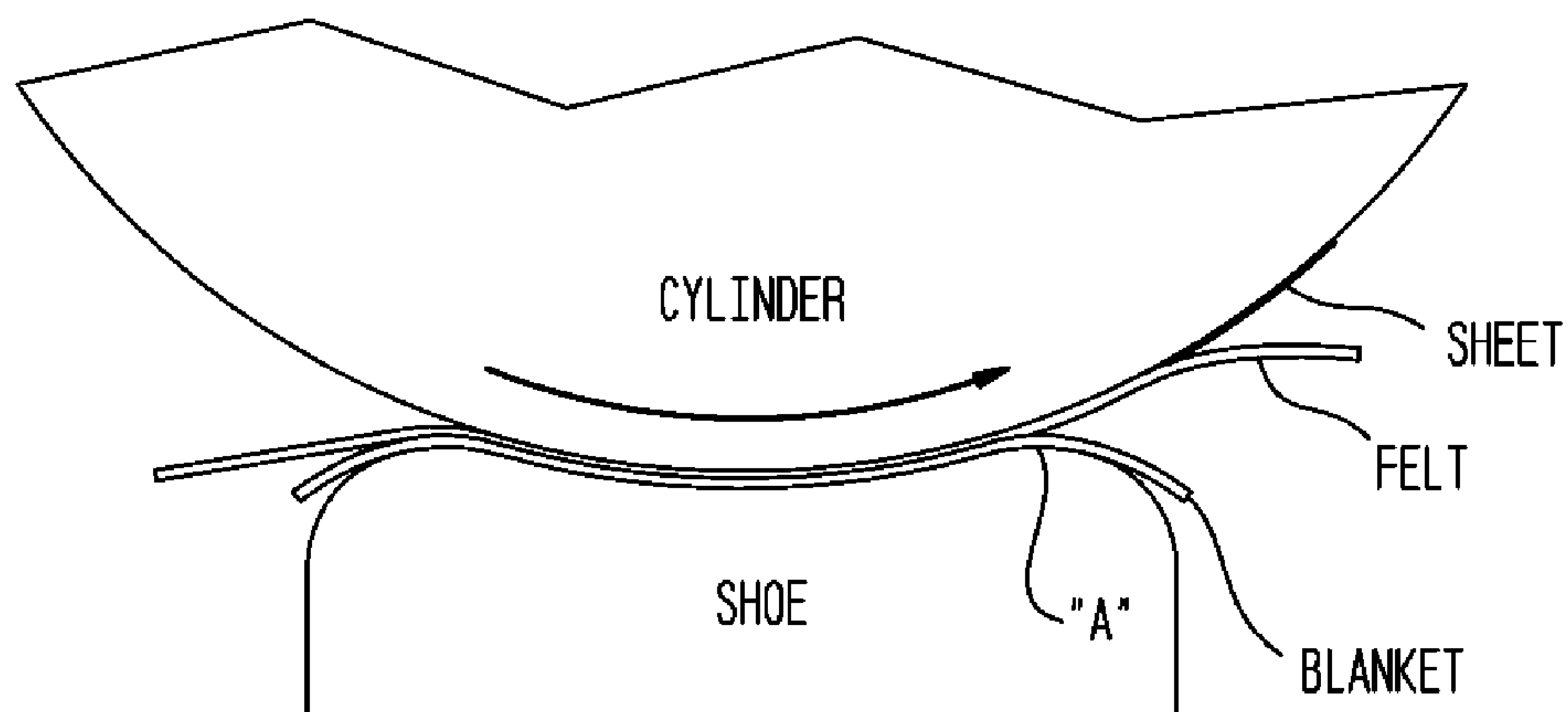
SHOE PRESS WITH LARGE DIAMETER TRANSFER CYLINDER AND WITH FELT PARTIALLY WRAPPING CYLINDER
