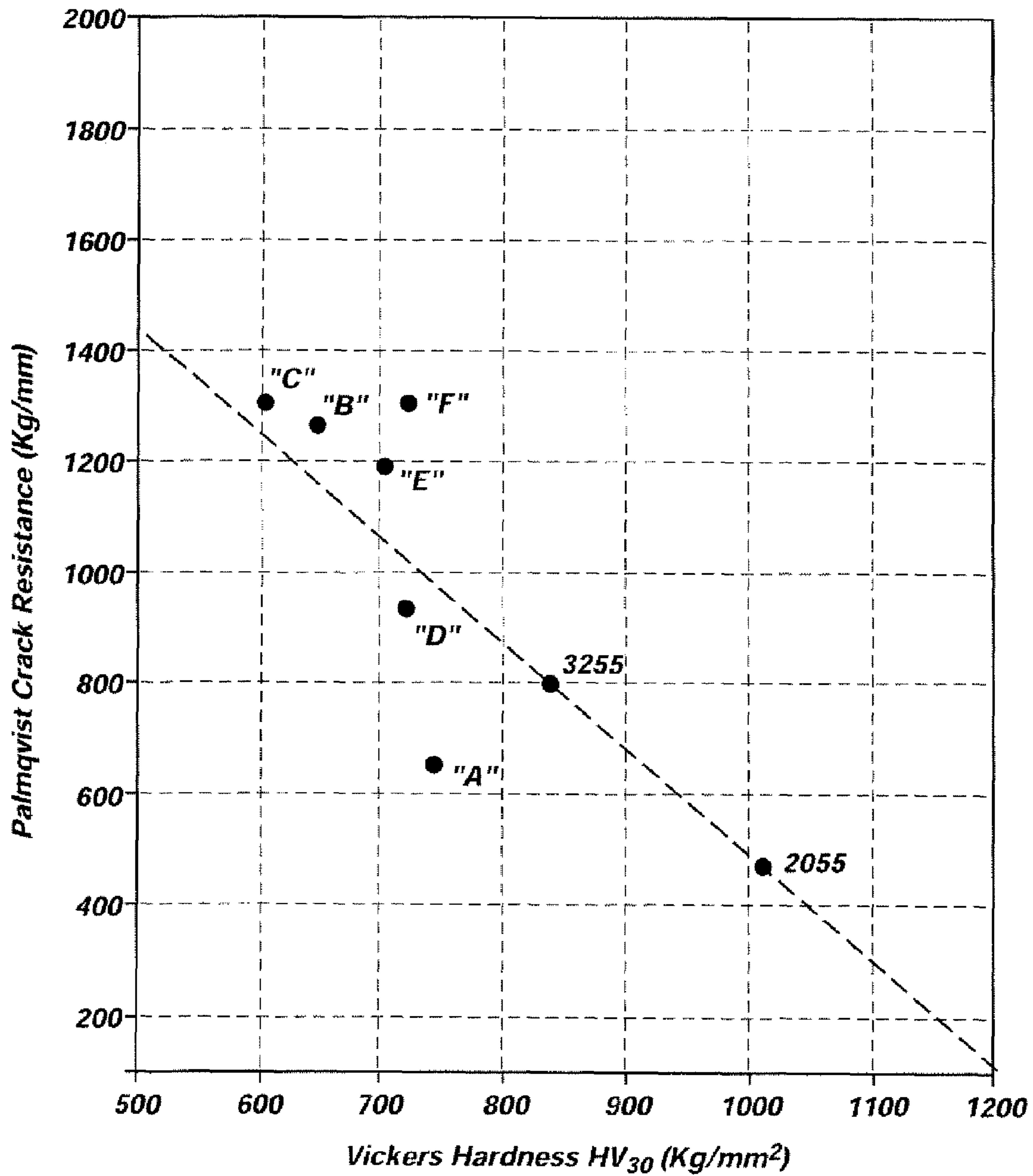
Hardness vs Toughness for example alloy binder carbides and conventional cemented carbides
