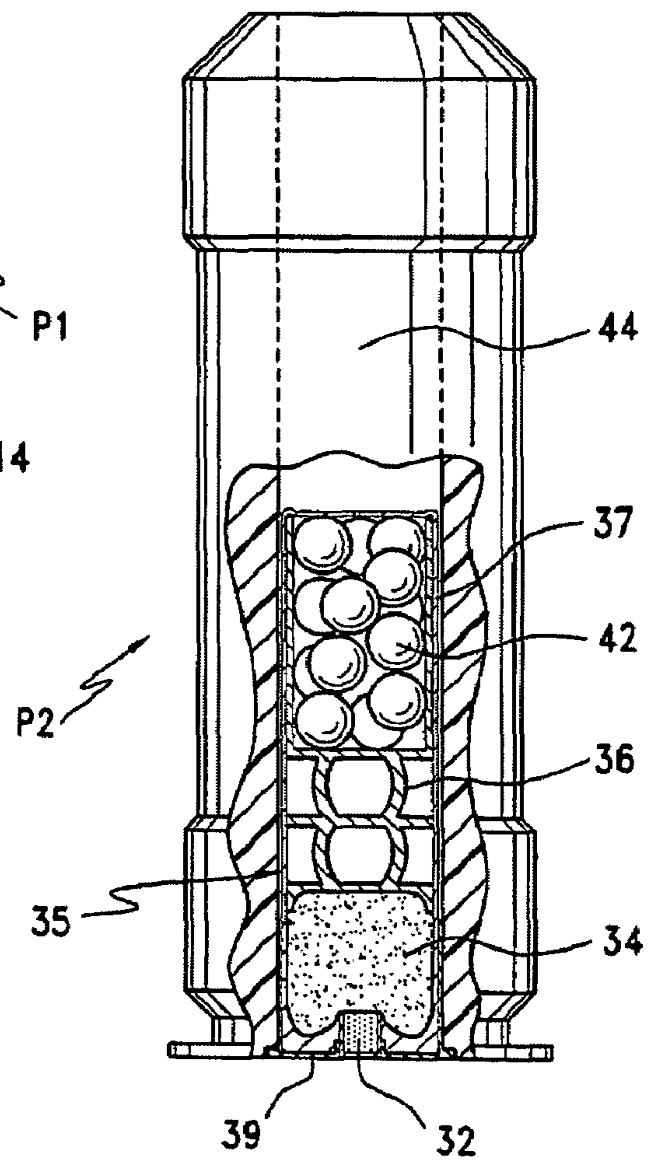
FIG. 2 (PRIOR ART)
