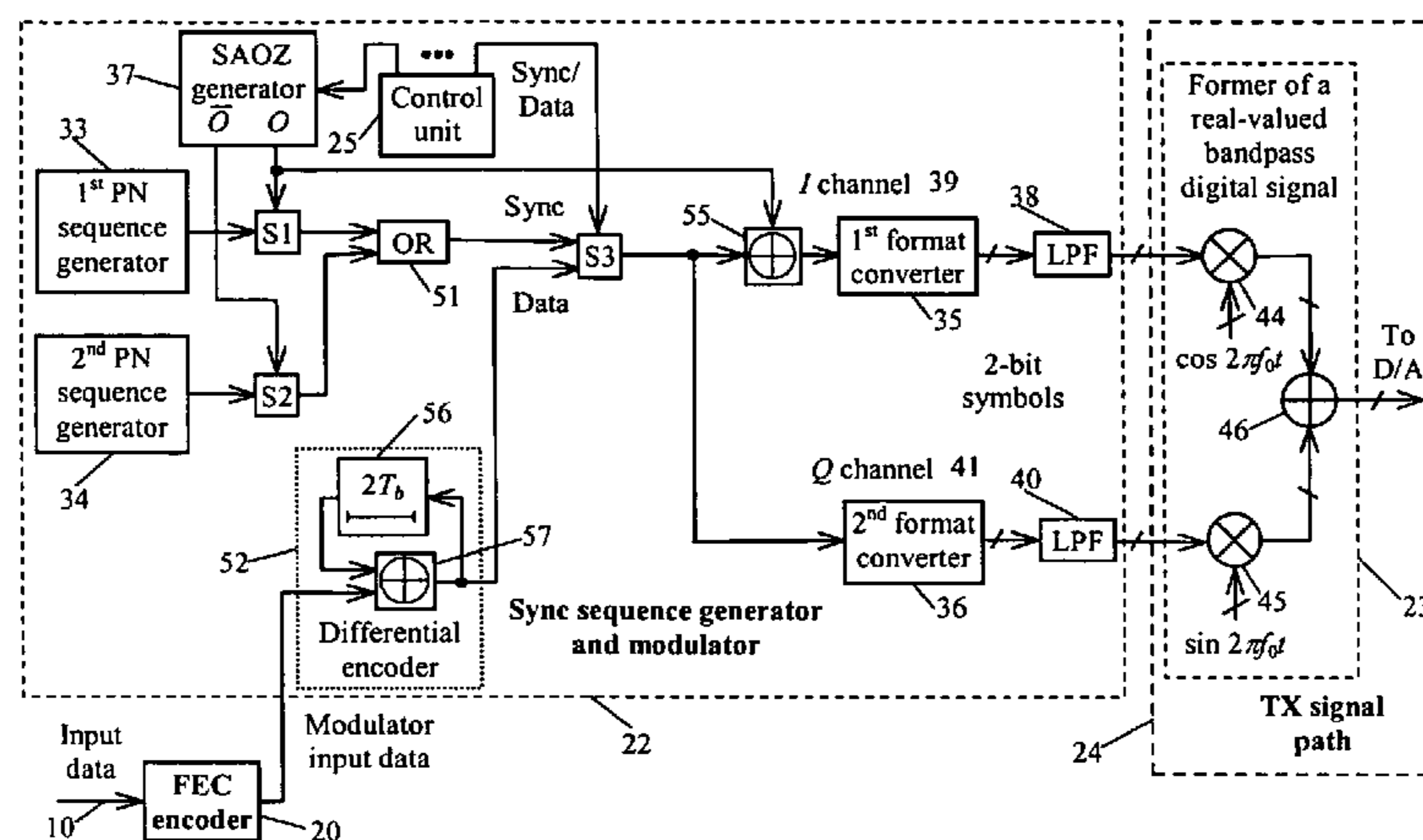
Block diagram of the sync sequence generator and modulator with joint differential encoding of the same parity modulator input data bits for the I and Q channels and separate format conversion in these channels (the 2 nd embodiment).
