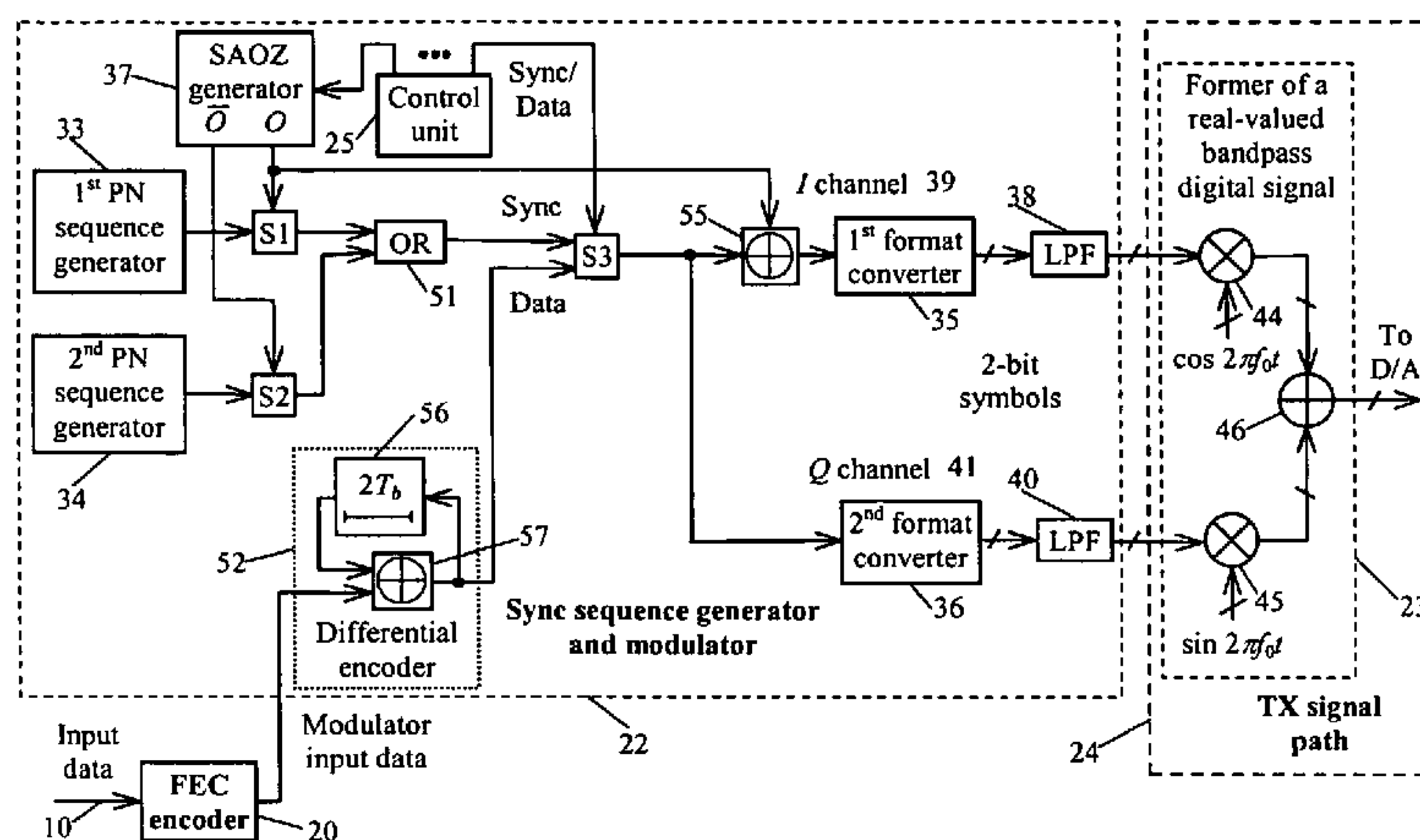
Block diagram of the sync sequence generator and modulator with joint differential encoding of the same parity modulator input data bits for the I and Q channels and separate format conversion in these channels (the 2 nd embodiment).
