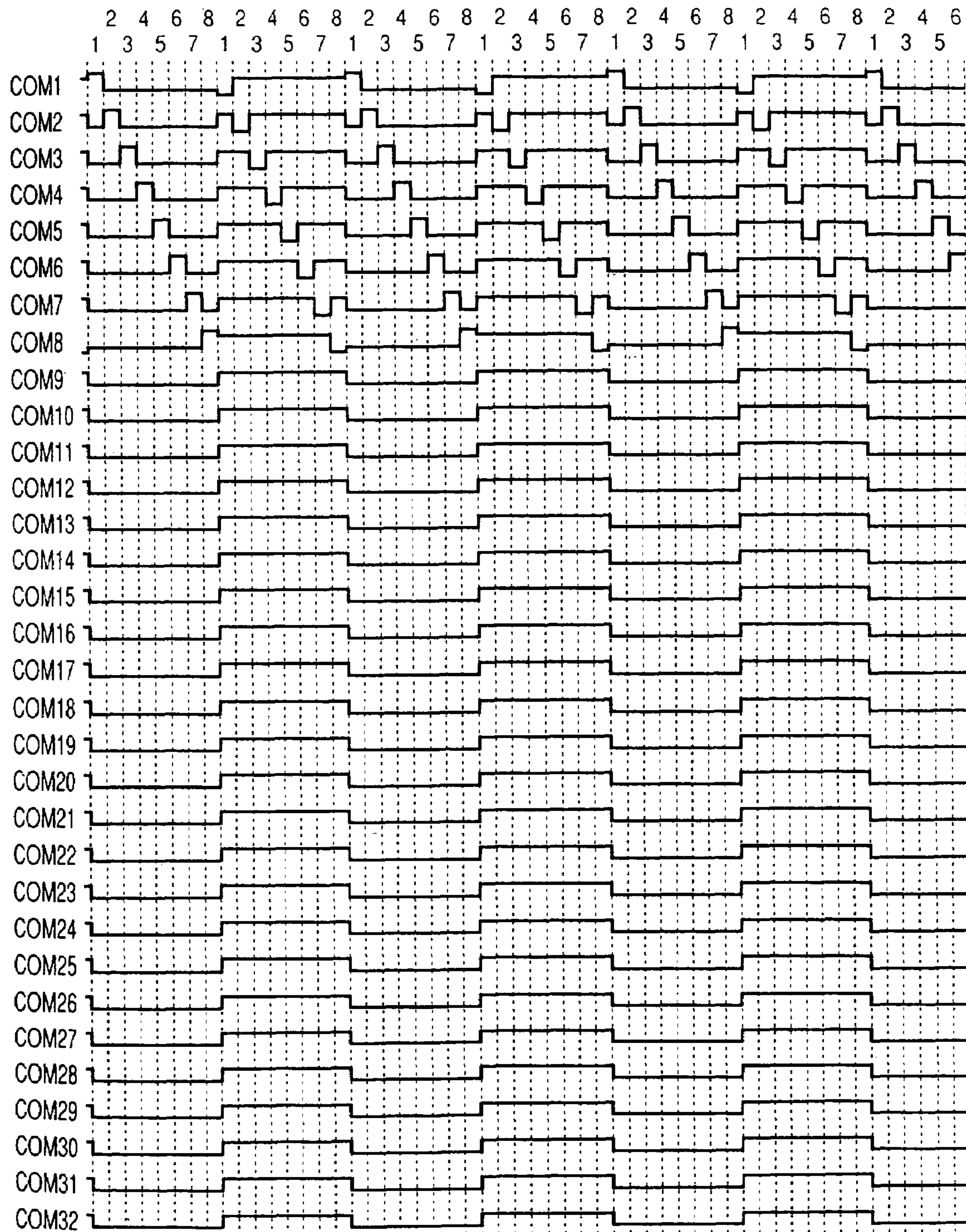
1/8 DUTY DRIVE (COM1~COM8)
