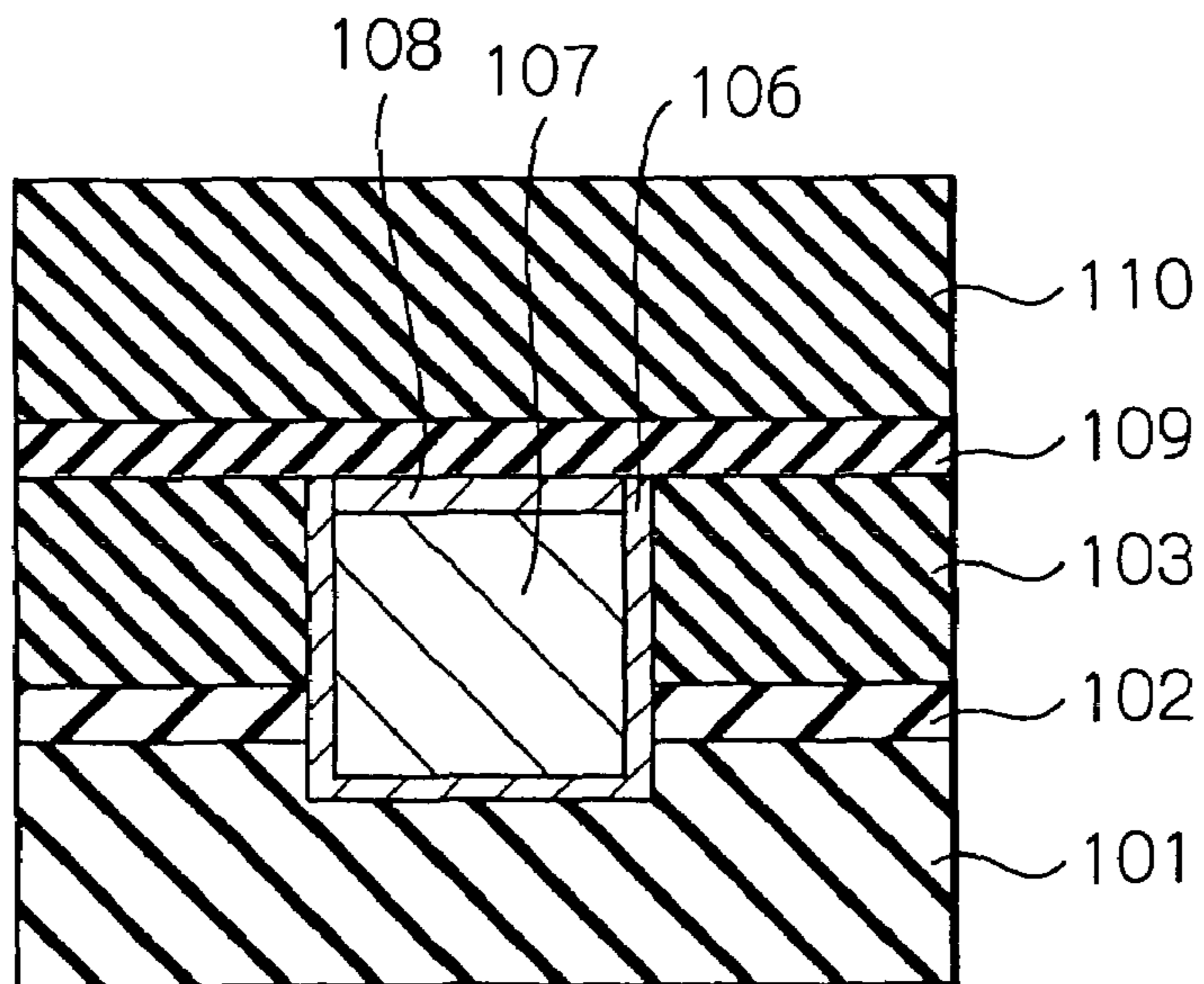
Fig. 1H PRIOR ART
