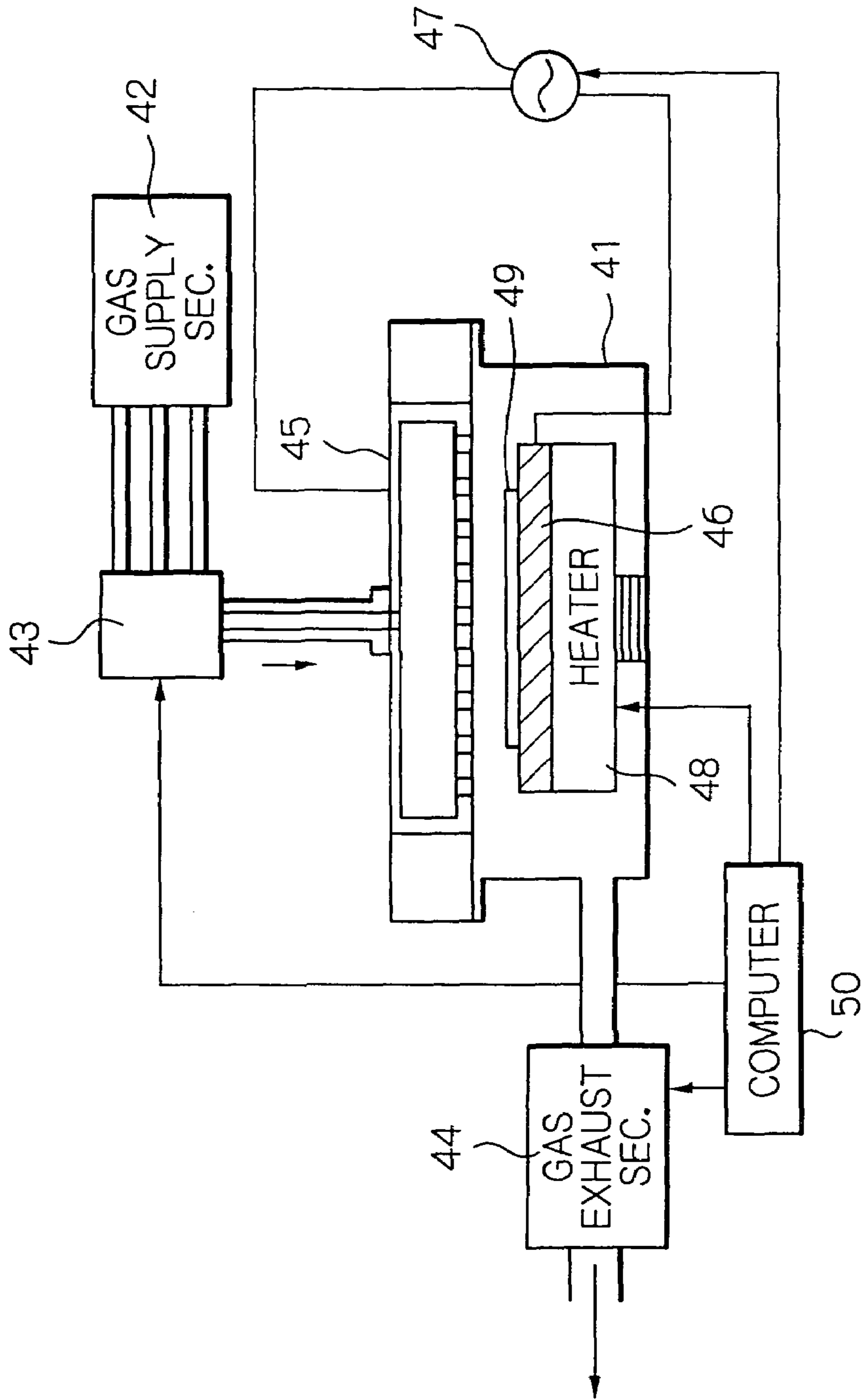
Fig. 4 PRIOR ART
