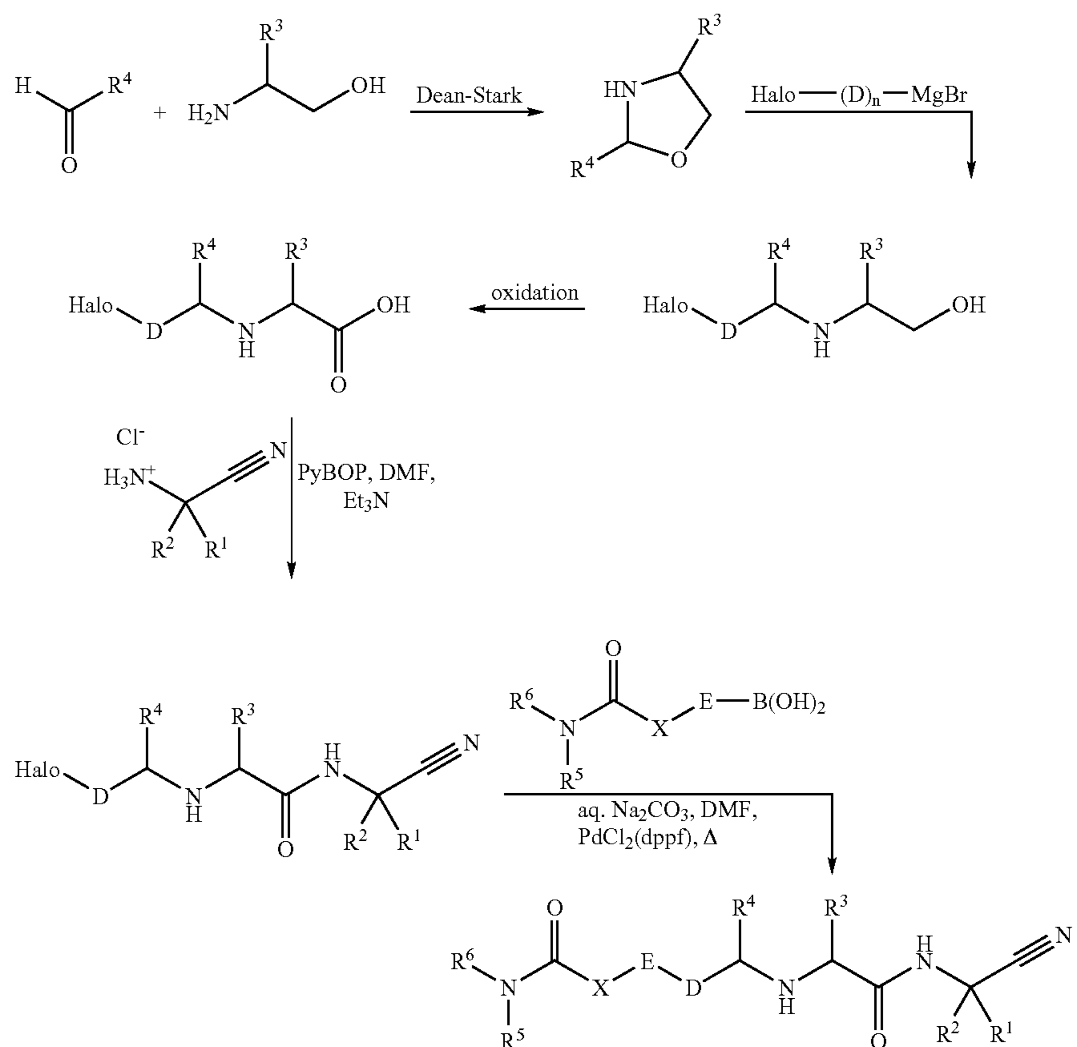
SCHEME 2
