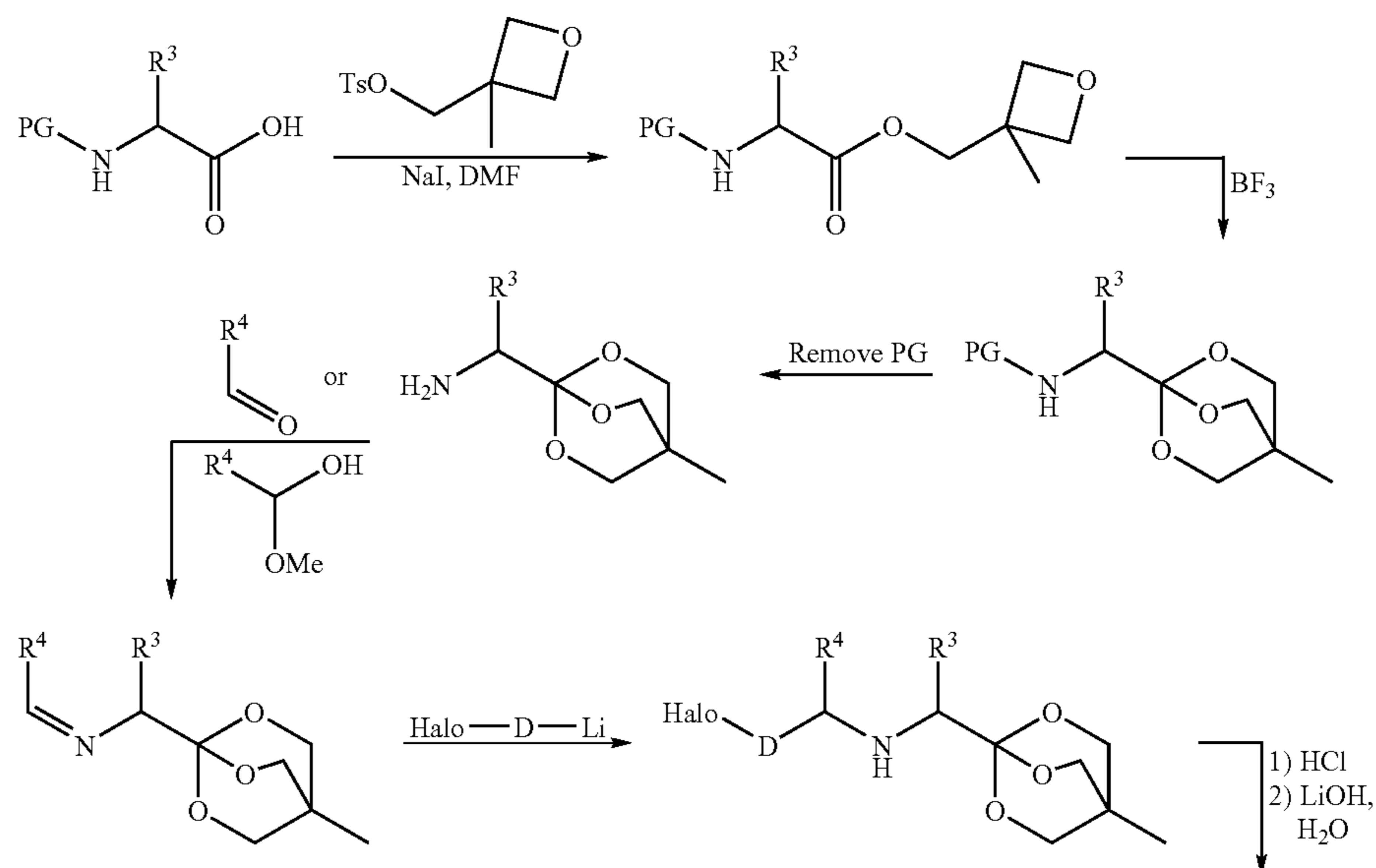
SCHEME 7
