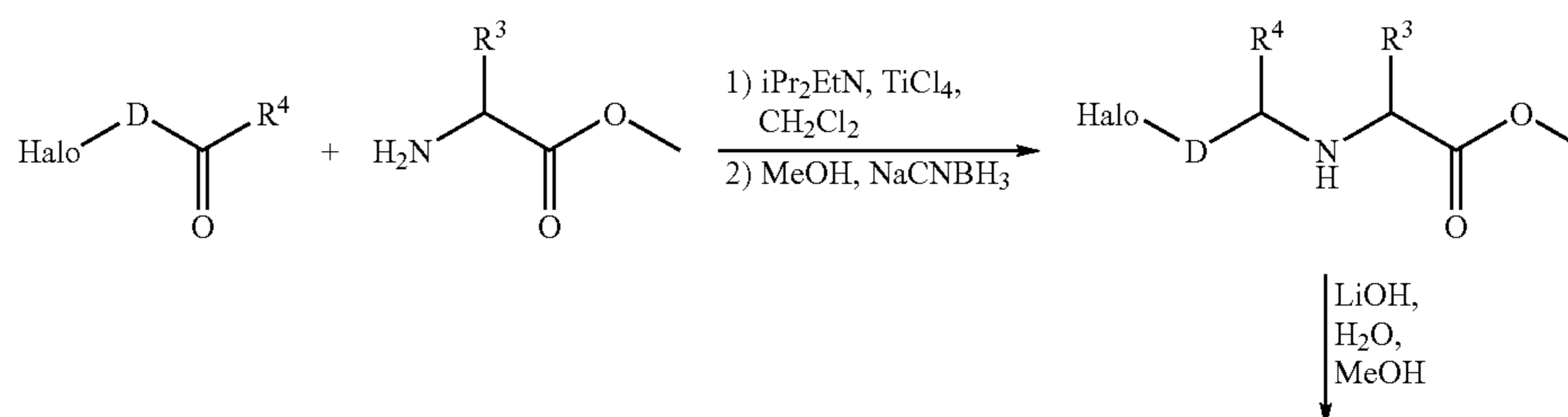
SCHEME 1
