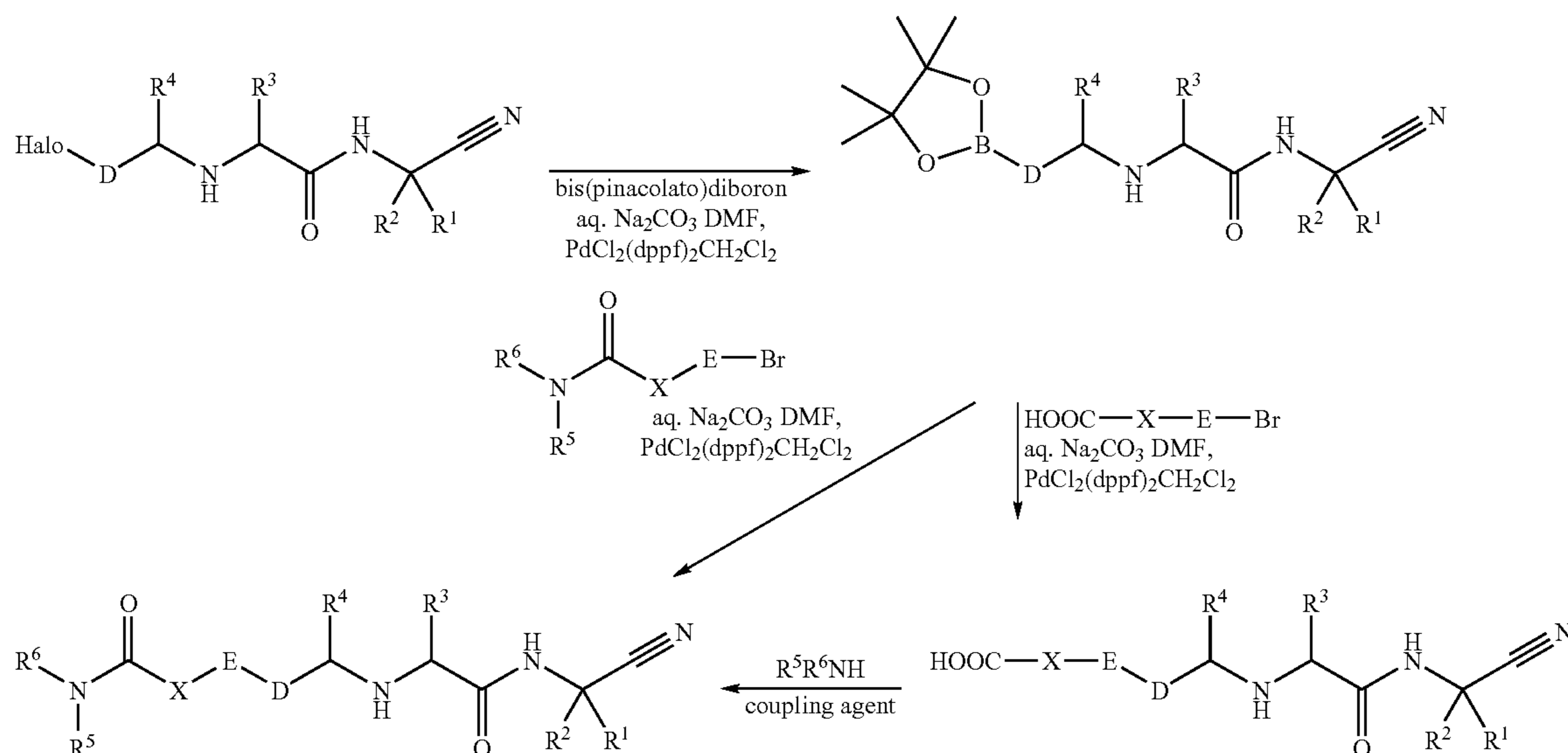
SCHEME 8
