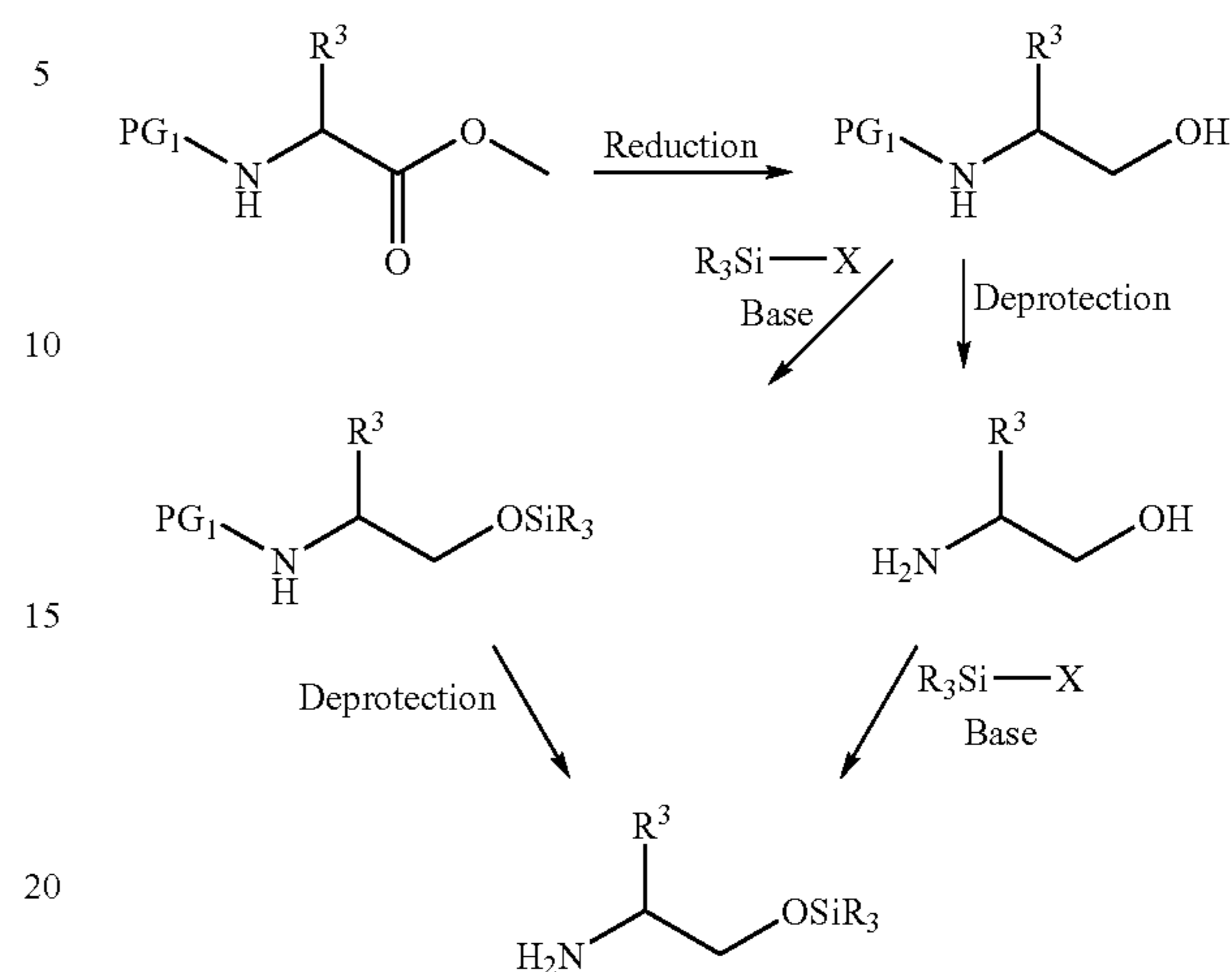
SCHEME 6
