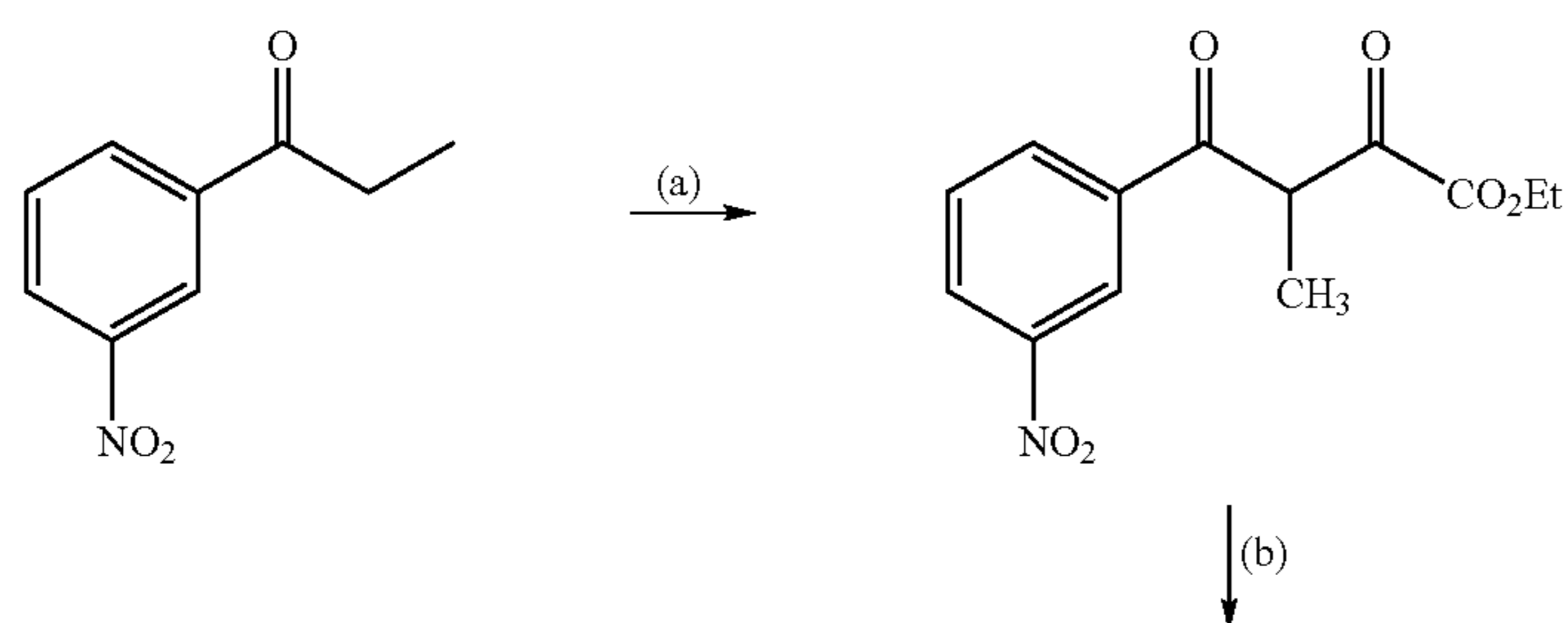
Scheme 5
