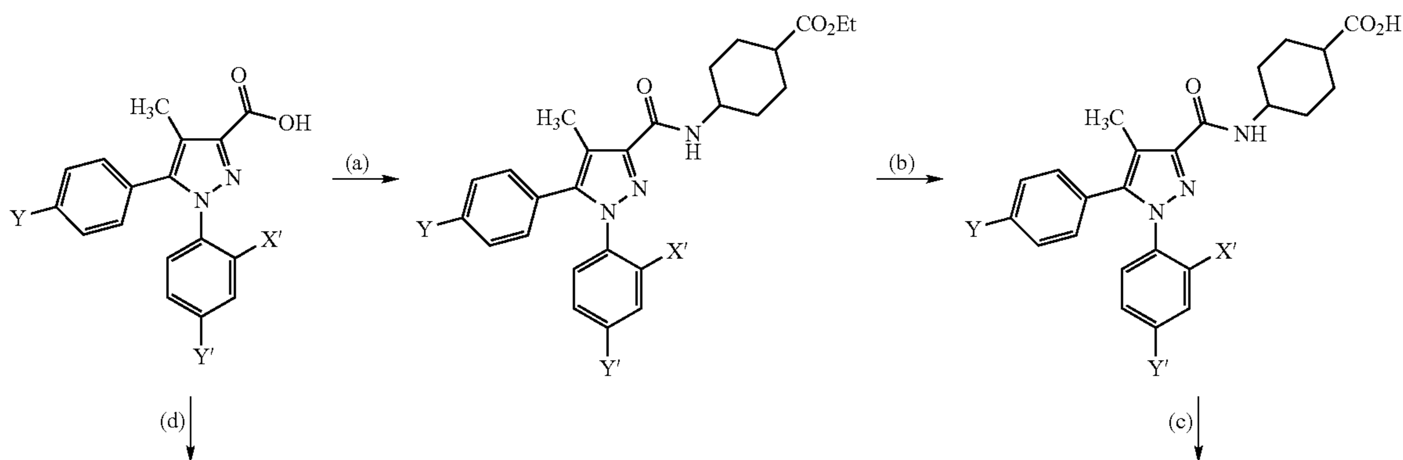
Scheme 2
