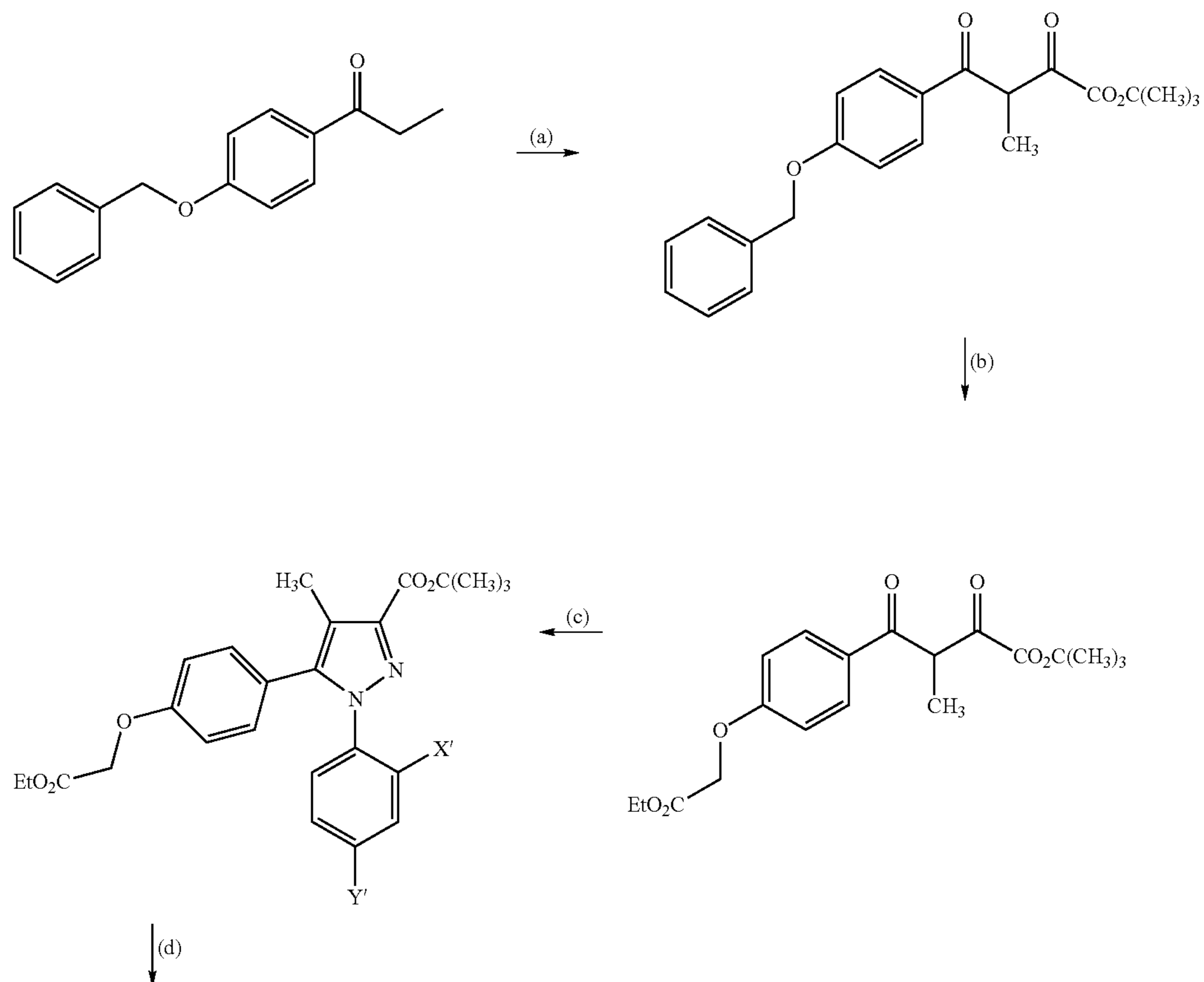
Scheme 4
