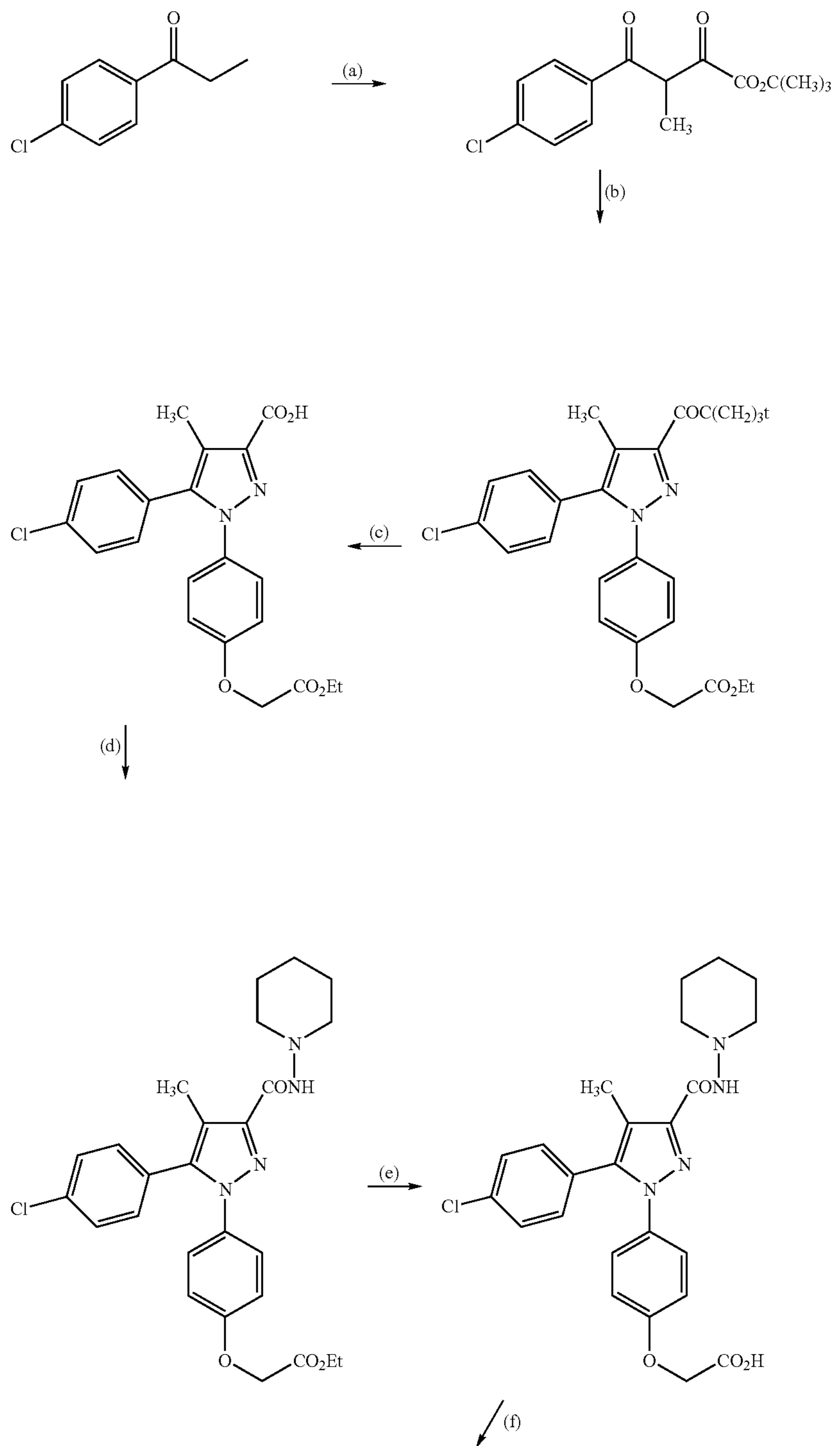
Scheme 9
