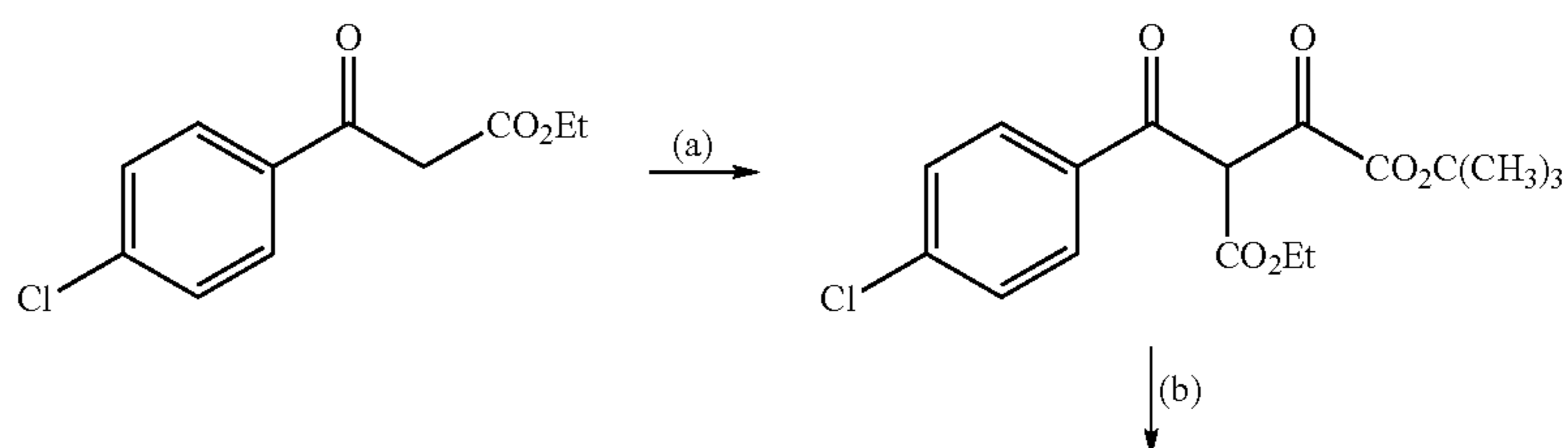
Scheme 11
