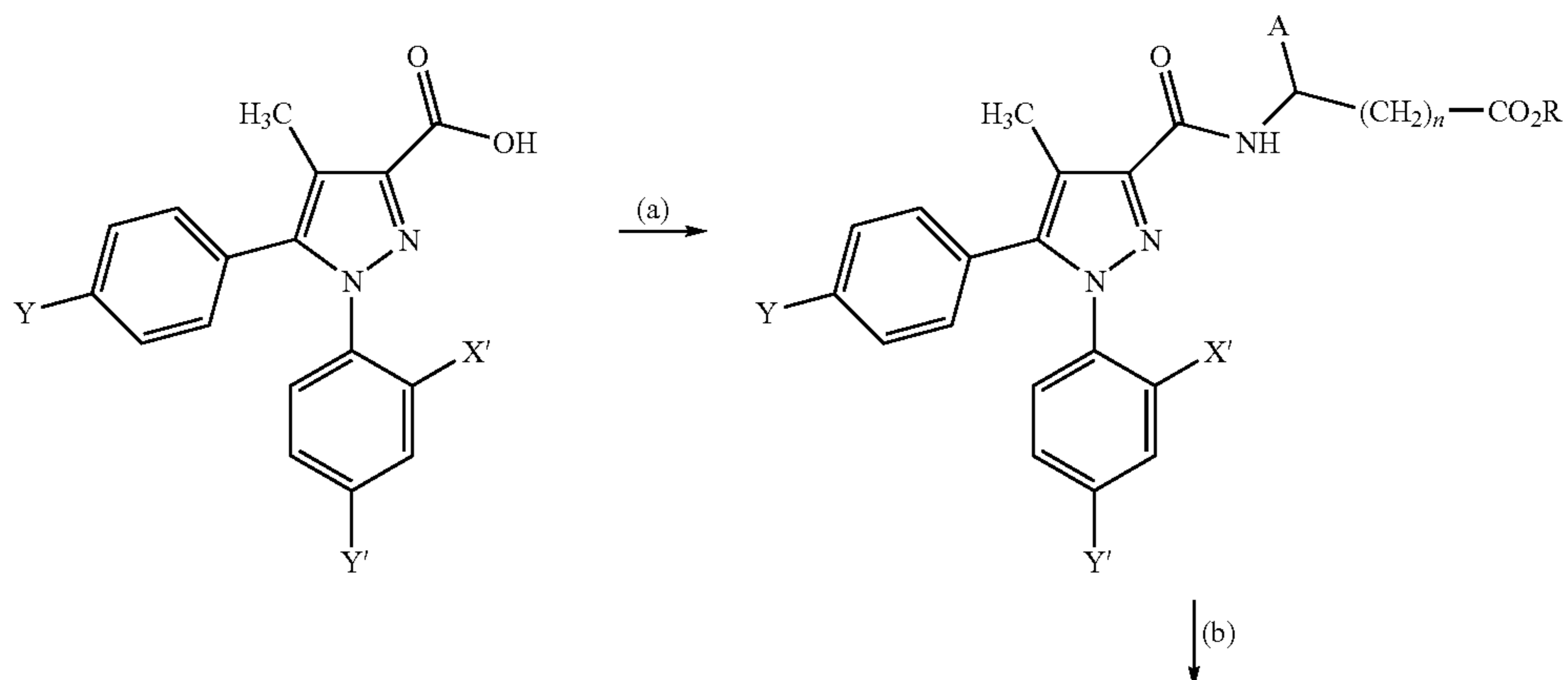
Scheme 3
