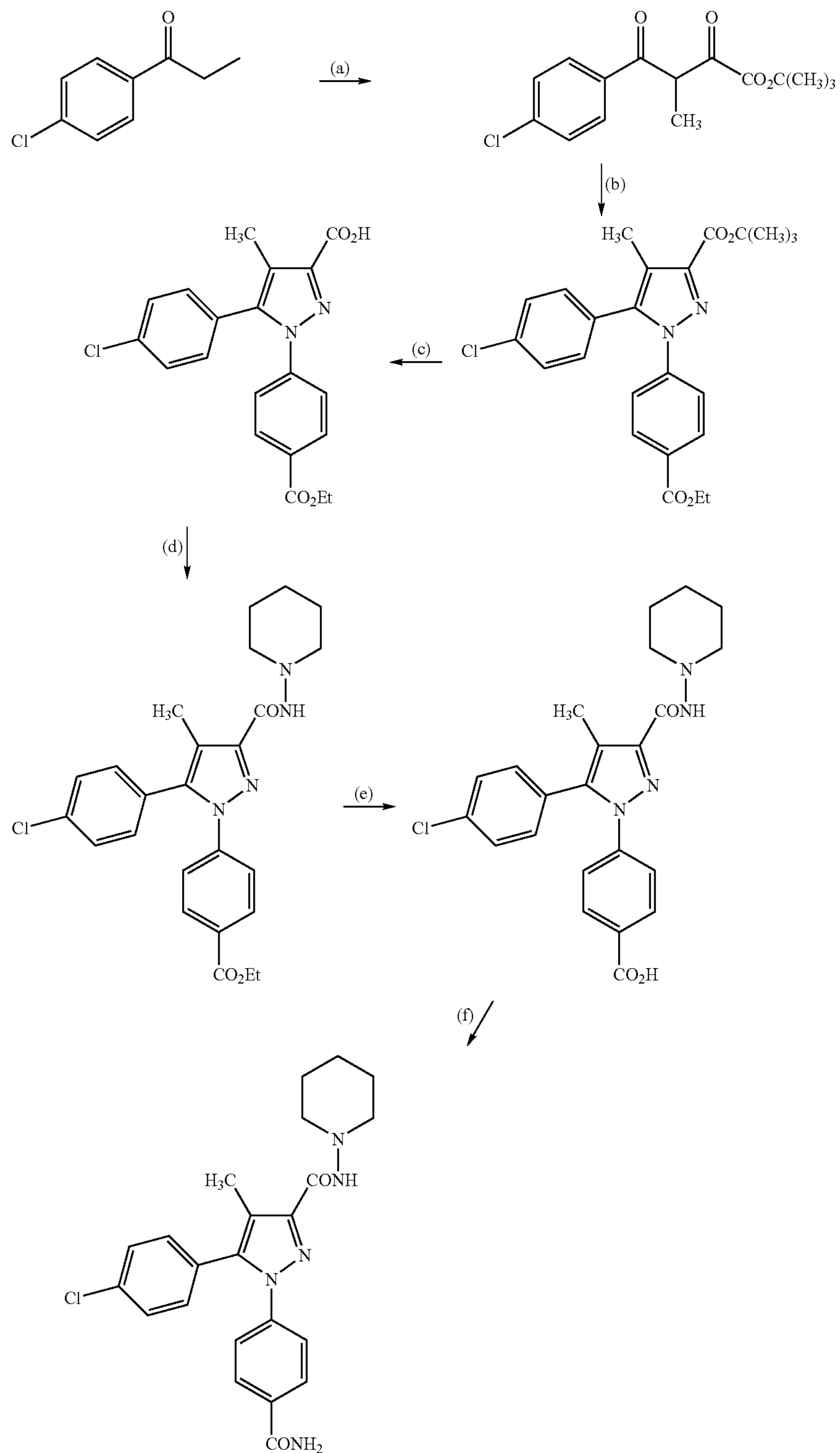
Scheme 8
