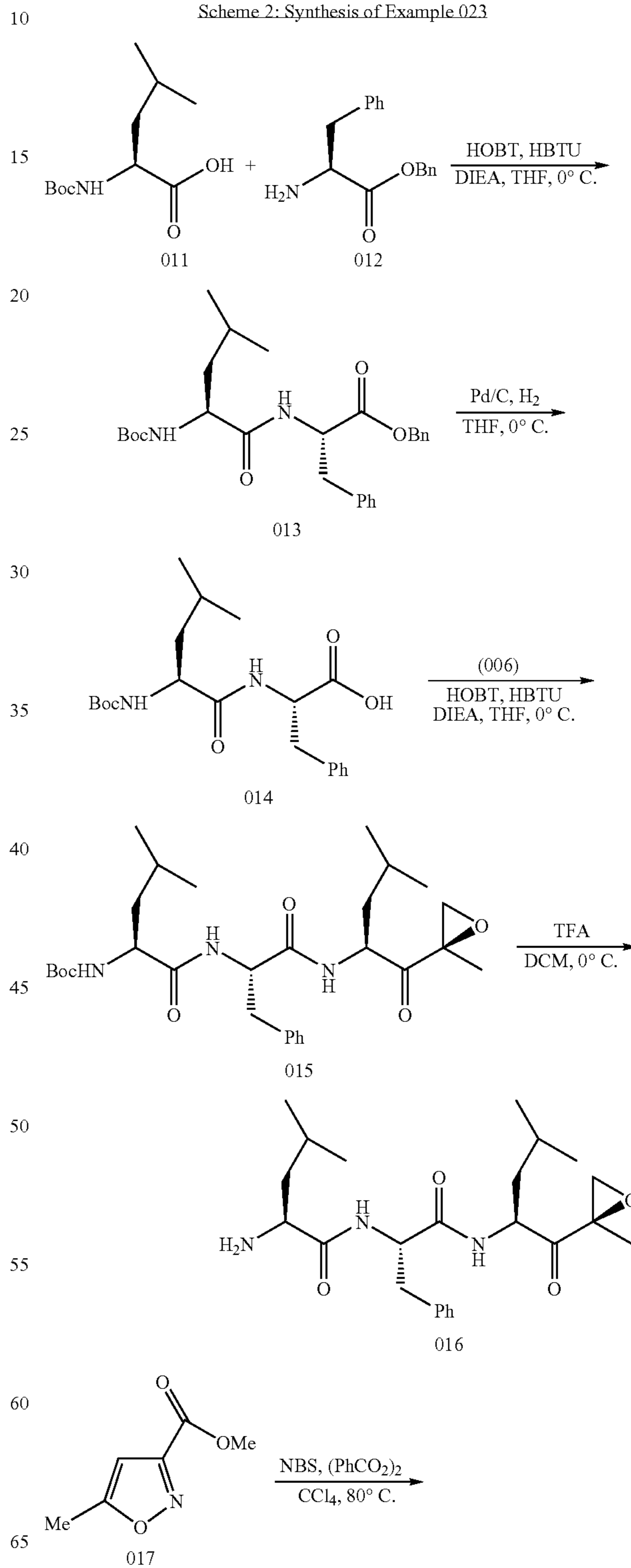
Scheme 2: Synthesis of Example 023
