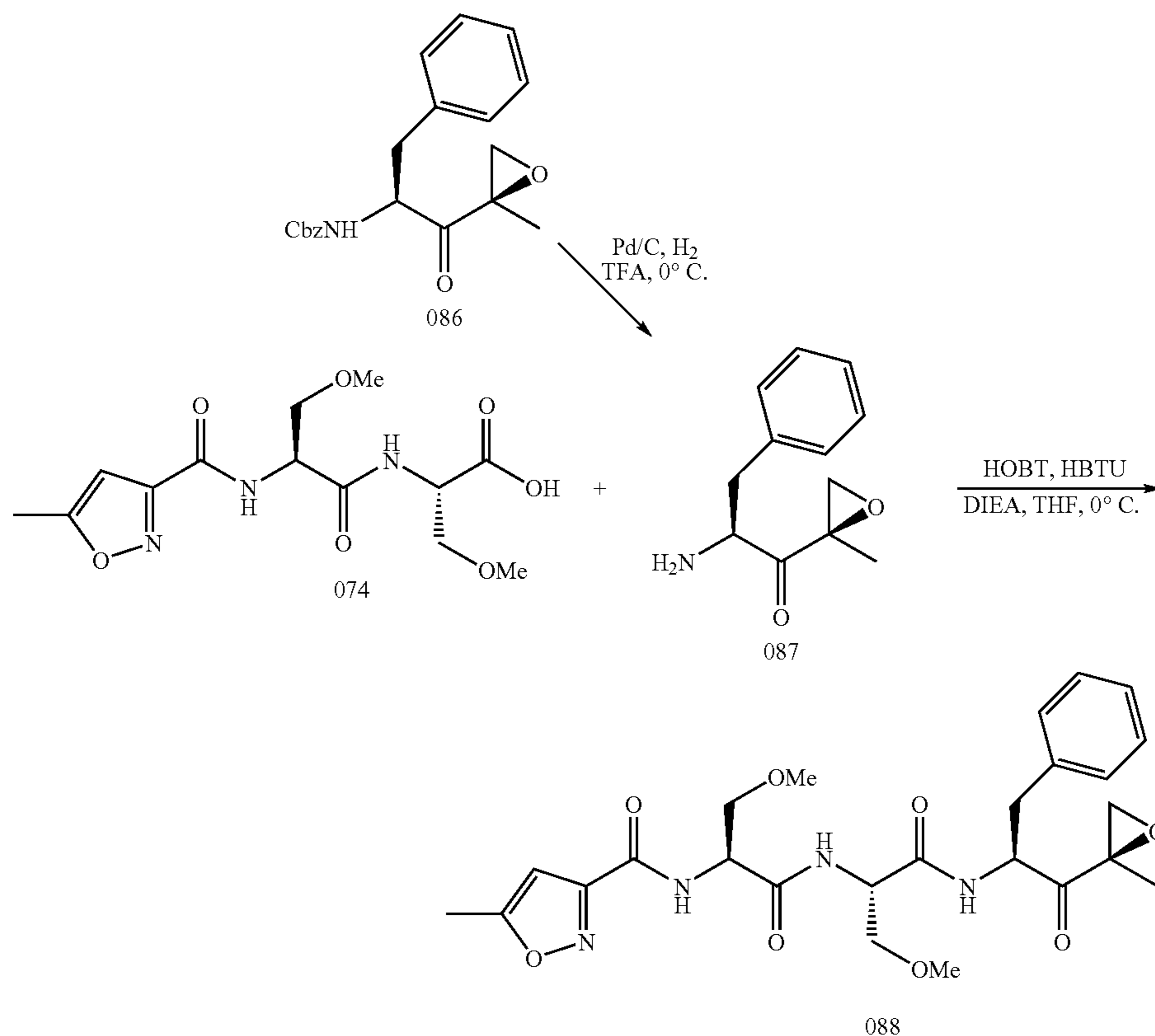
Scheme 15: Synthesis of Example 088
