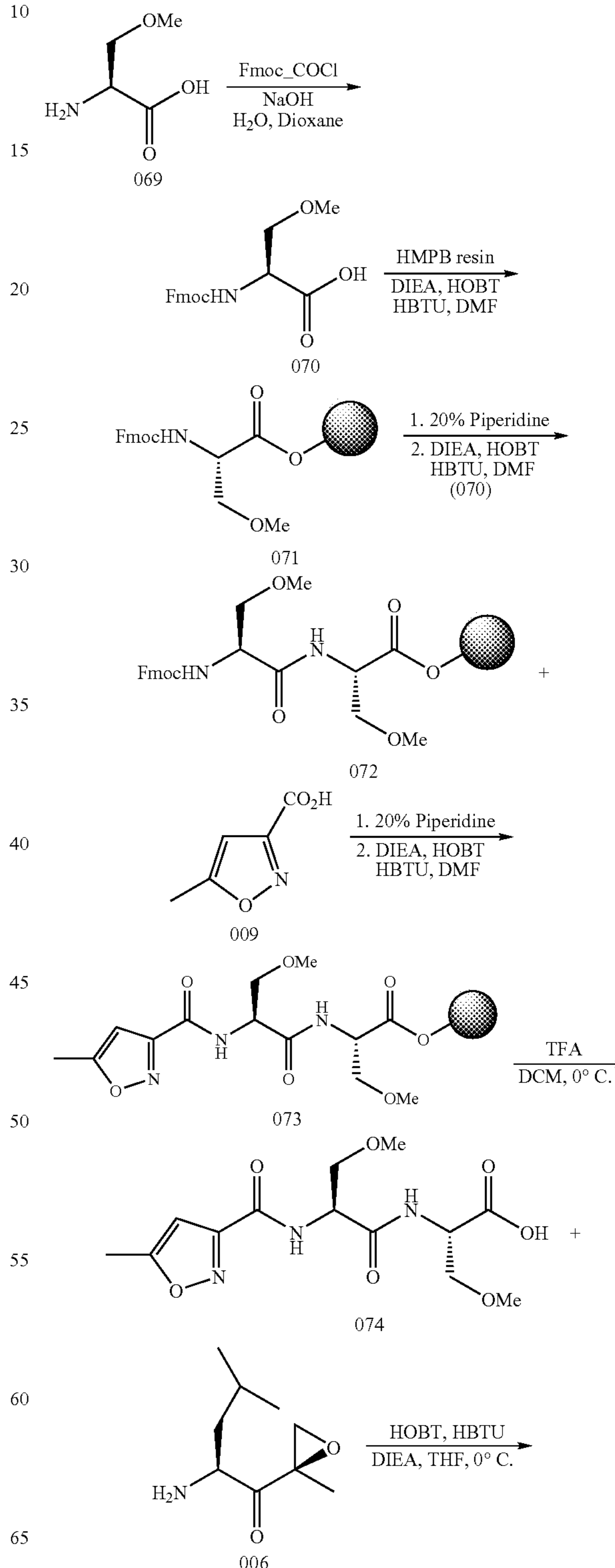
Scheme 11: Synthesis of Example 075 (approach A)
