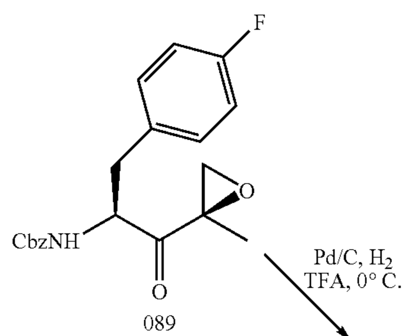
Scheme 16: Synthesis of Example 091
