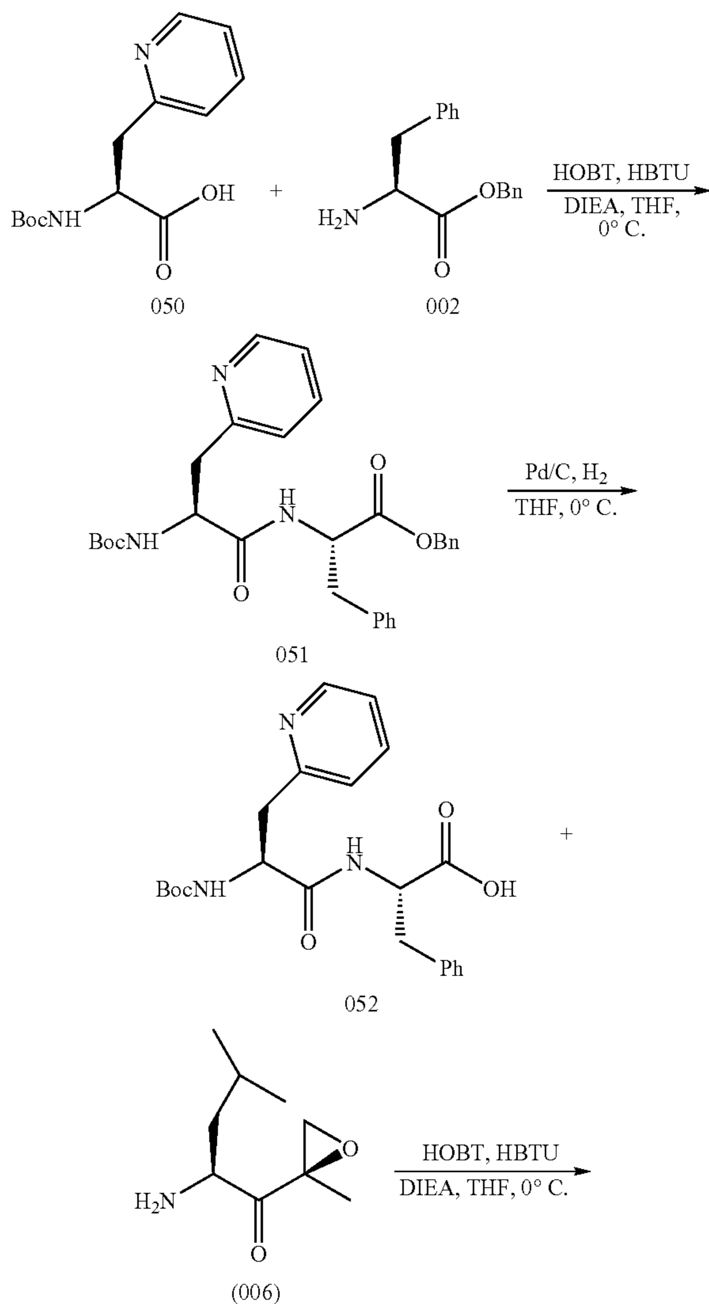
Scheme 8: Synthesis of Example 055
