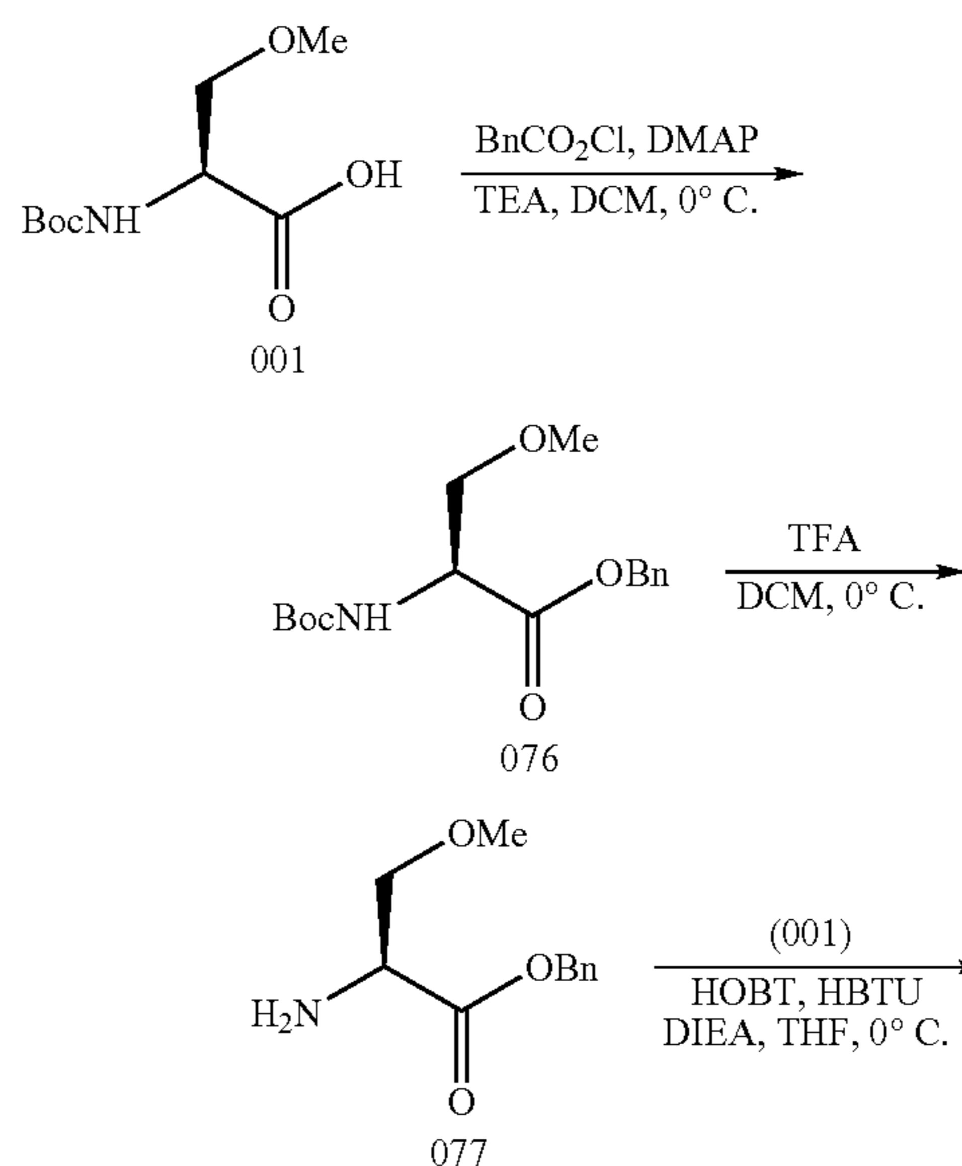
Scheme 12: Synthesis of Example 075 (approach B)
