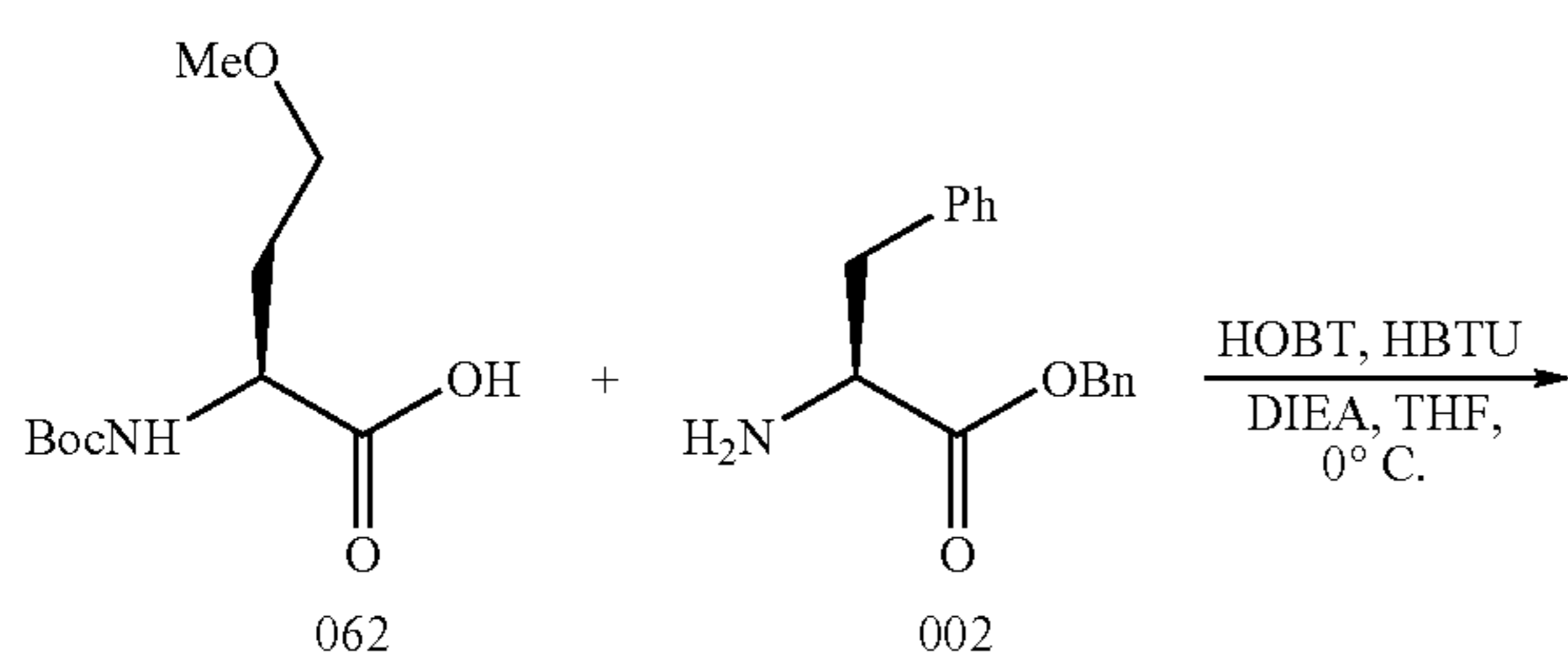
Scheme 10: Synthesis of Example 068
