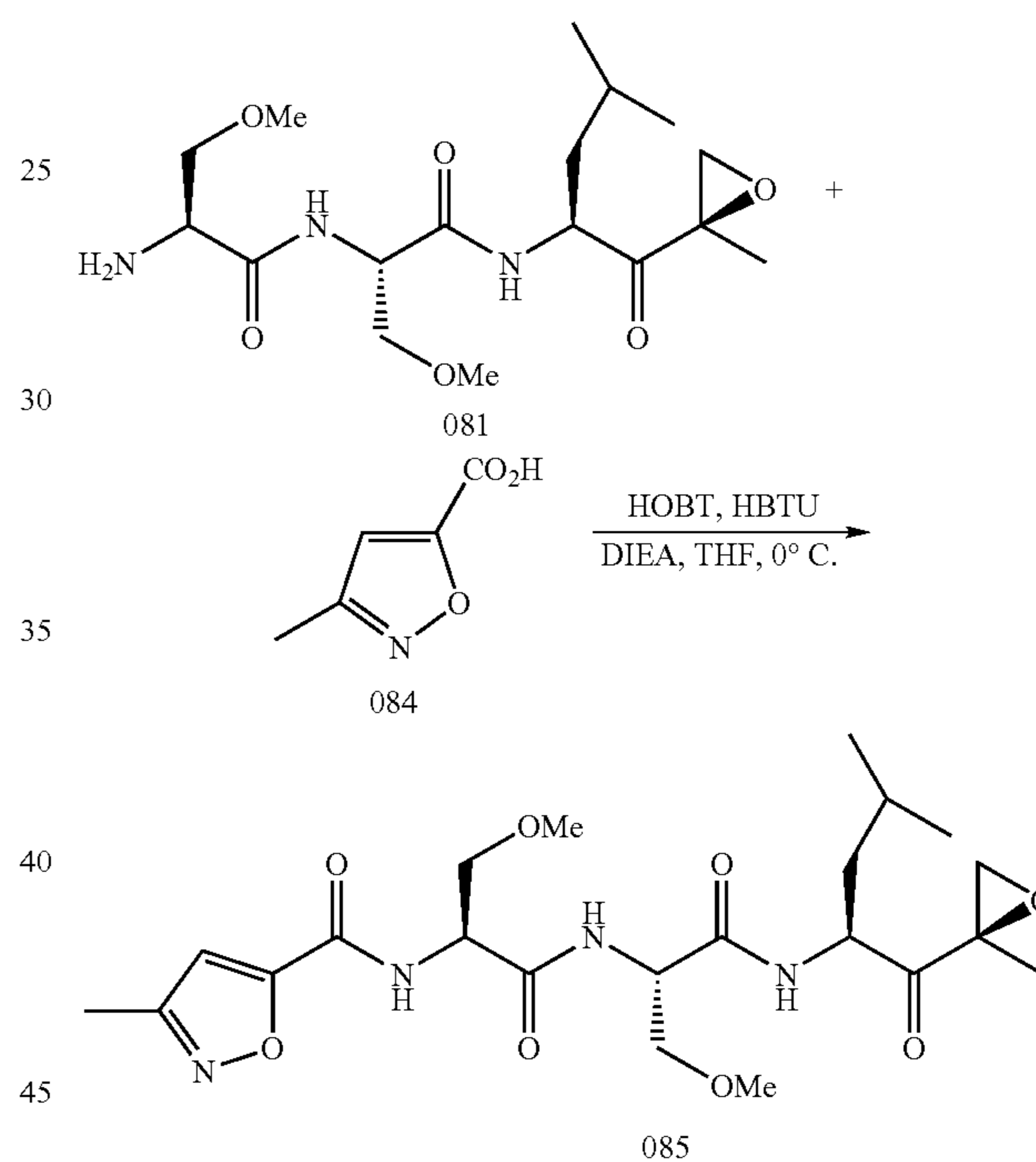
Scheme 14: Synthesis of Example 085
