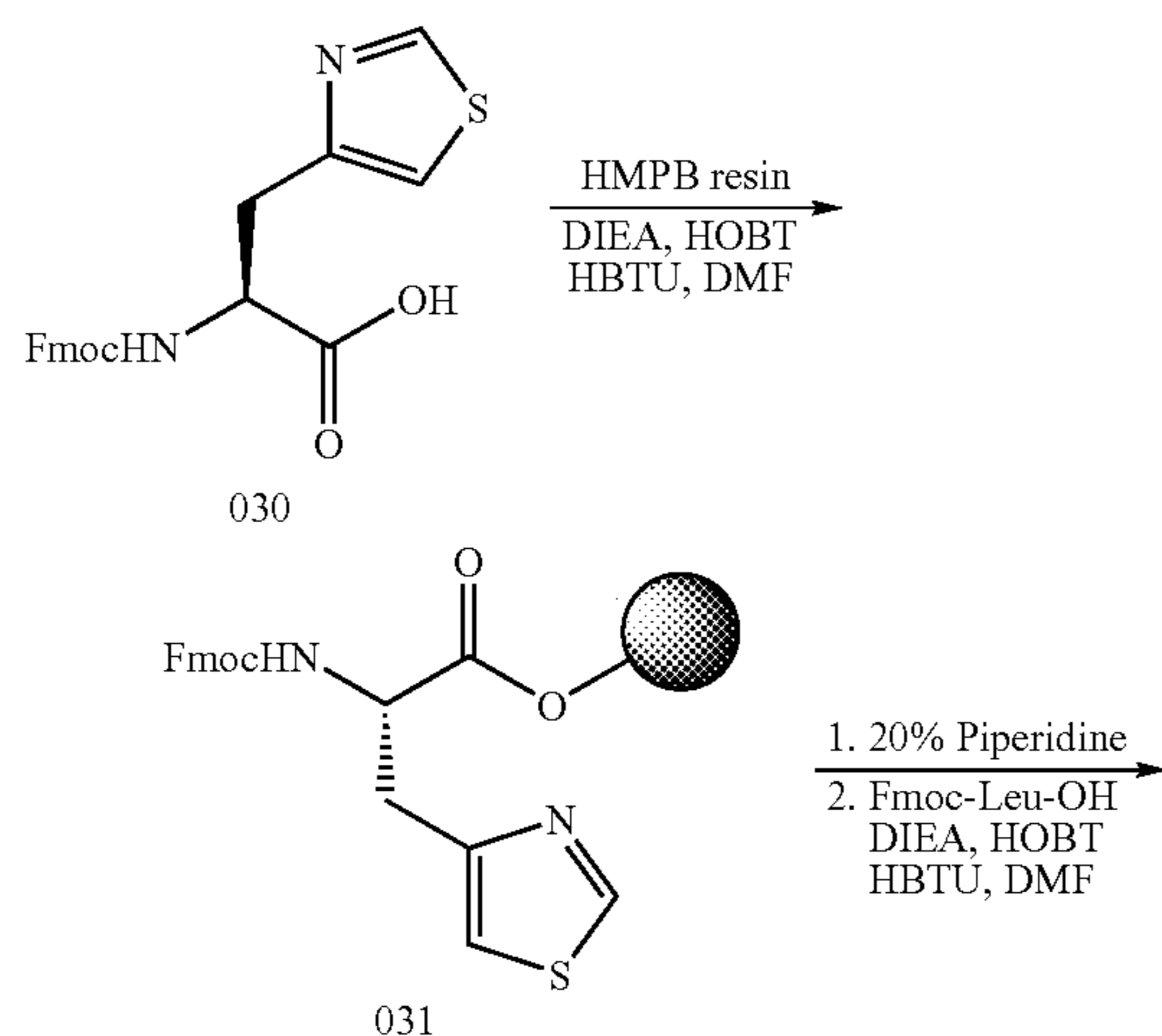
Scheme 4: Synthesis of Example 035
