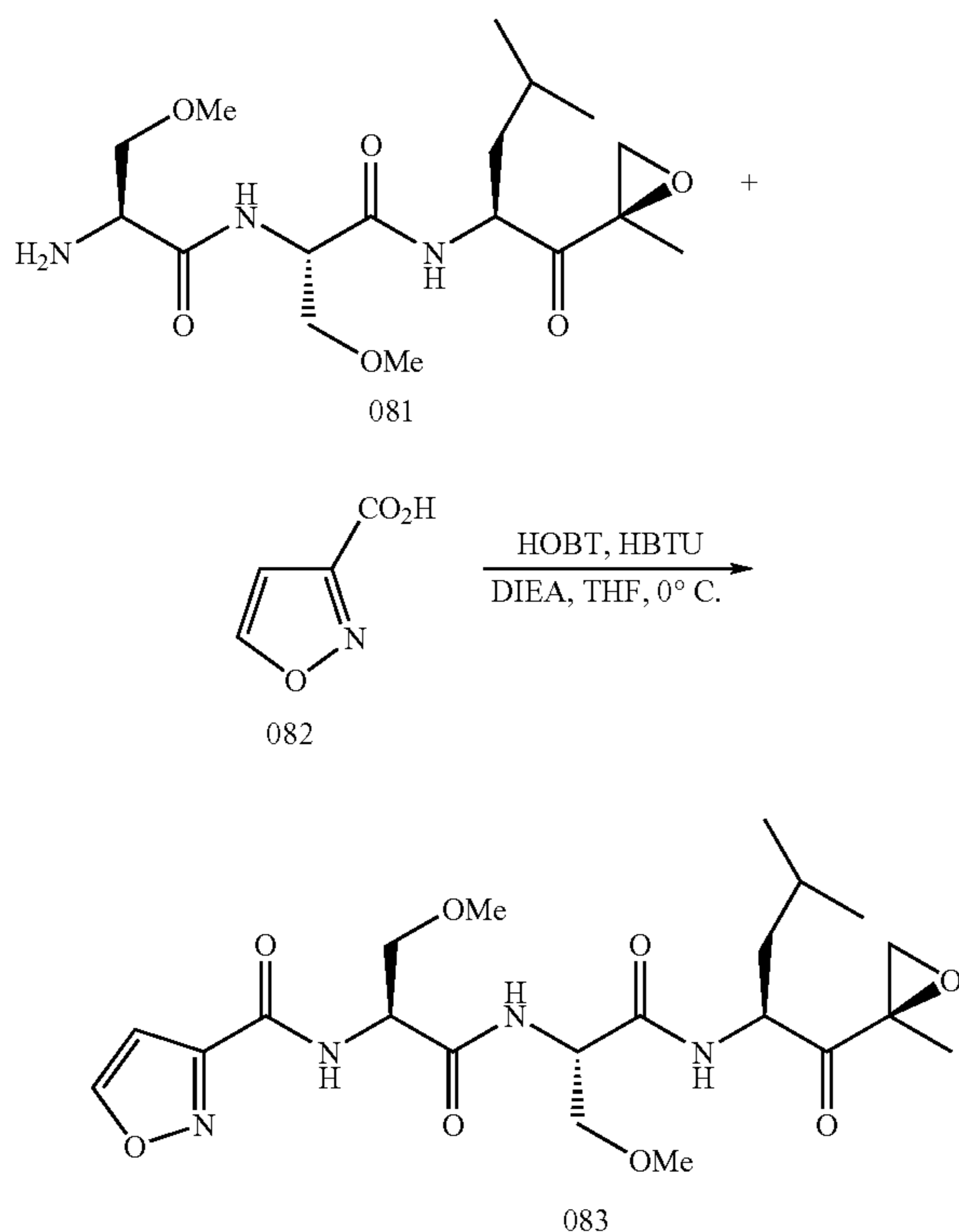
Scheme 13: Synthesis of Example 083
