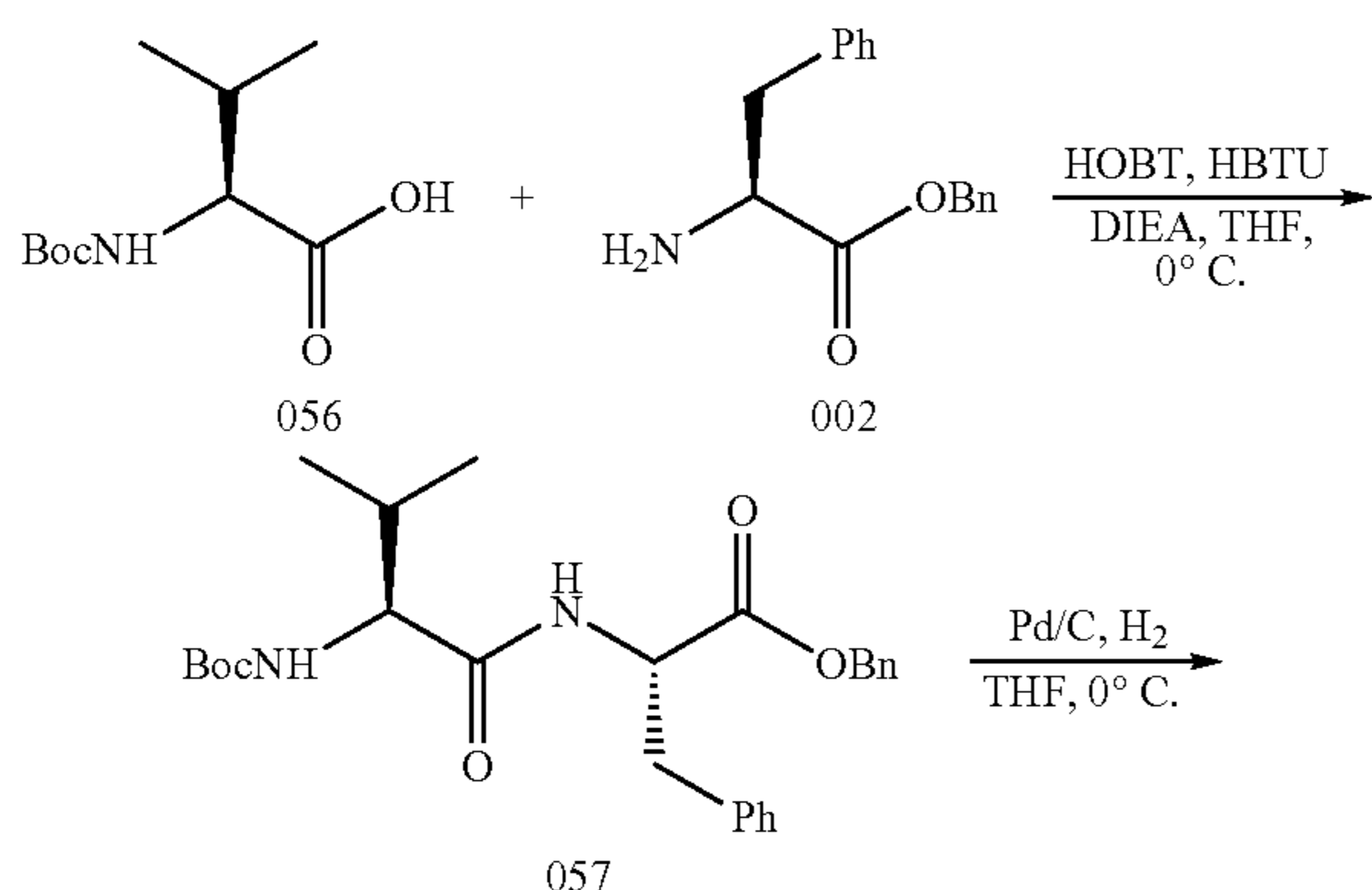
Scheme 9: Synthesis of Example 061
