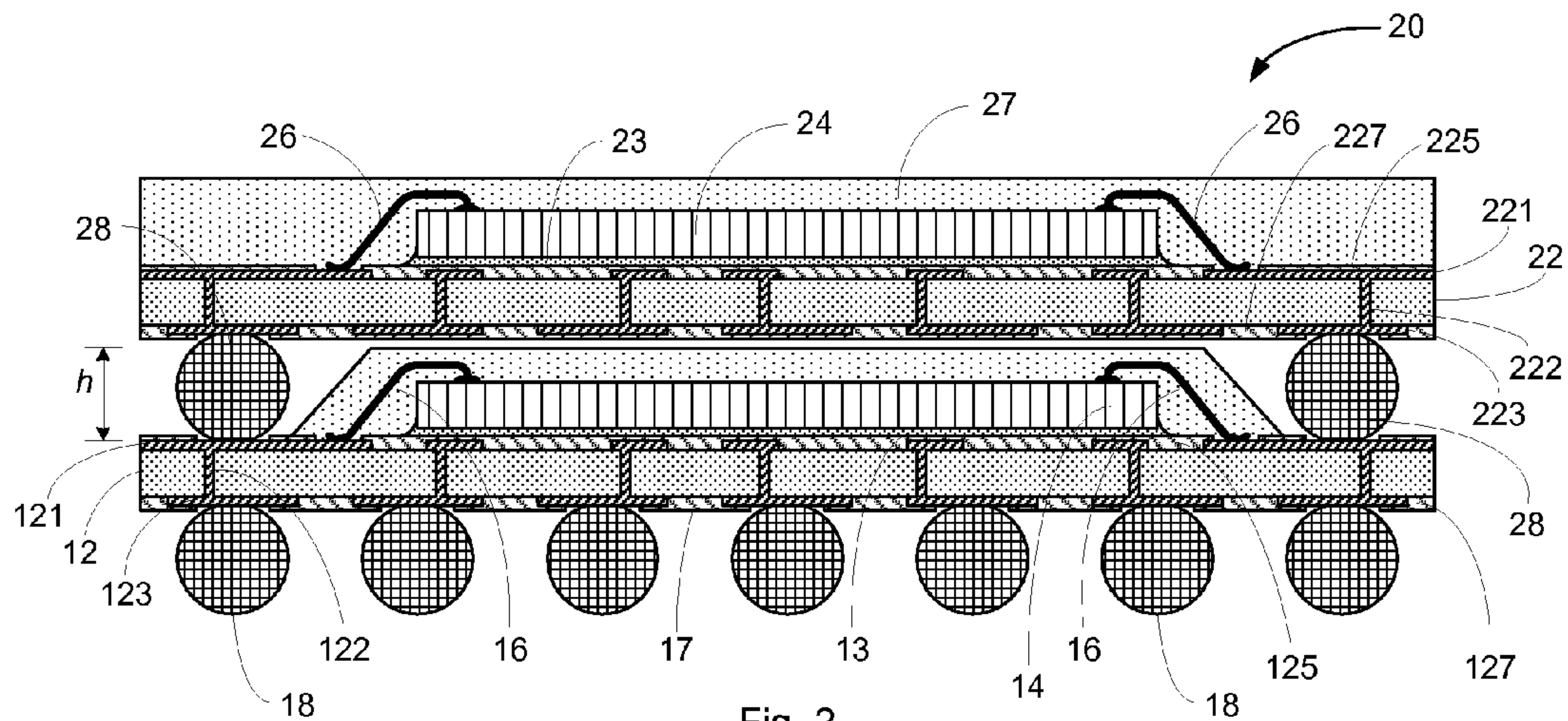
Fig. 2 PRIOR ART
