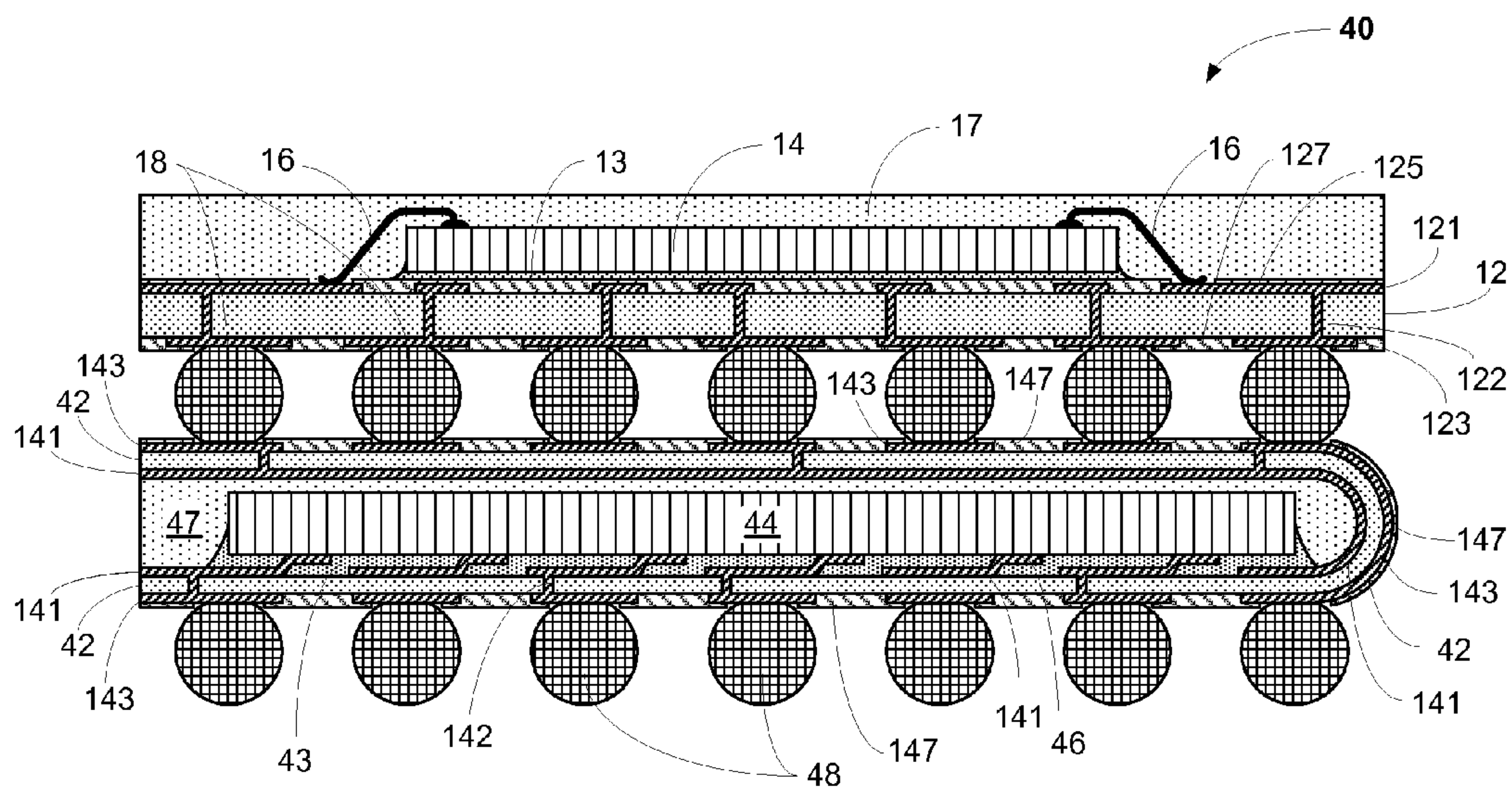
Fig. 4 PRIOR ART
