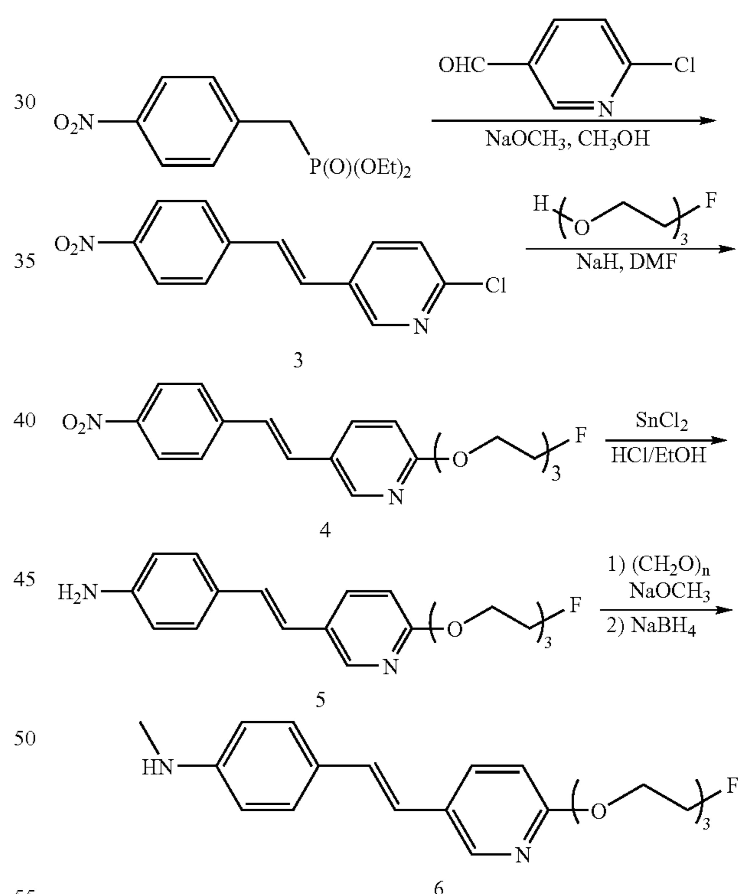
SCHEME 2
