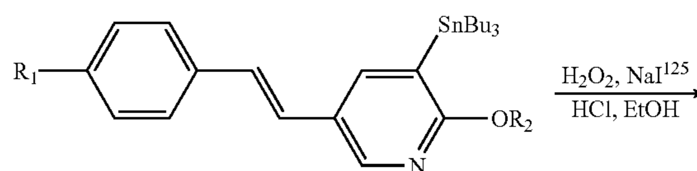
SCHEME 7
