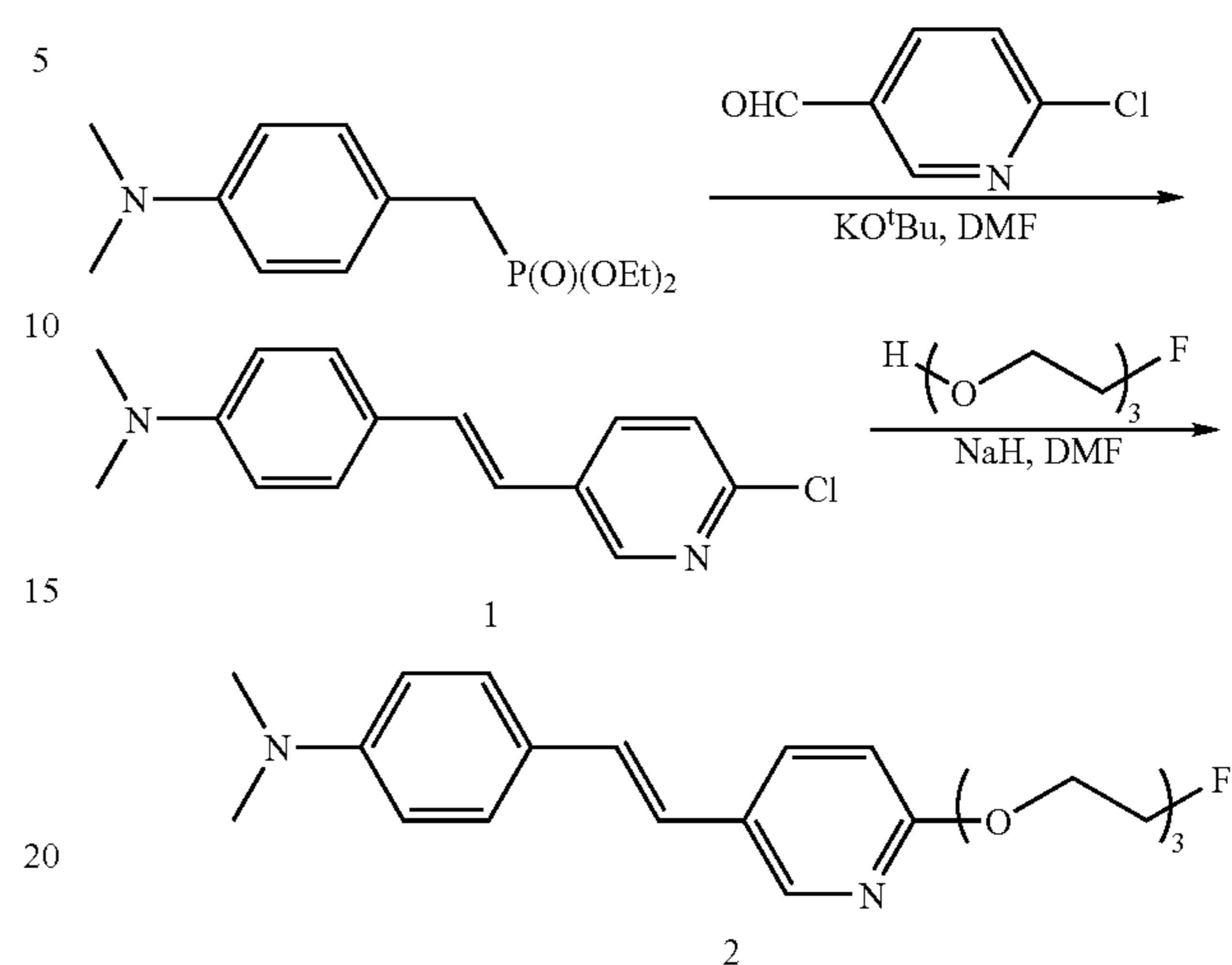
SCHEME 1
