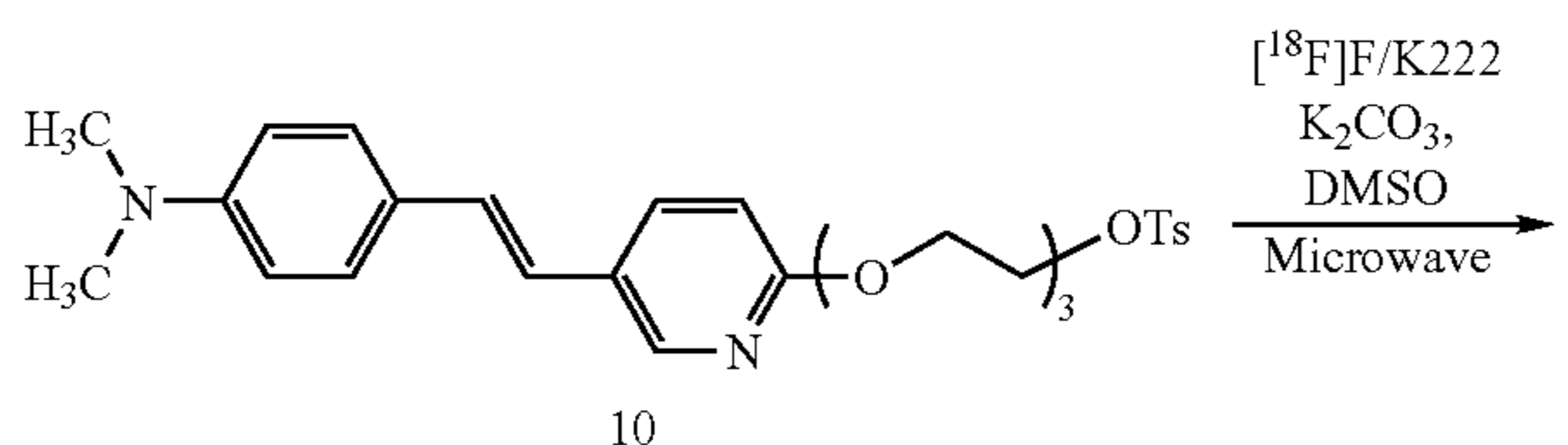
SCHEME 4
