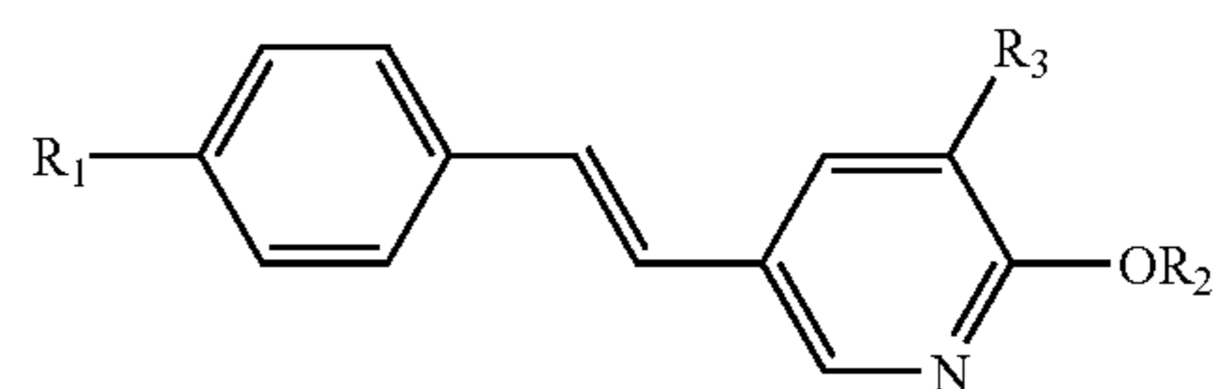
SCHEME 6
