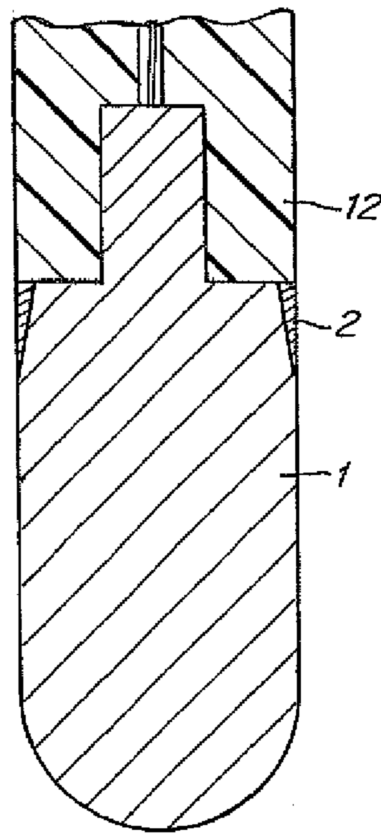
Fig. 1 PRIOR ART
