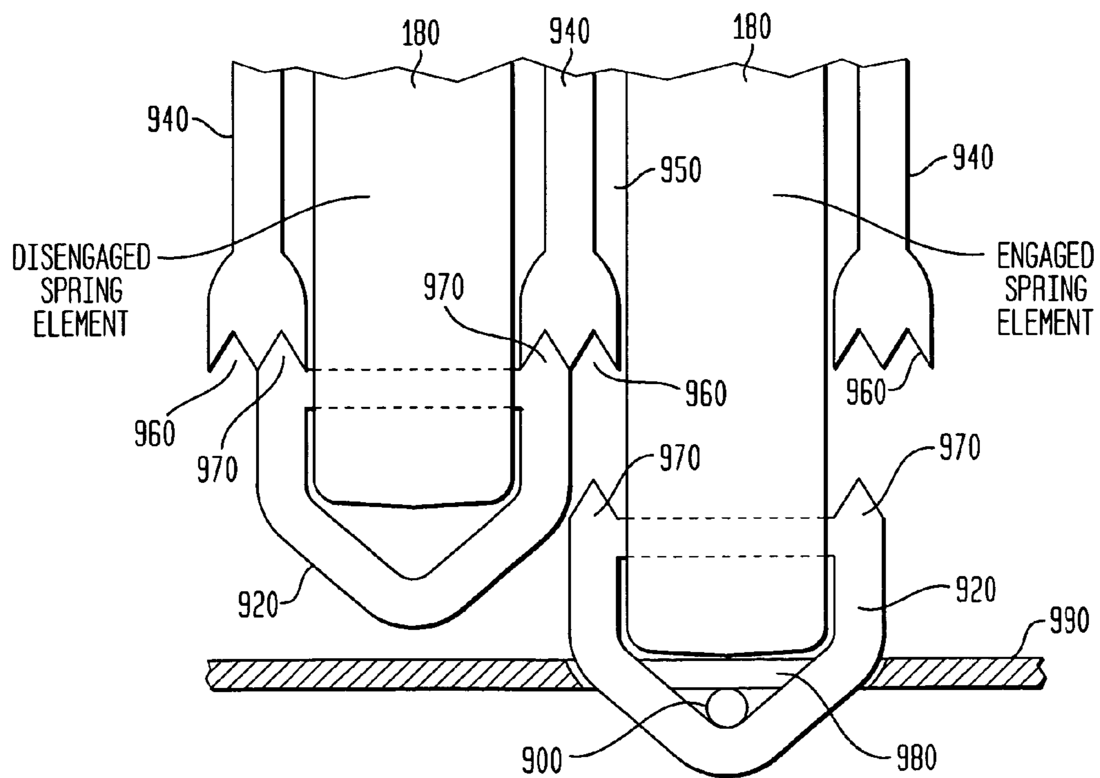
CUTAWAY SIDE VIEW OF LOWER MOUNT
