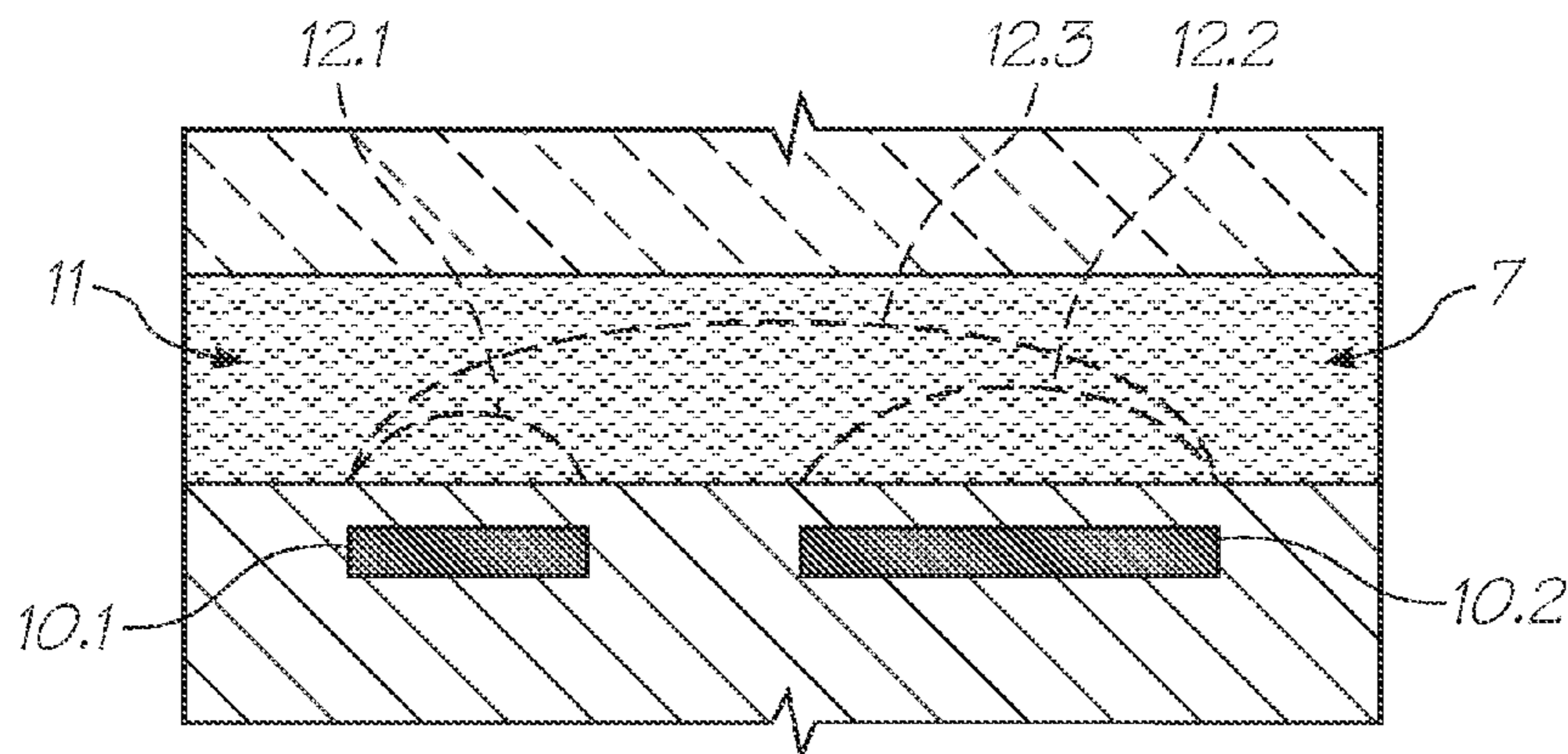
FIG. 52 (PRIOR ART)
