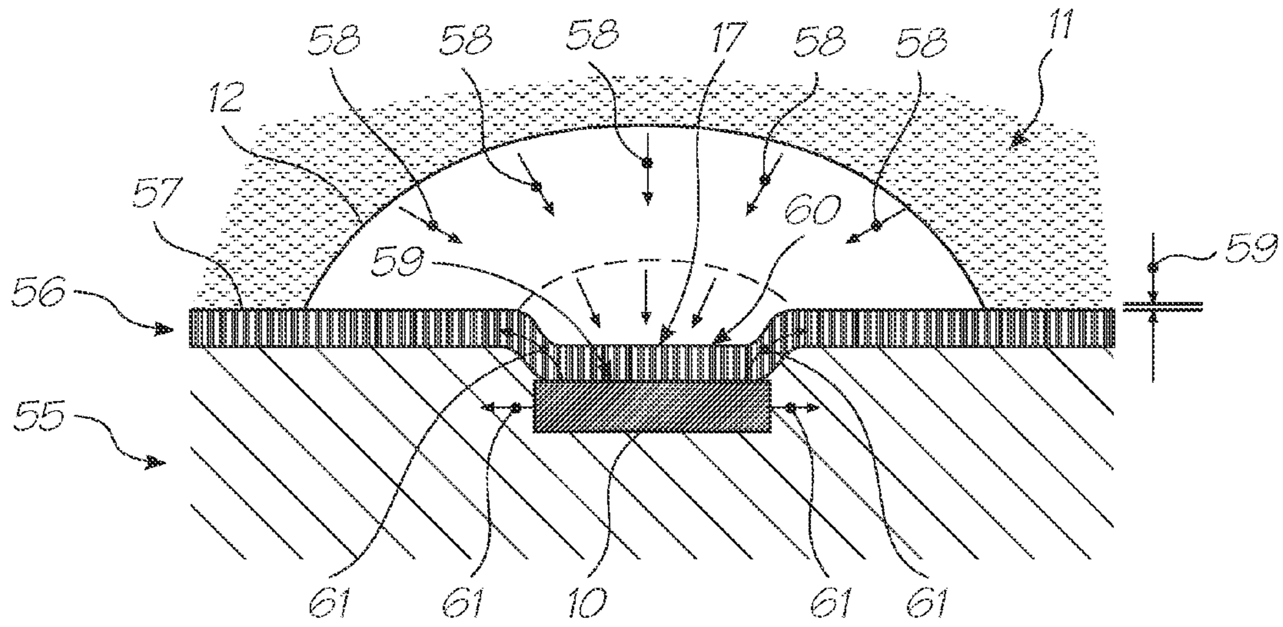
FIG. 47 (PRIOR ART)
