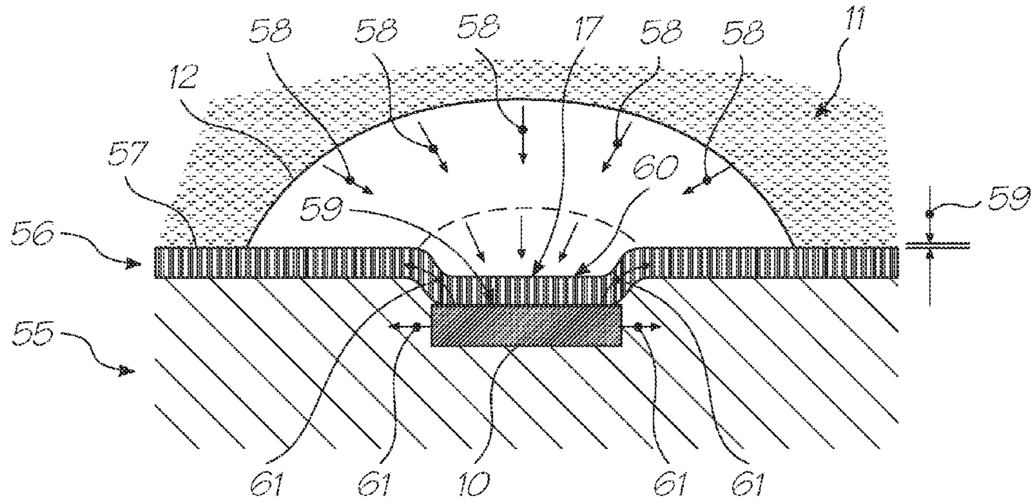
FIG. 57 (PRIOR ART)
