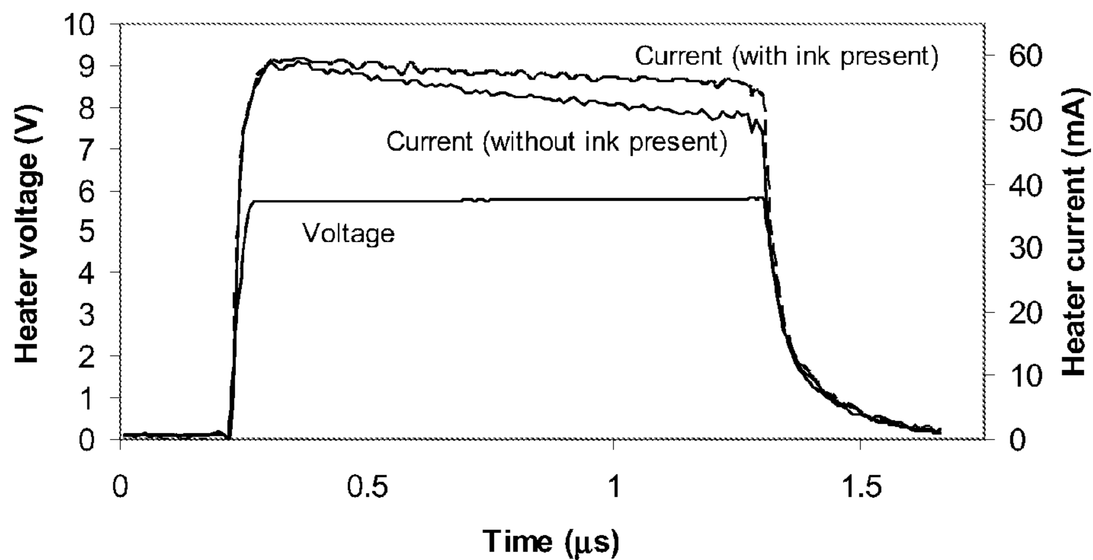
Using a suspended heater to detect the presence of ink
