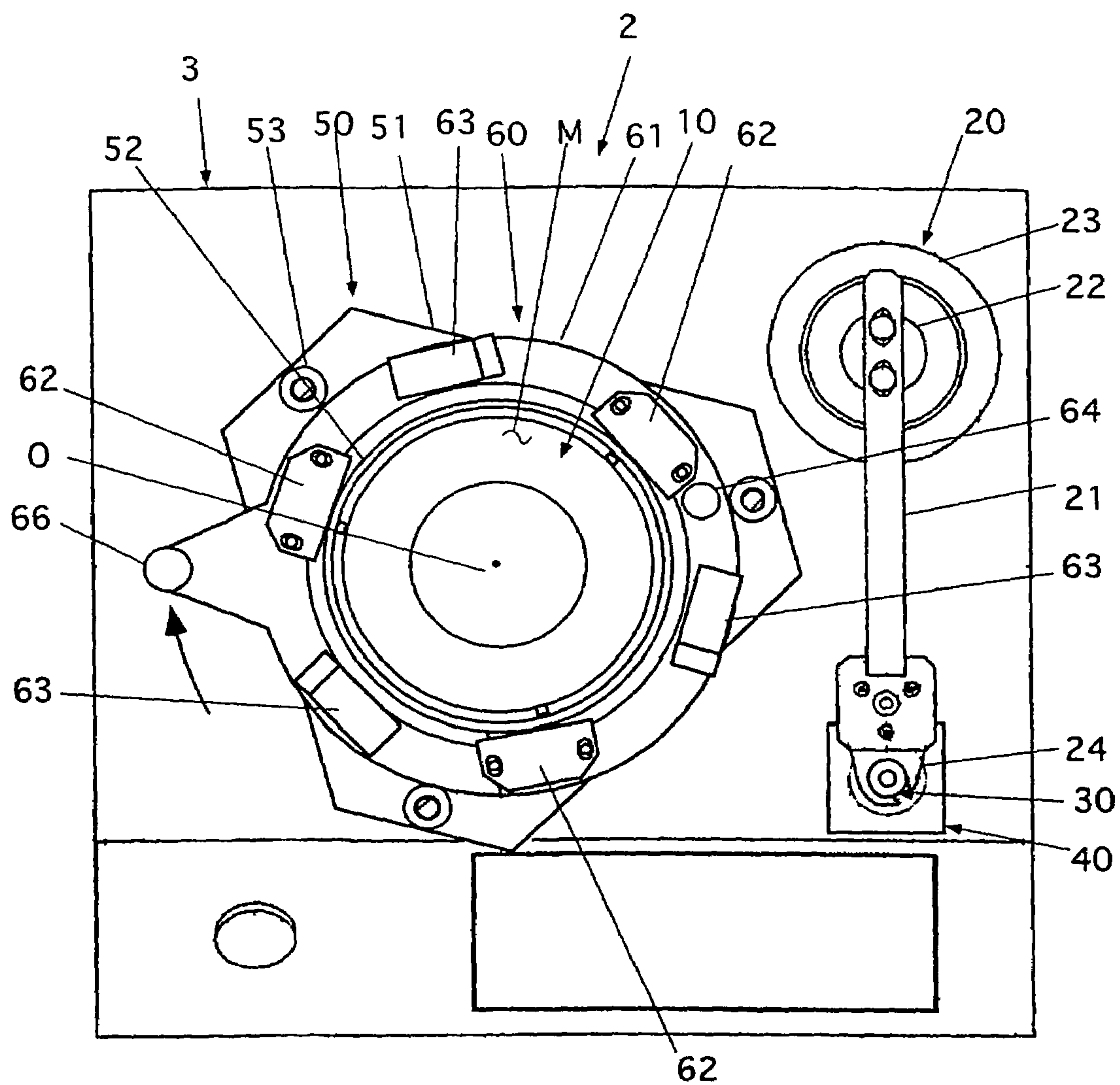
III - III CROSS SECTION
