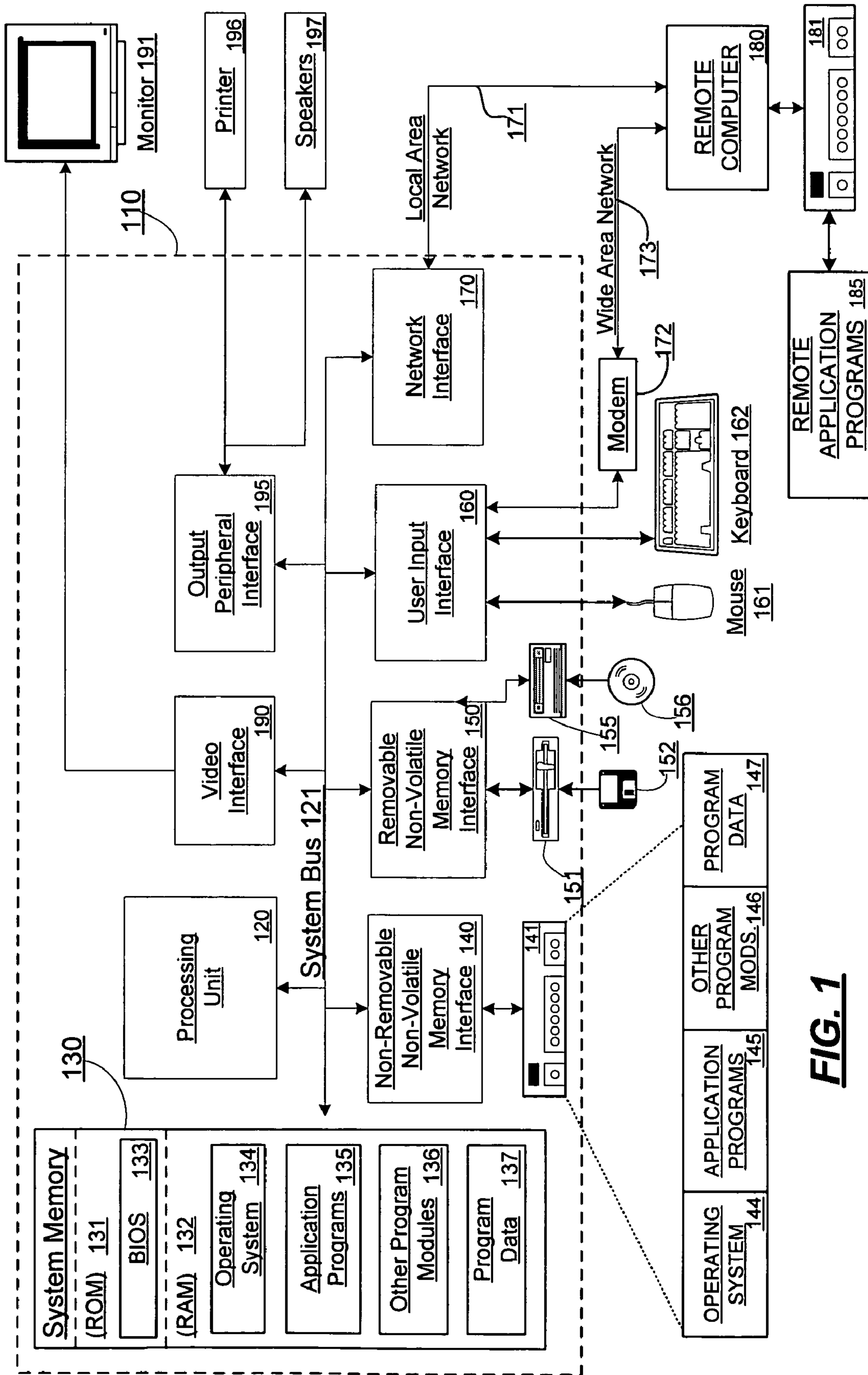
Computing Environment 100
