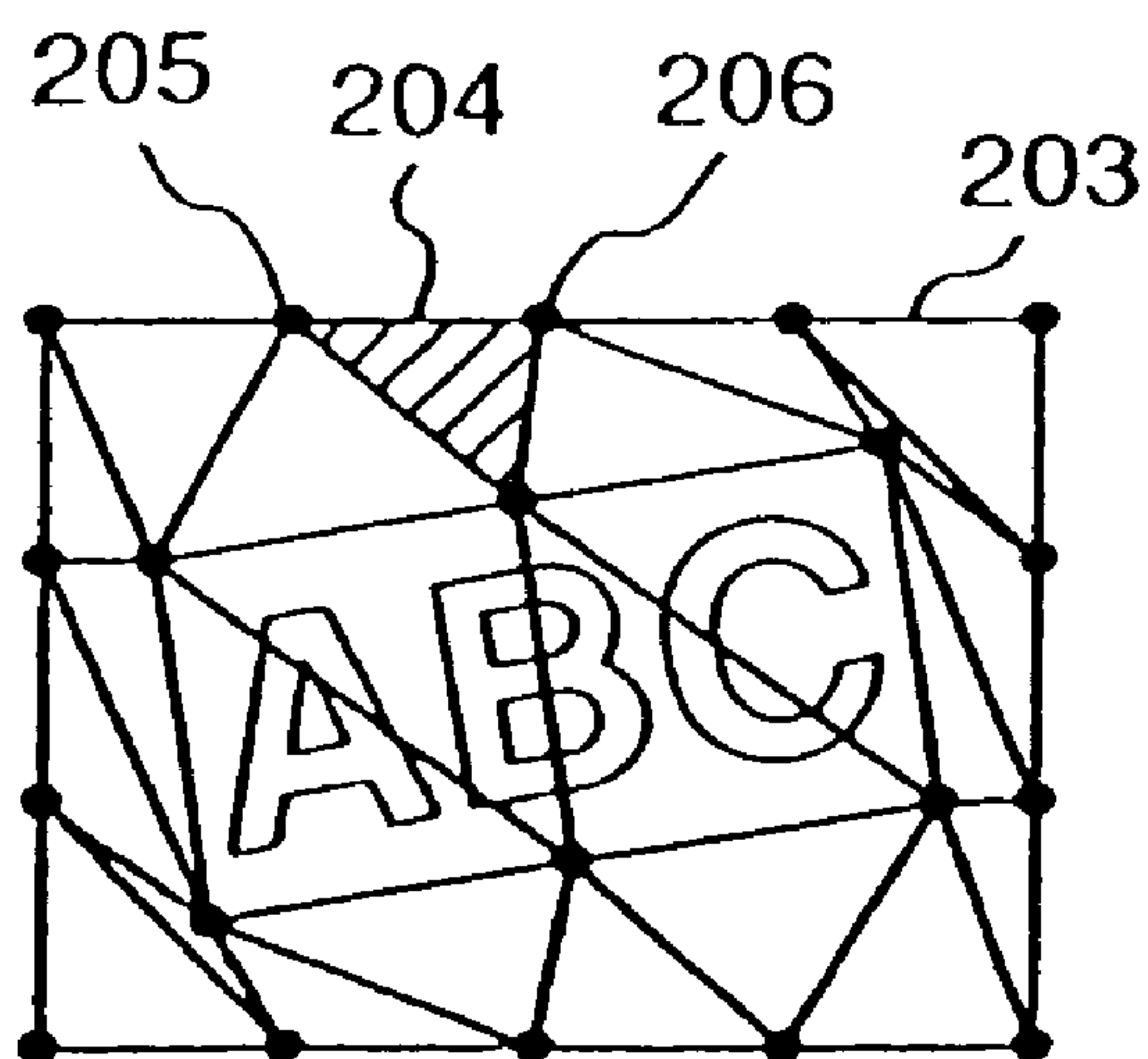
PATCHES AND GRID POINTS IN THE REFERENCE IMAGE AFTER MOTION ESTIMATION
