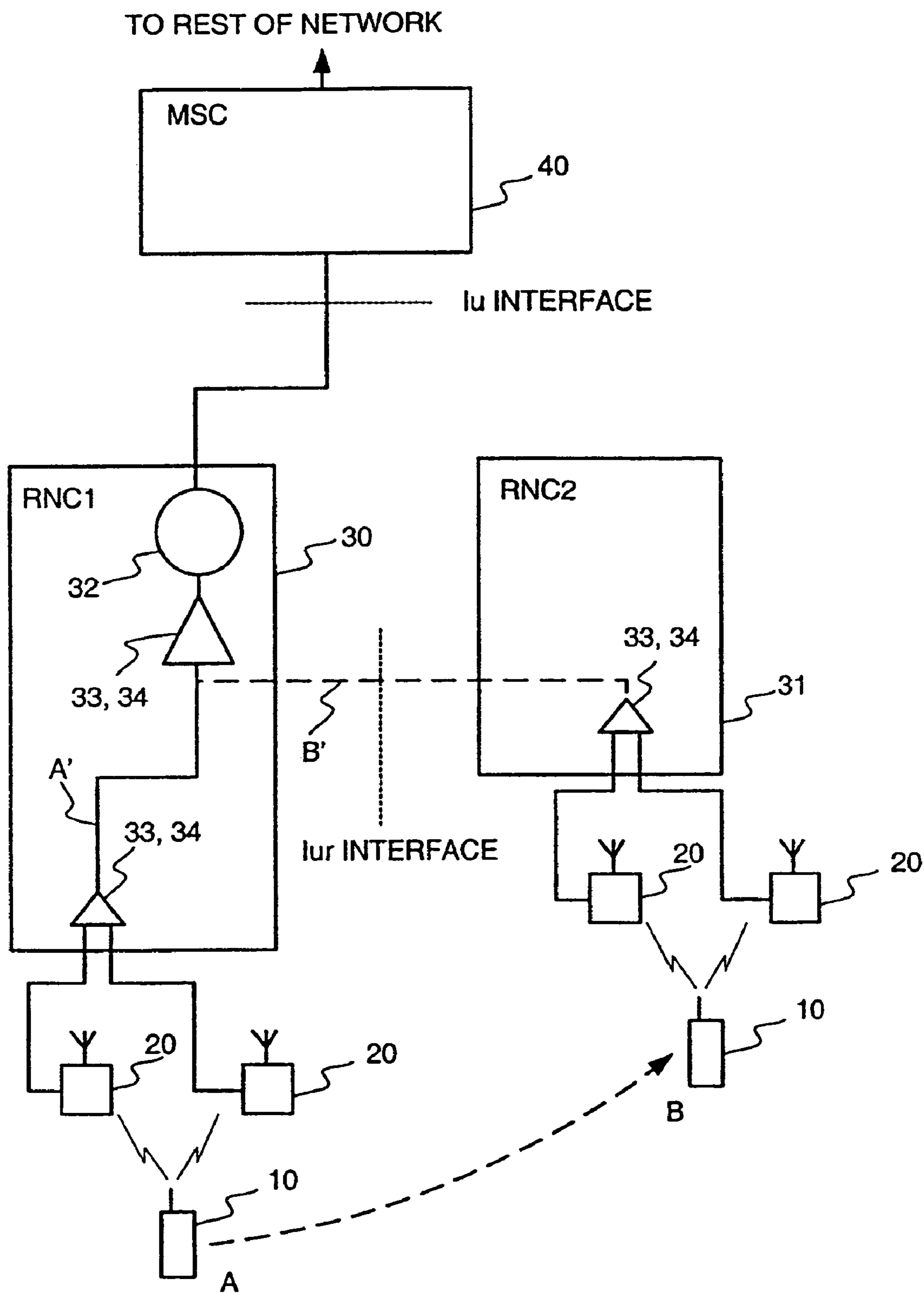
Fig. 1 PRIOR ART
