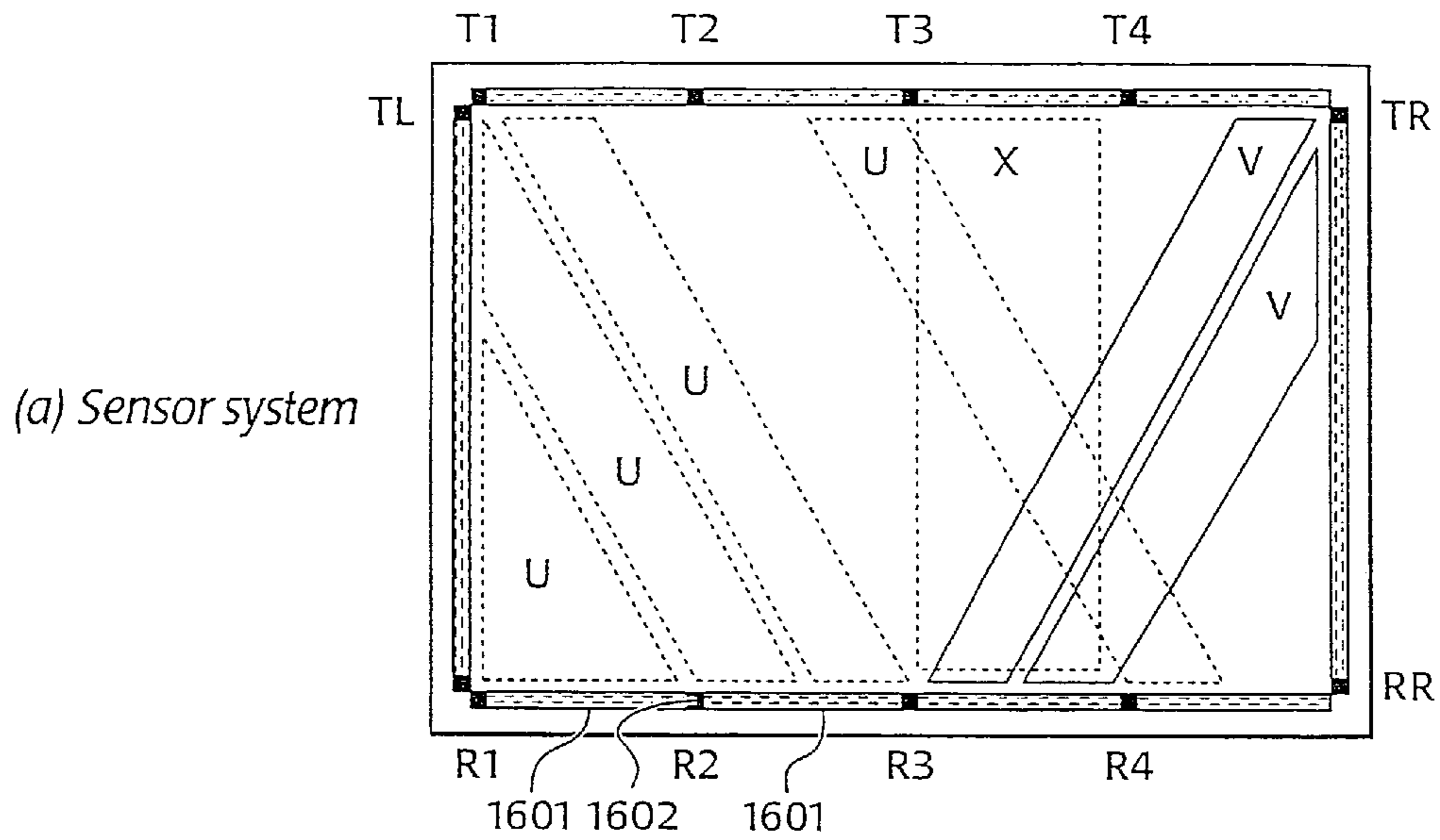
Fig. 16 - Large rectangular sensor
