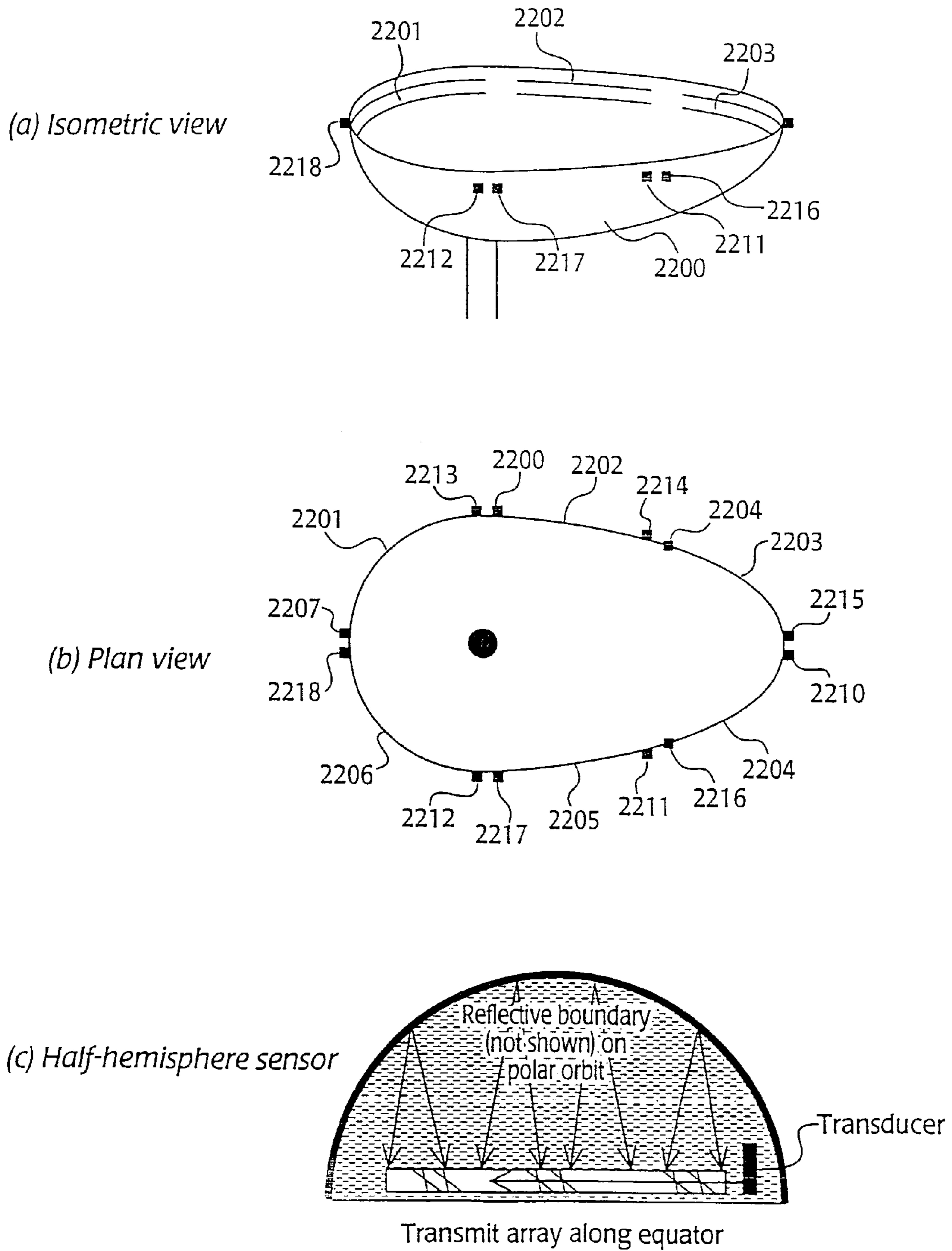
Fig. 22 - Basin sensor
