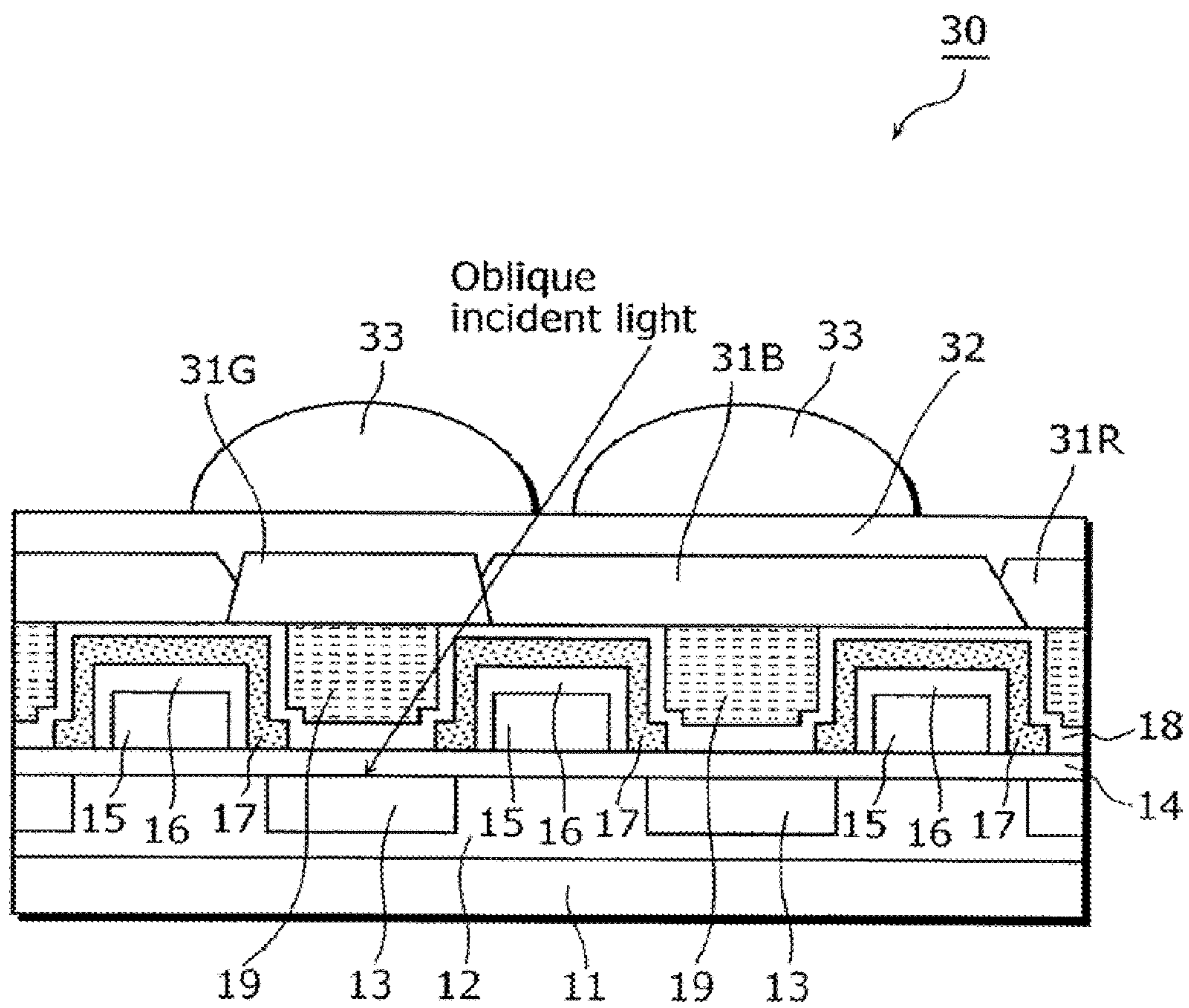
FIG. 1 PRIOR ART
