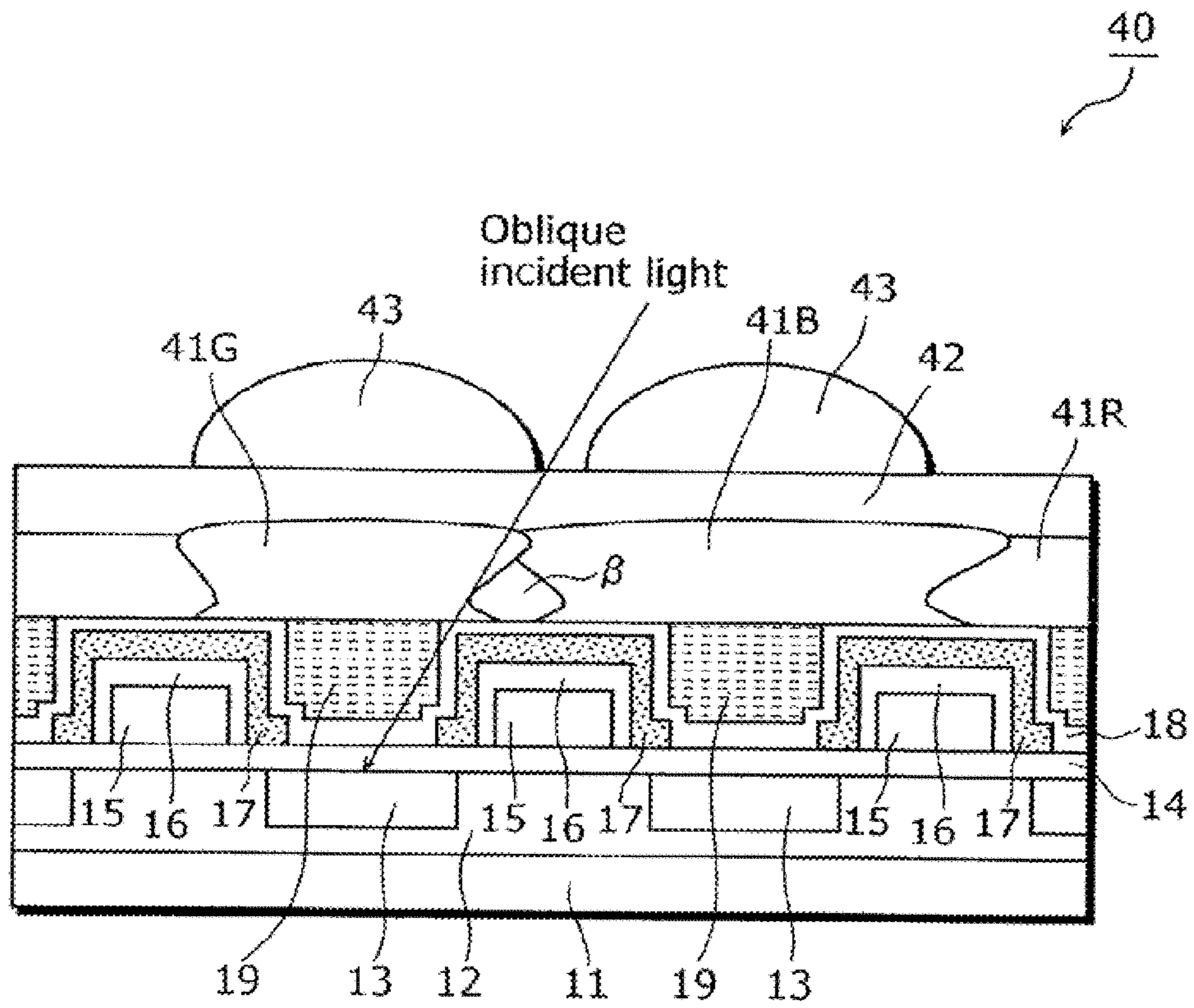
FIG. 3 PRIOR ART
