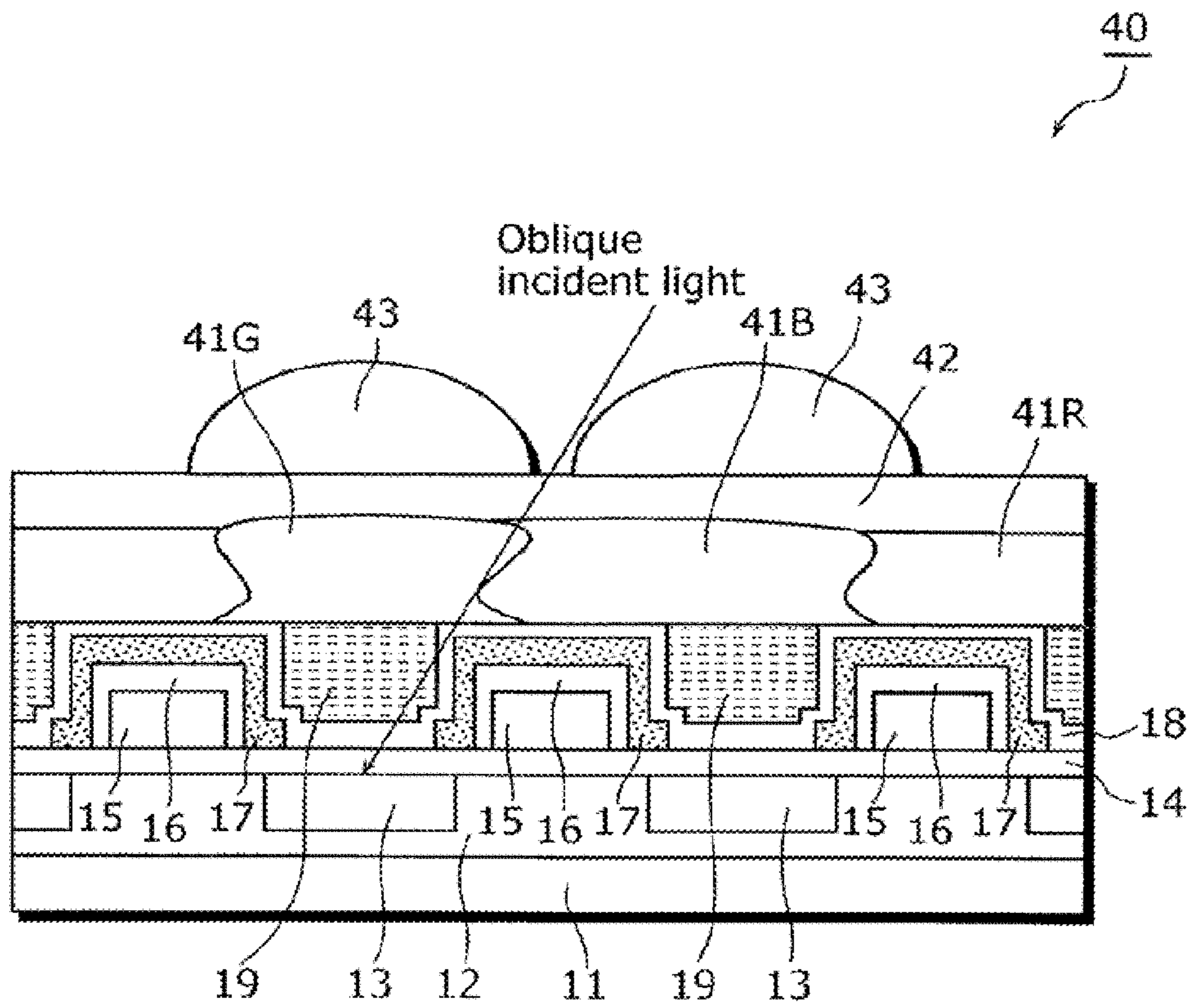
FIG. 2 PRIOR ART
