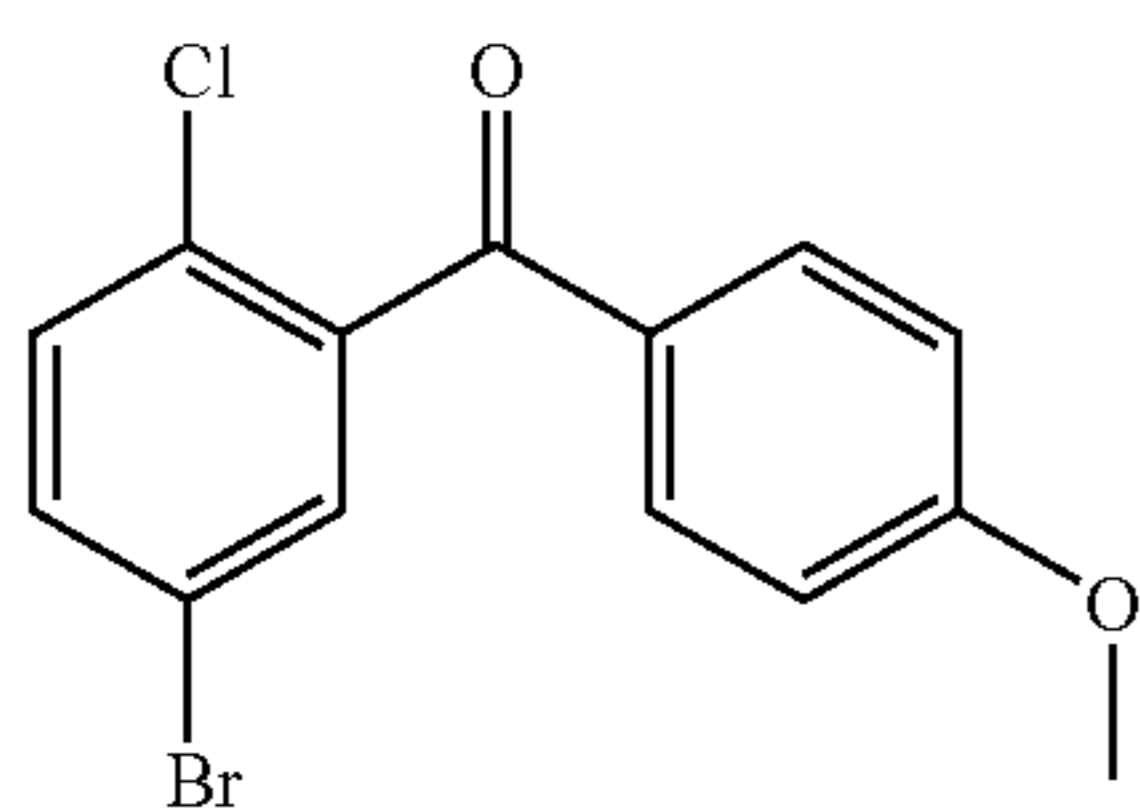
(5-Bromo-2-chloro-phenyl)-(4-methoxy-phenyl)-methanone
