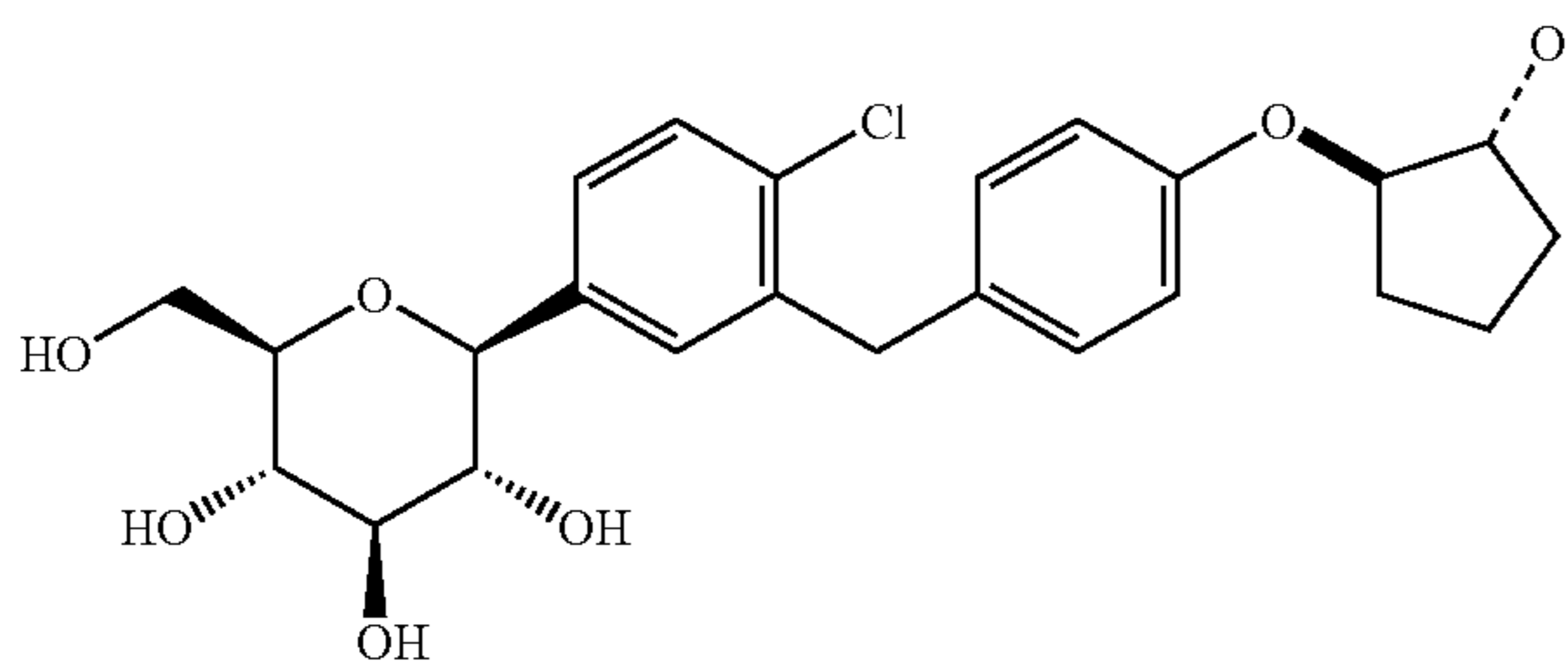
1-Chloro-4-(β-D-glucopyranos-1-yl)-2-[4-(trans-2-hydroxy-cyclopent-1-yloxy)-benzyl]-benzene
