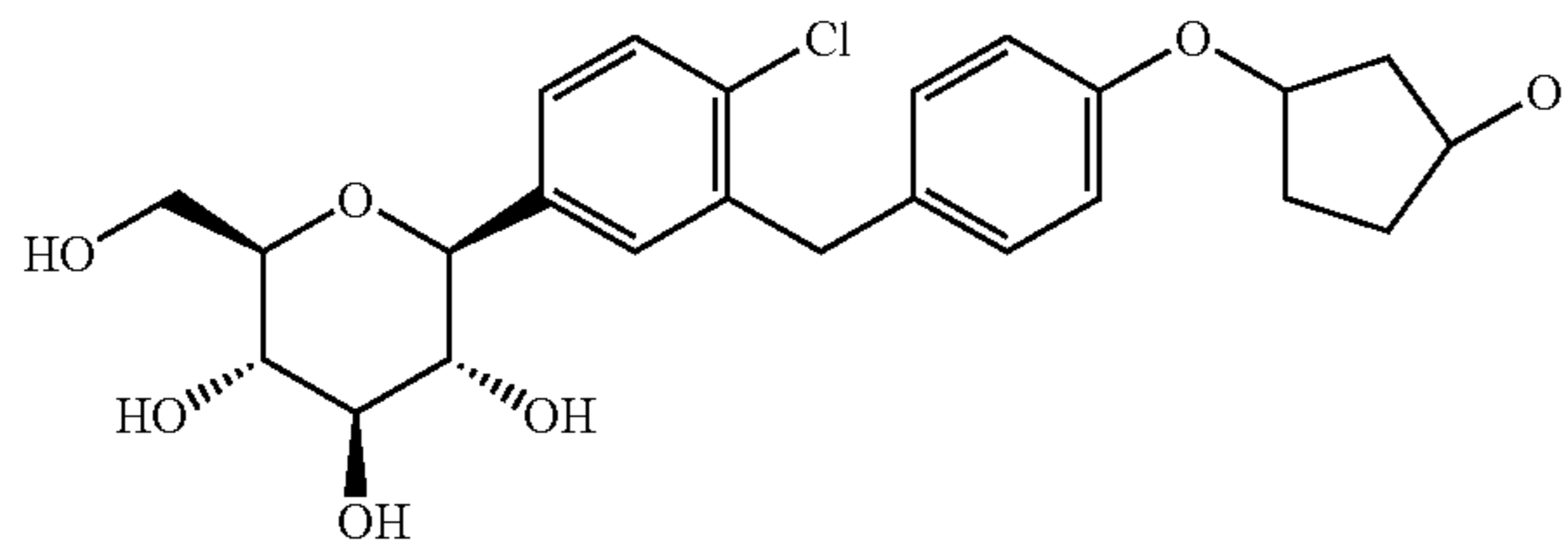
1-Chloro-4-(β-D-glucopyranos-1-yl)-2-[4-(3-hydroxy-cyclopent-1-yloxy)-benzyl]-benzene
