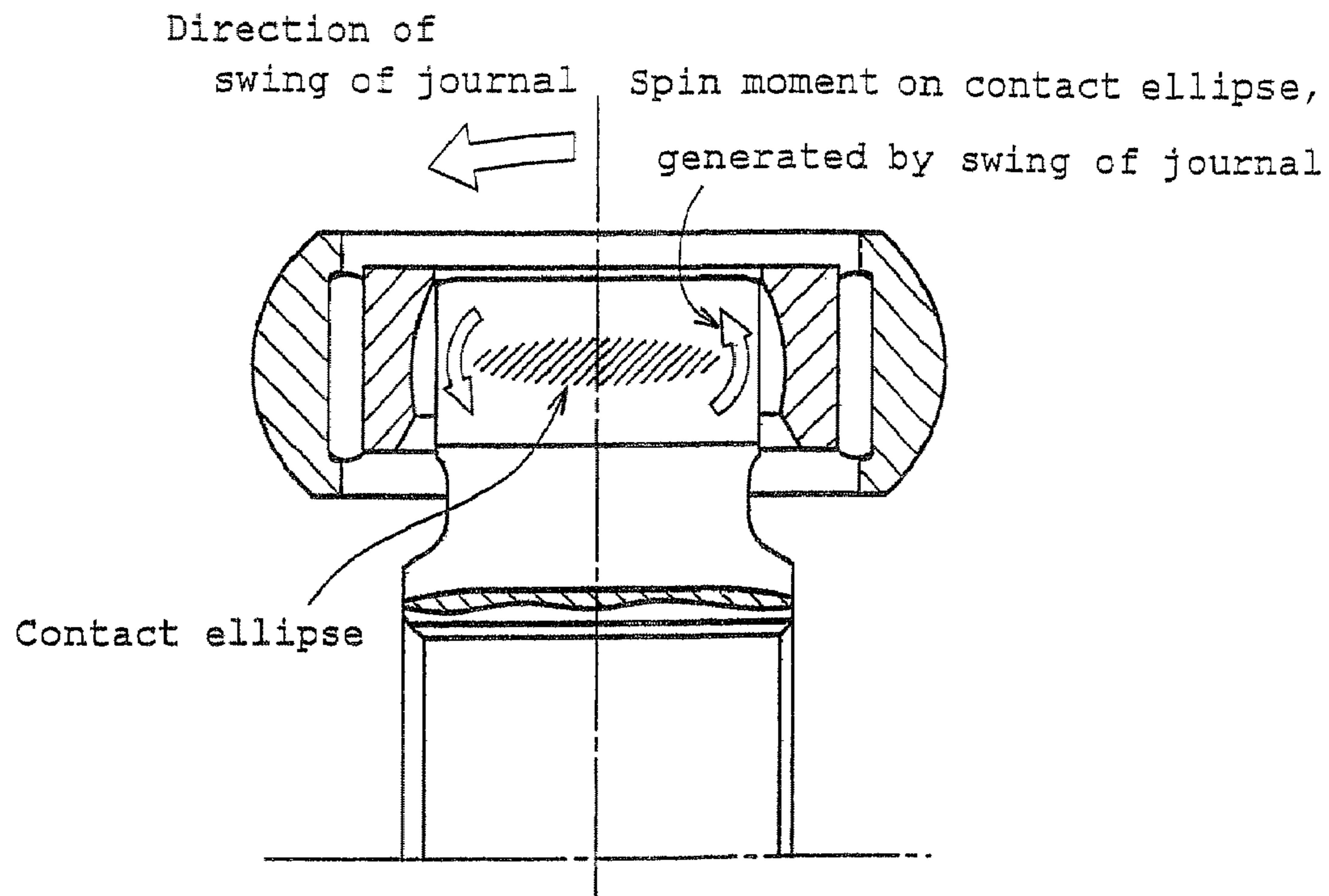
Fig. 18 PRIOR ART
