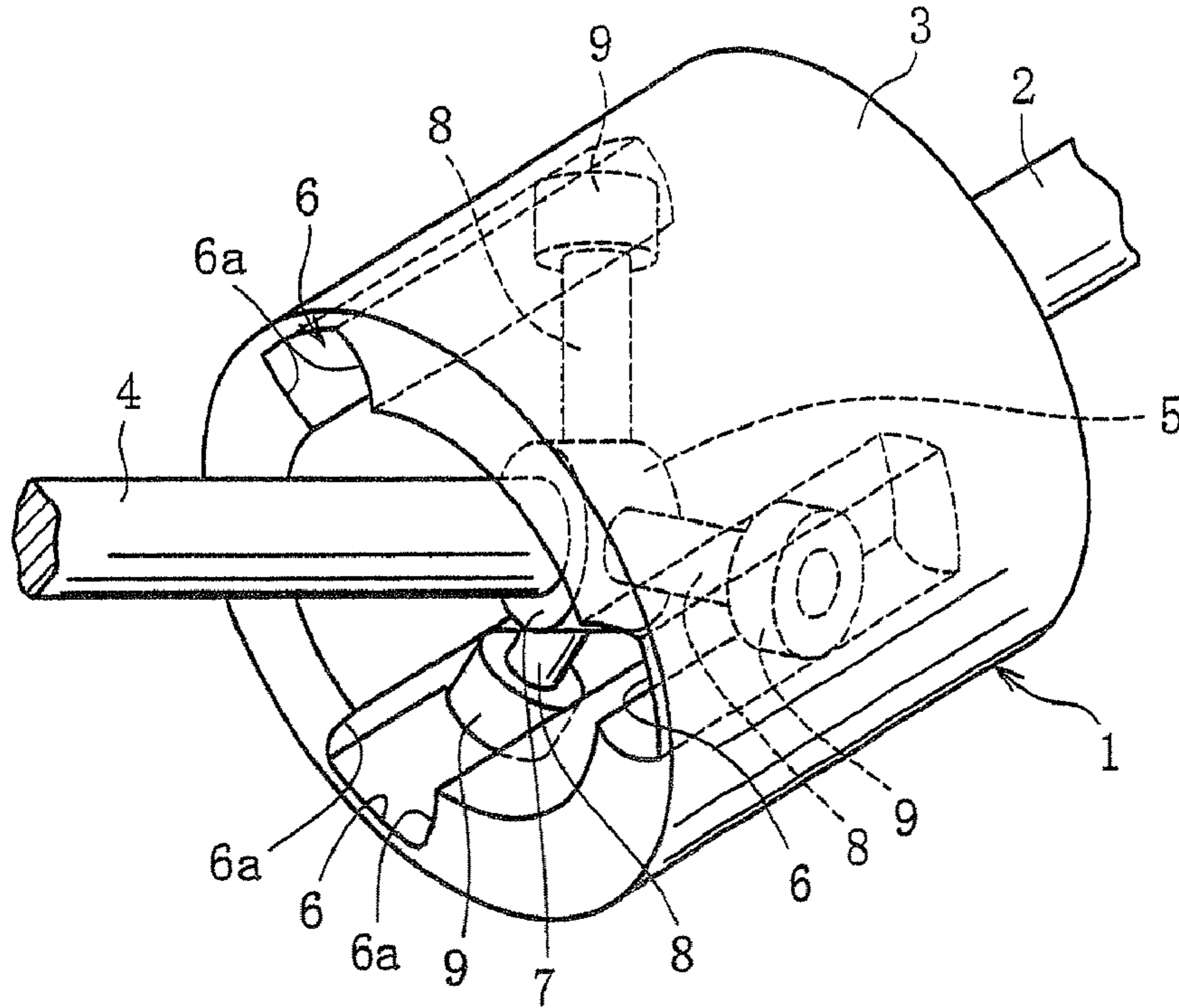
Fig. 16 PRIOR ART
