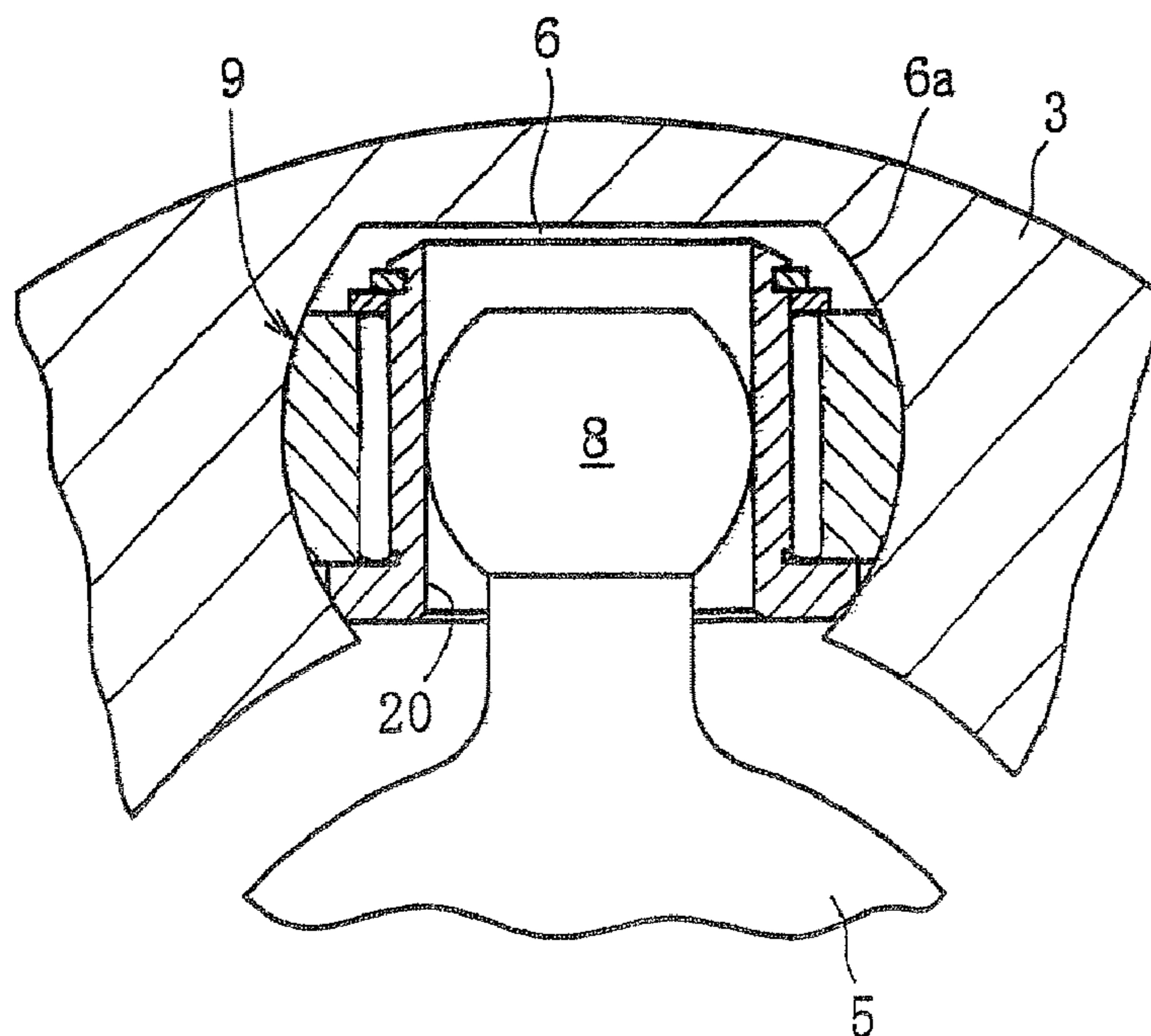
Fig. 19 PRIOR ART
