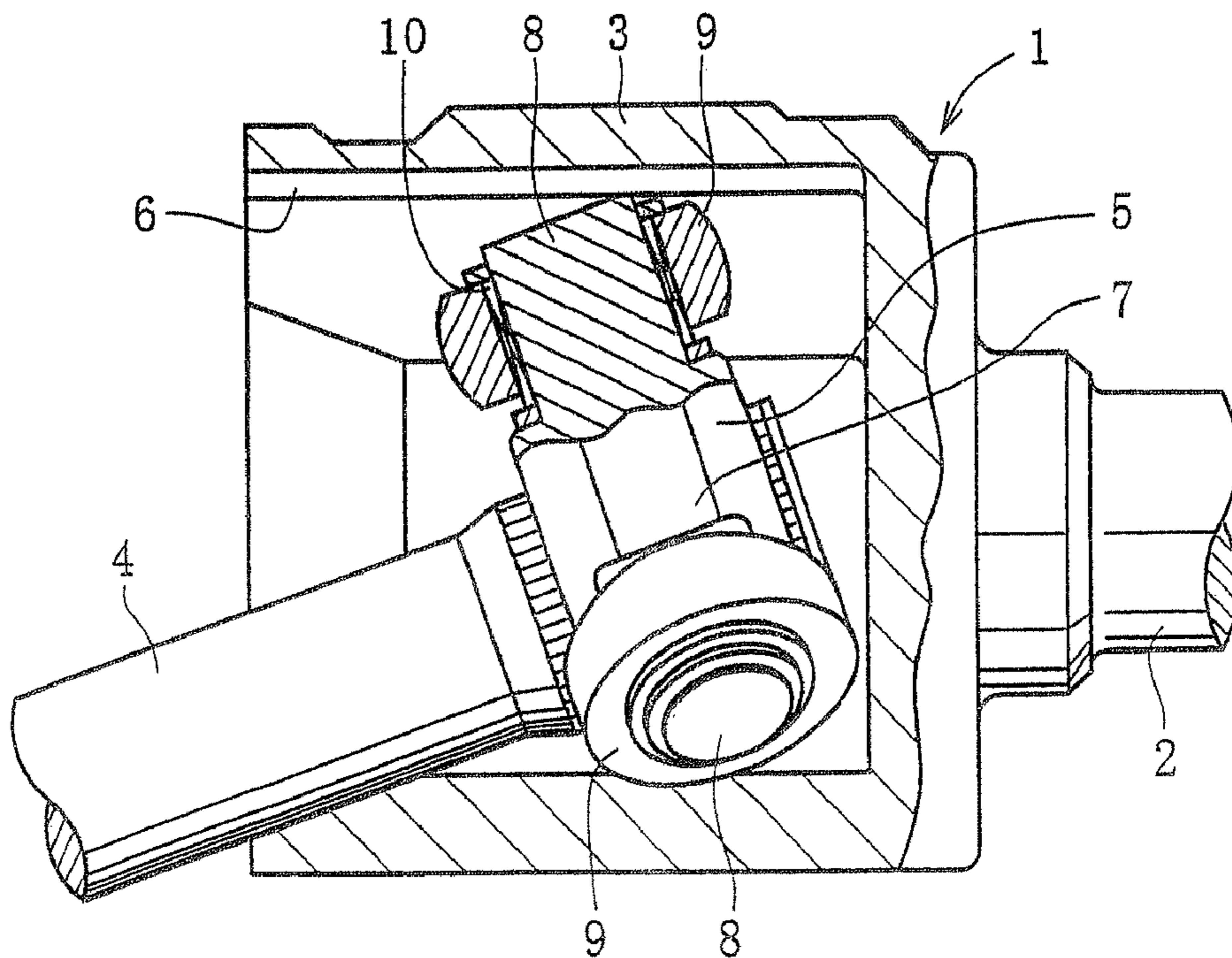
Fig. 16 PRIOR ART
