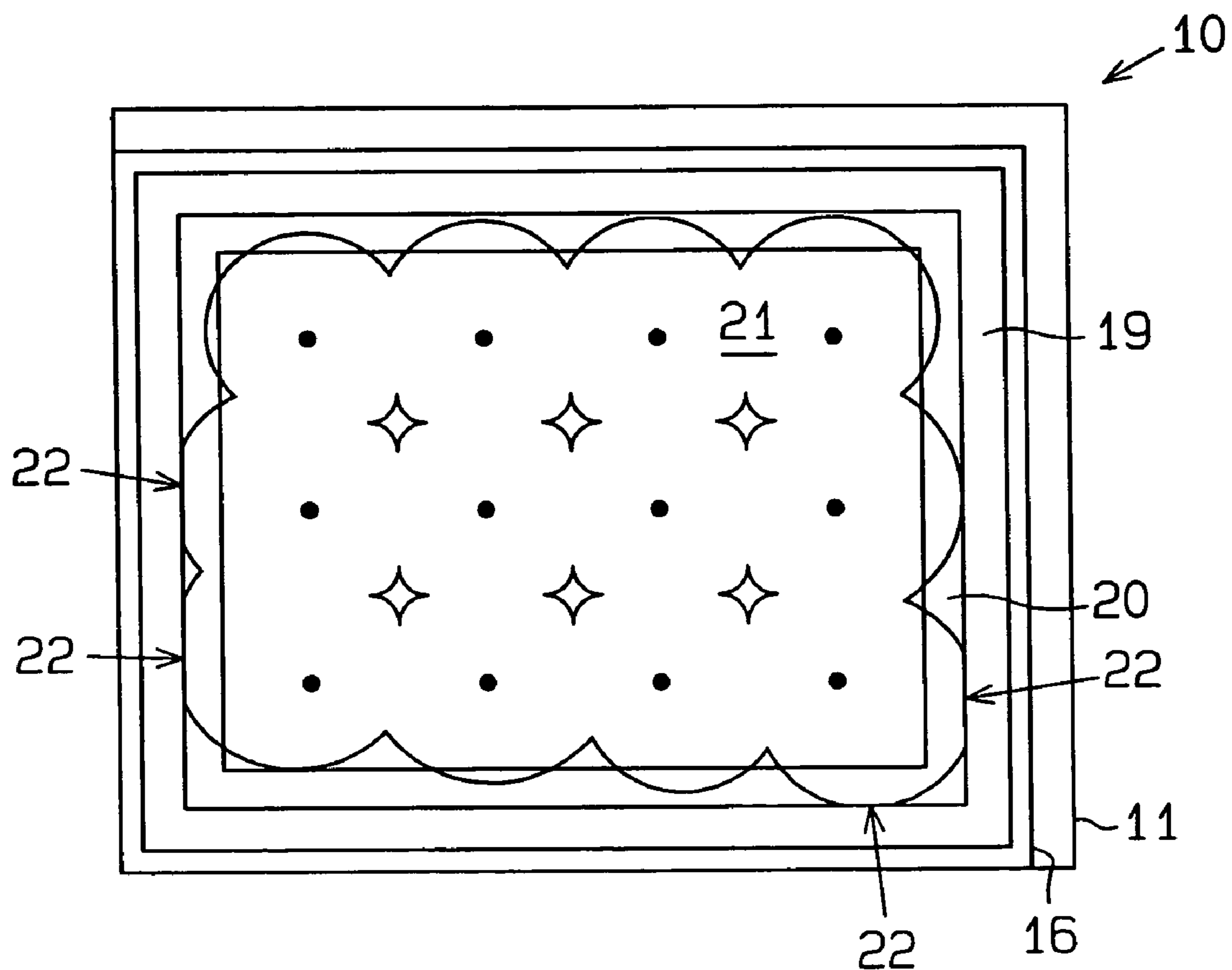
Fig.3 (Prior Art)
