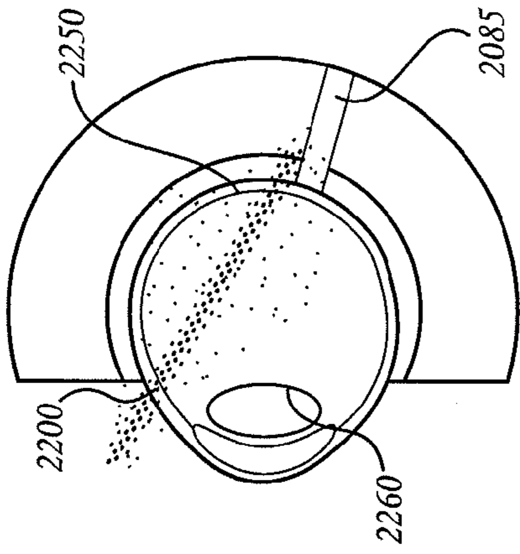
Beam 1 FIG. 7A
