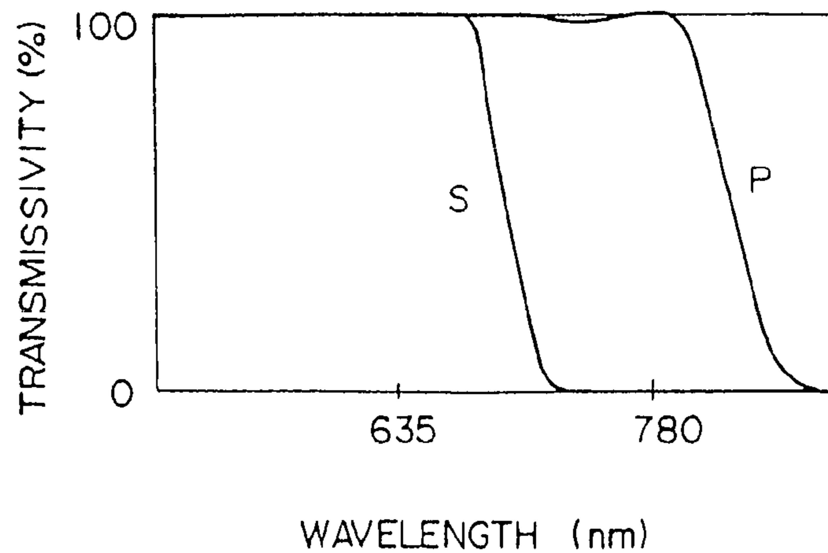
WAVELENGTH-DEPENDENT POLARIZING FILTER CHARACTERISTIC
