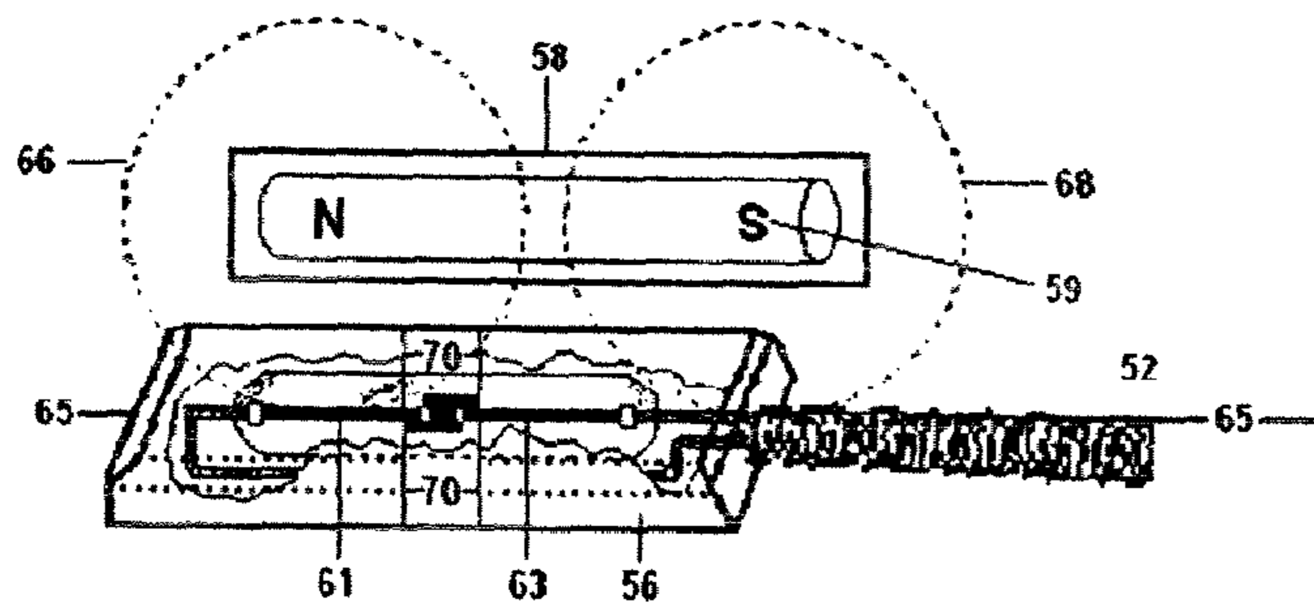
FIG 6C Normal Circuit PRIOR ART
