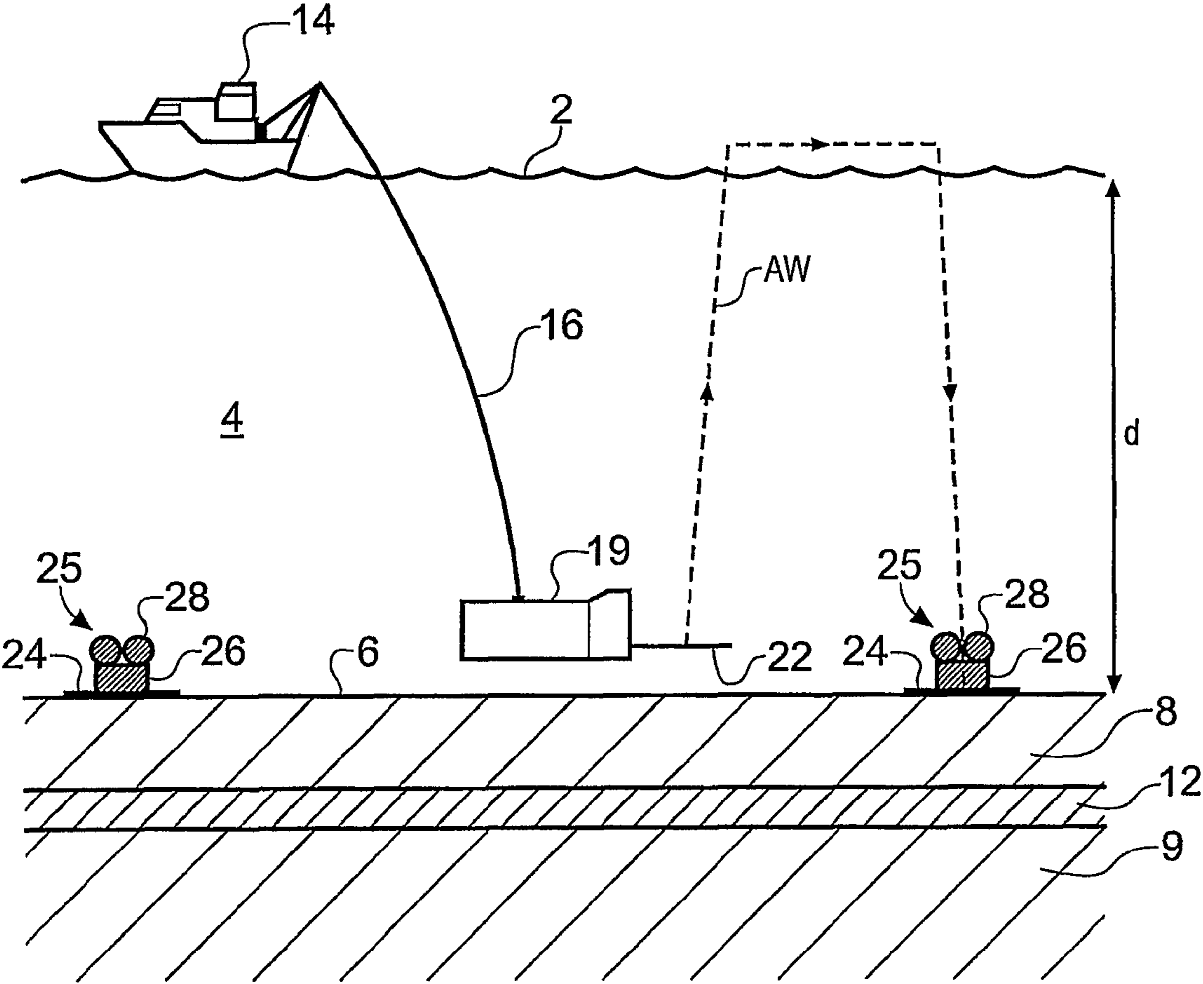
Fig. 1 PRIOR ART
