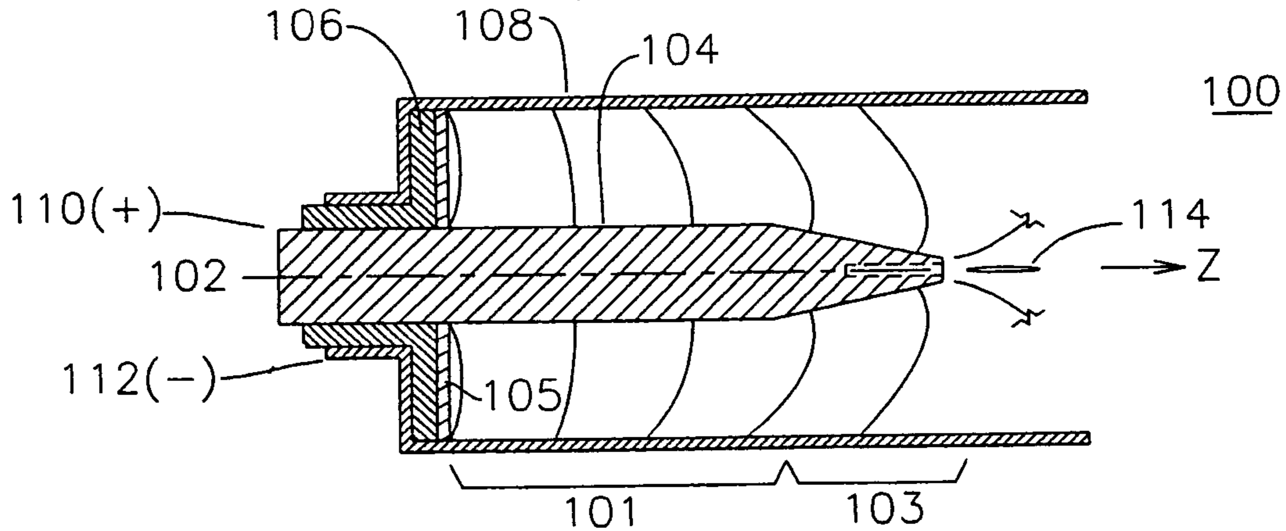
Figure 7a: Conical Anode & Cylindrical Cathode, Radial Ignition
