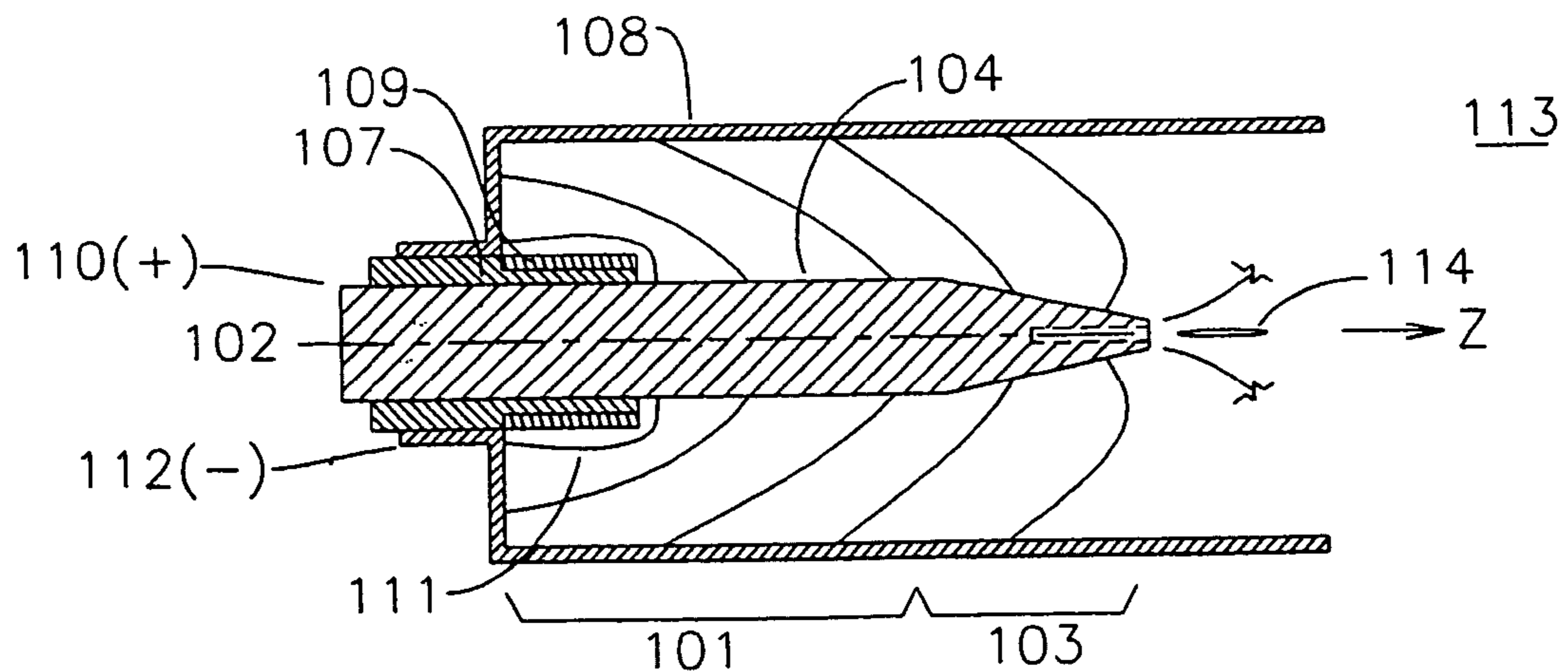
Figure 7b: Conical Anode & Cylindrical Cathode, Axial Ignition
