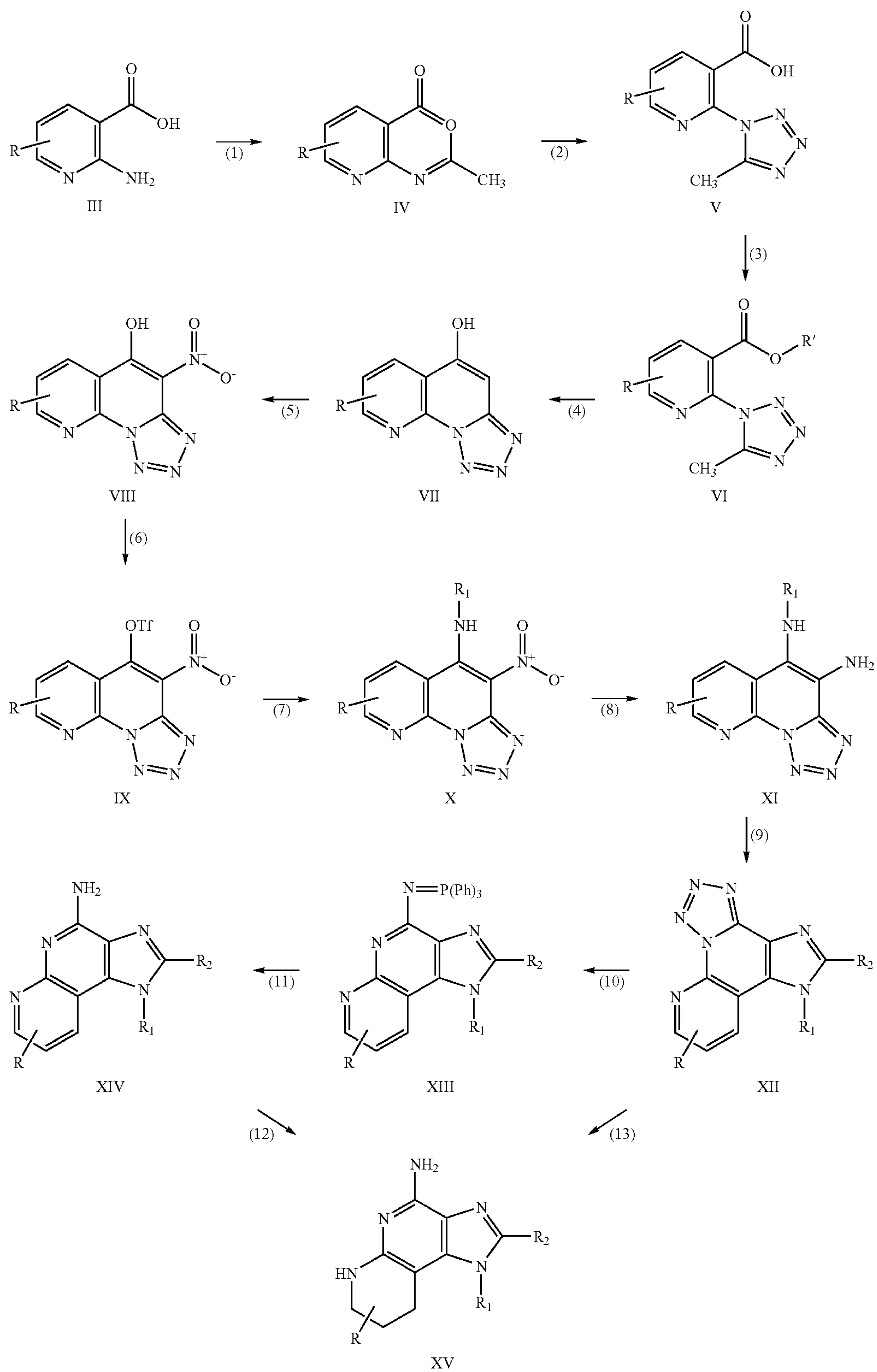
Reaction Scheme 1
