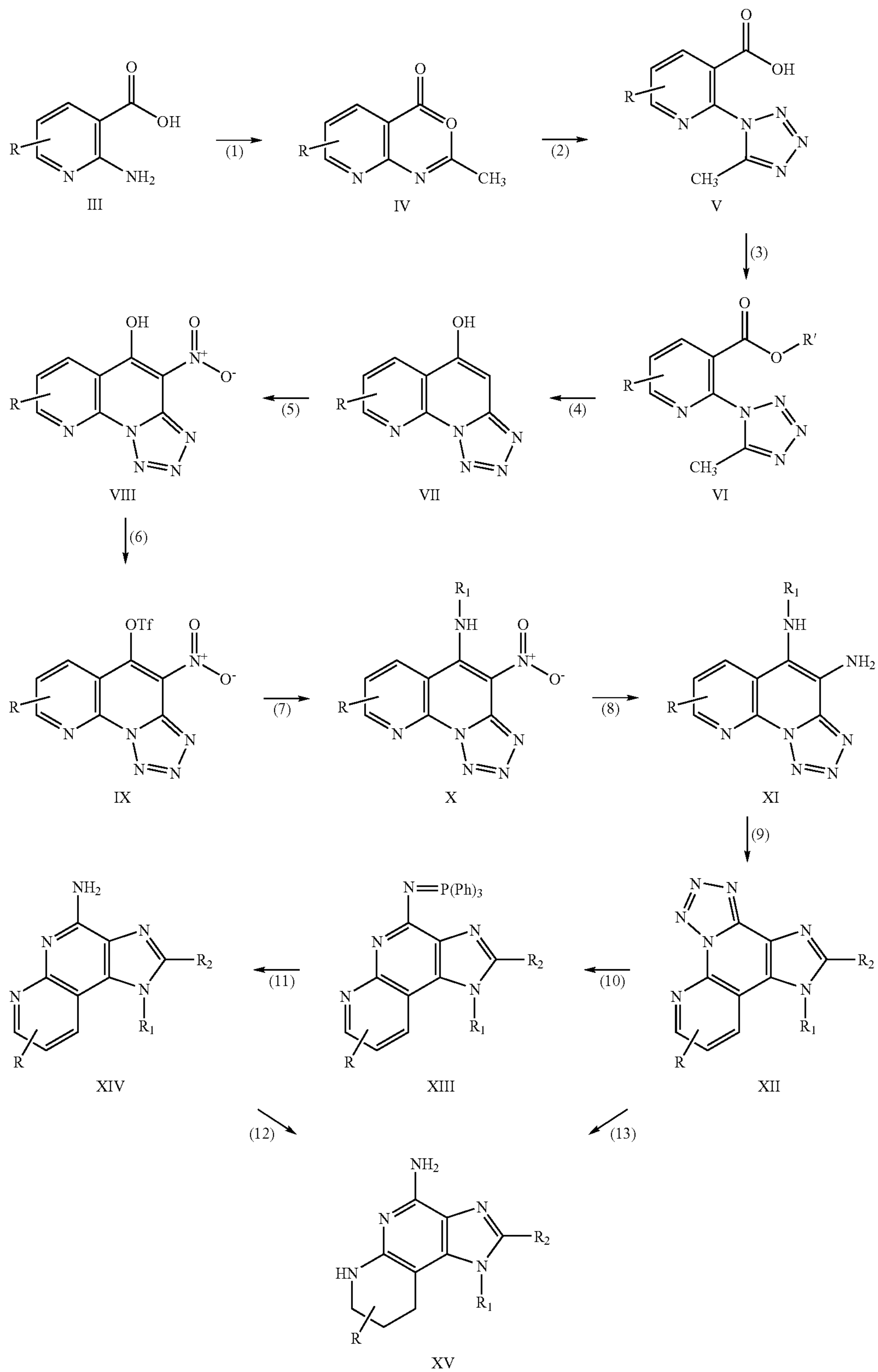
Reaction Scheme 1
