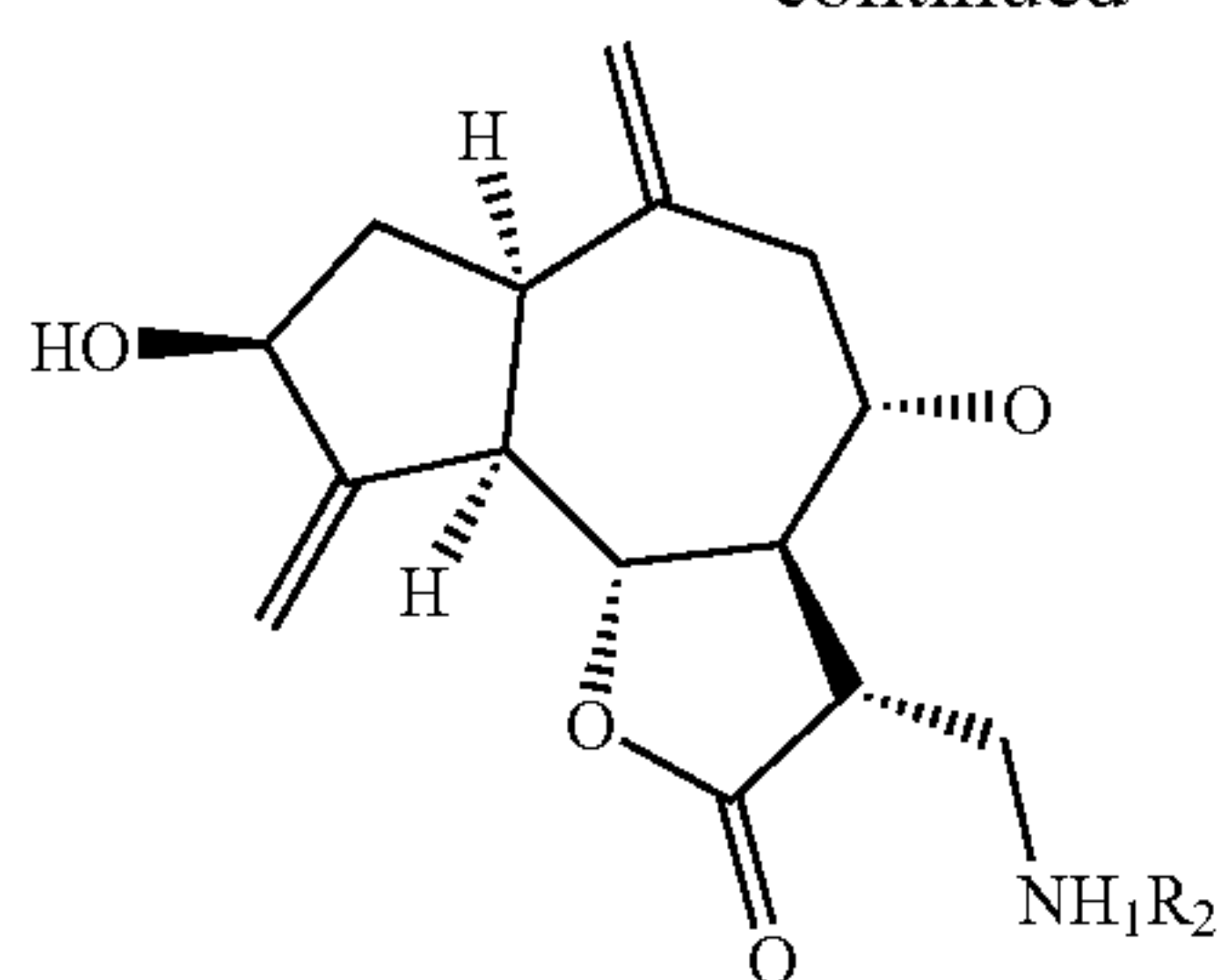
Aminodesacylcynaropicrins
