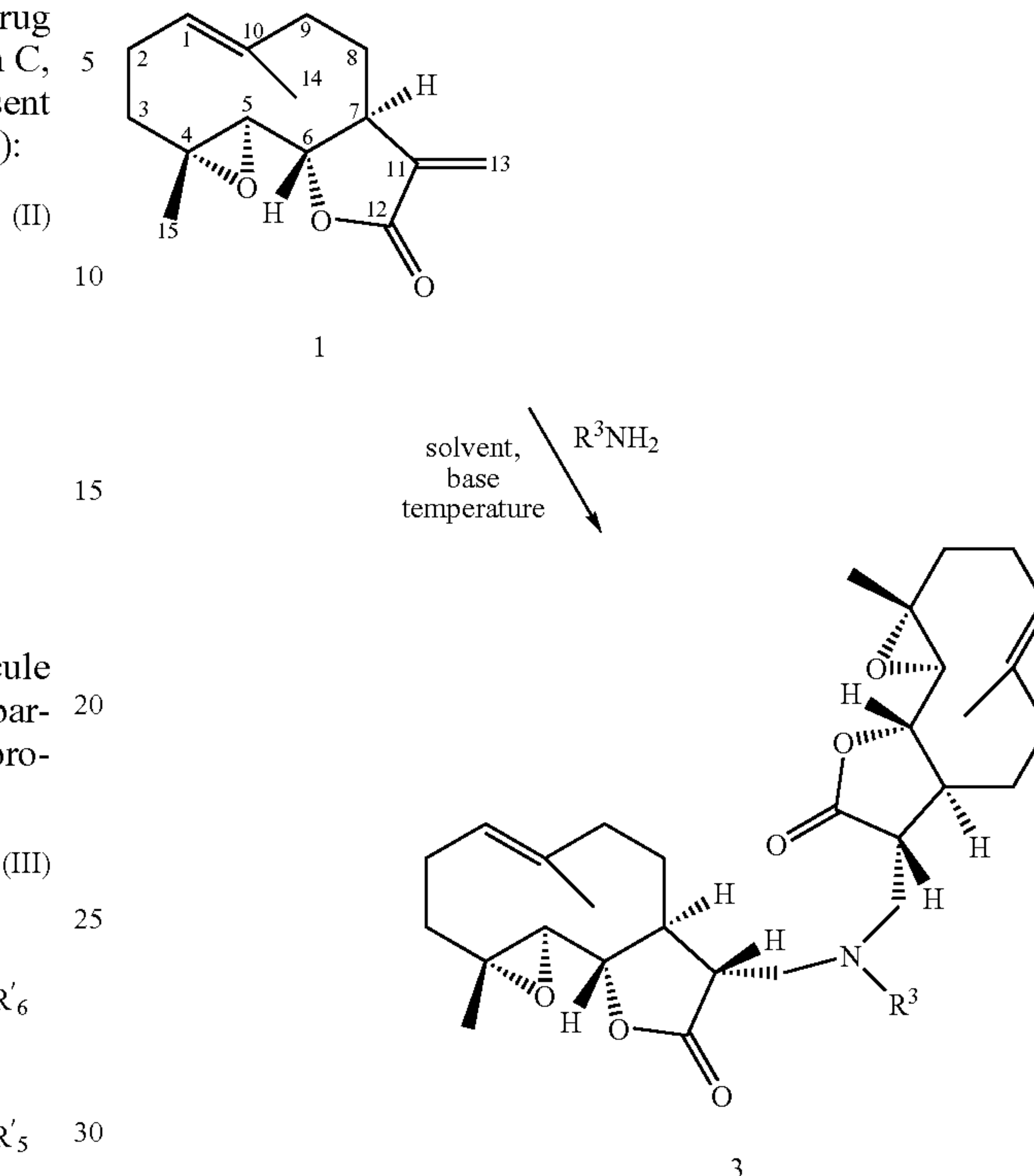
Scheme II
