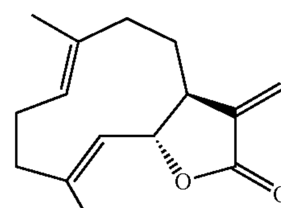
Costunolide
