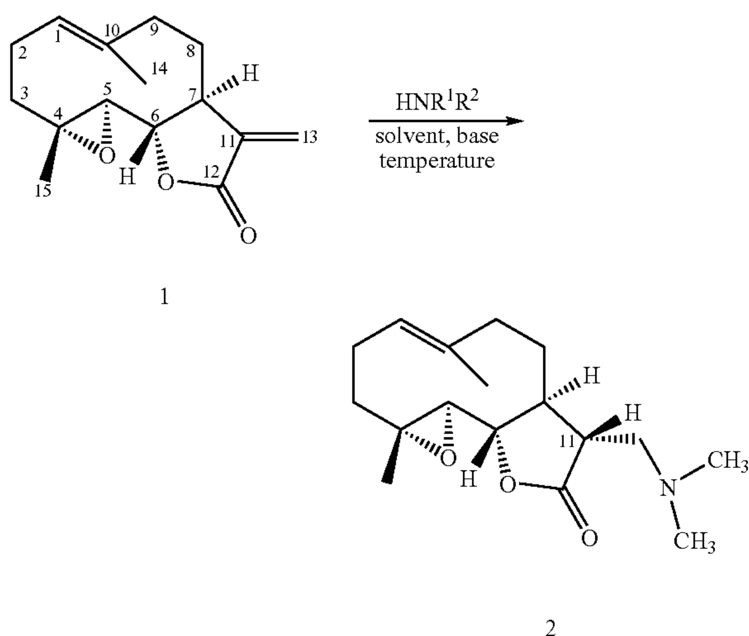
Scheme I
