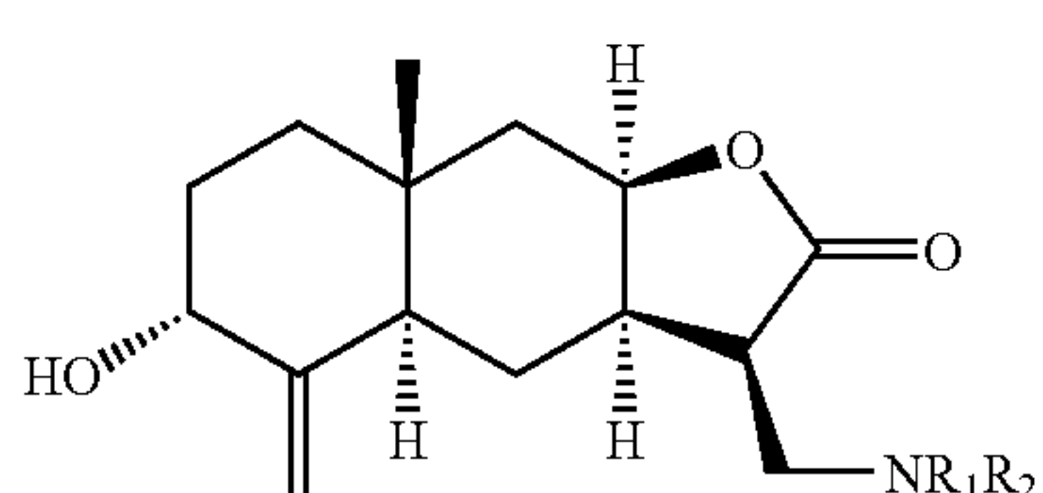
Aminoisotelekins
