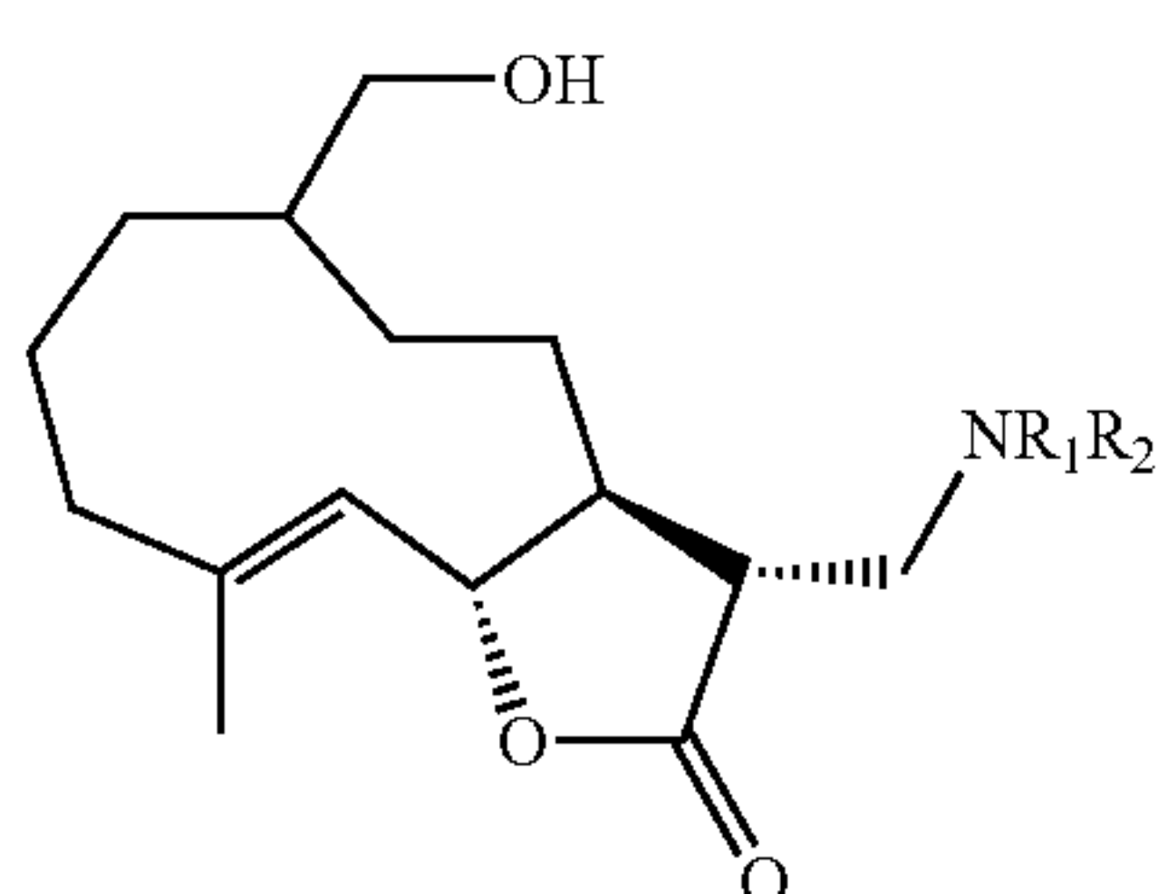
Aminosoulangianolides
