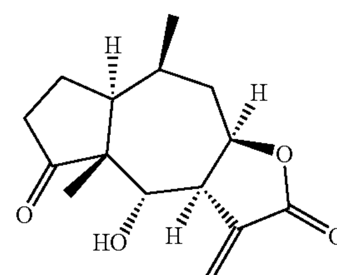
11, 13-Dihydrohelenalin
