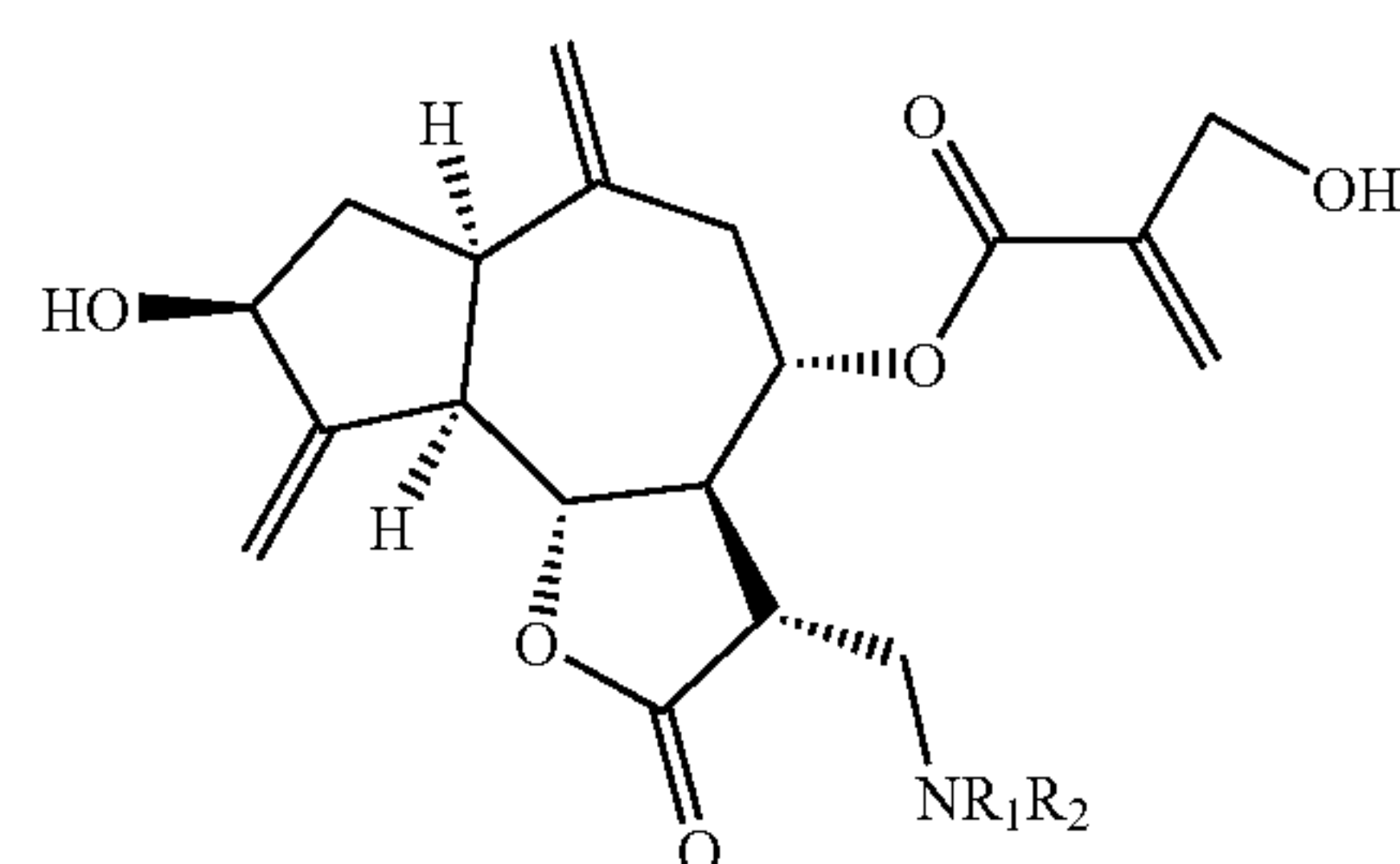
Aminocyanaropicrins
