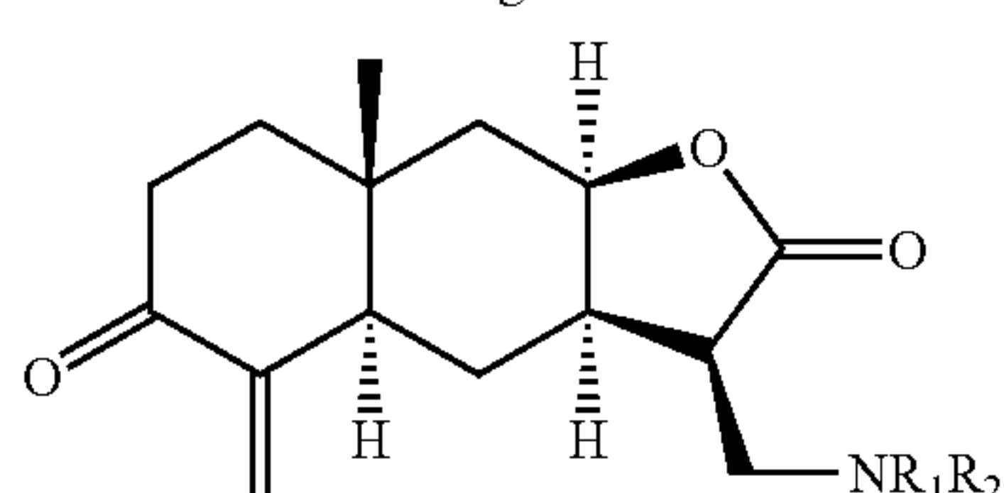
Aminosoulangianolides
