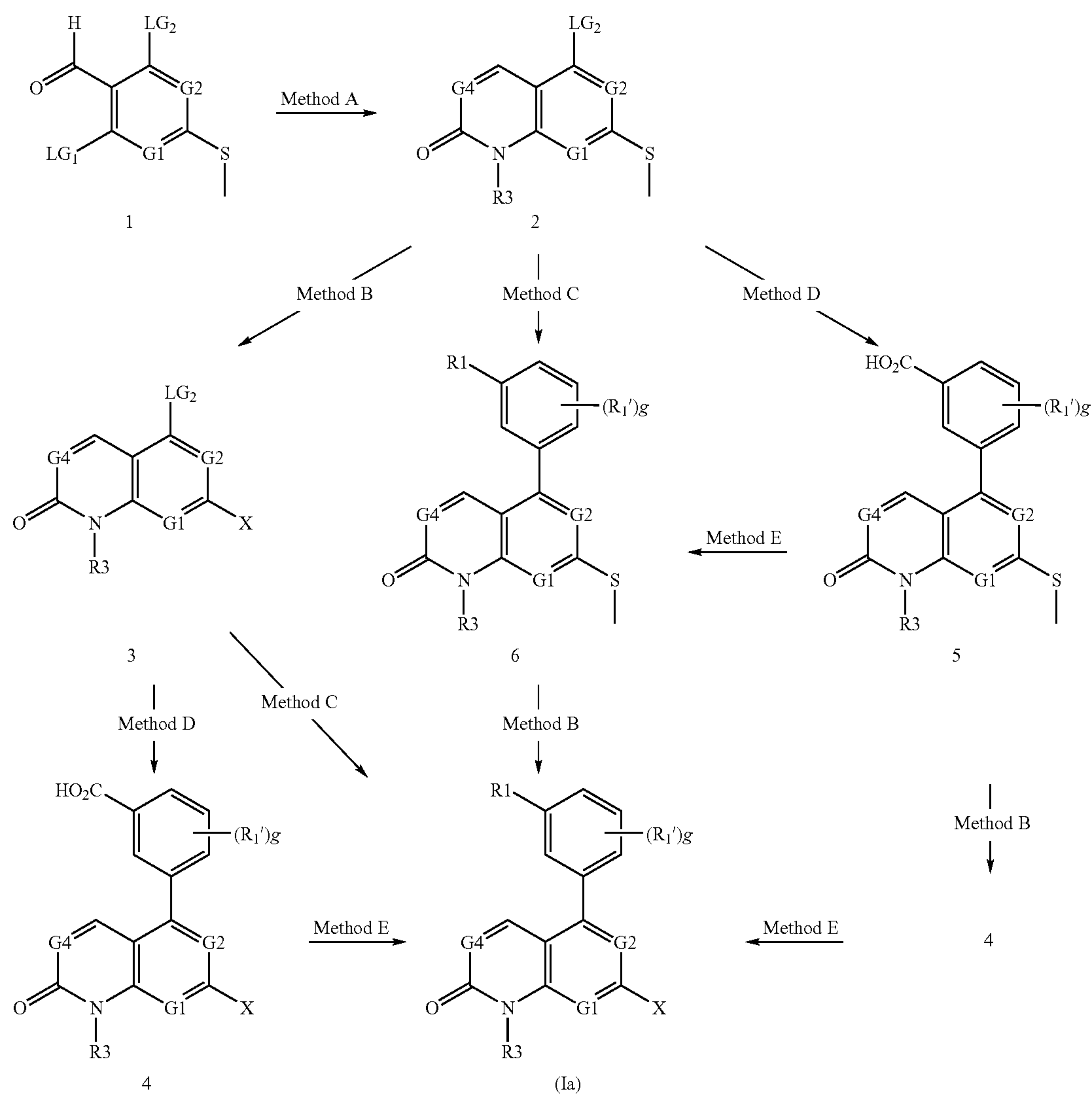
Scheme 1
