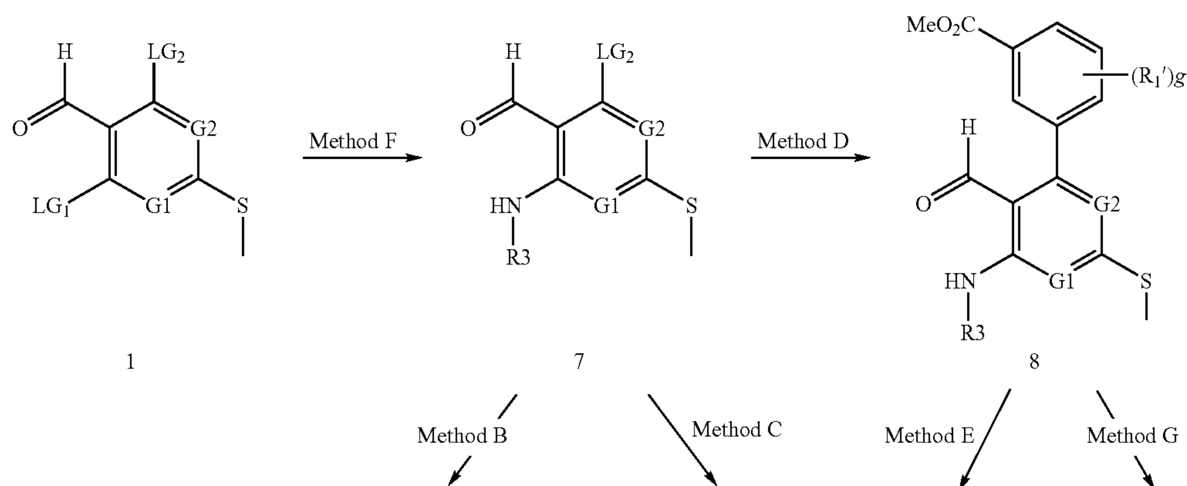
Scheme 2
