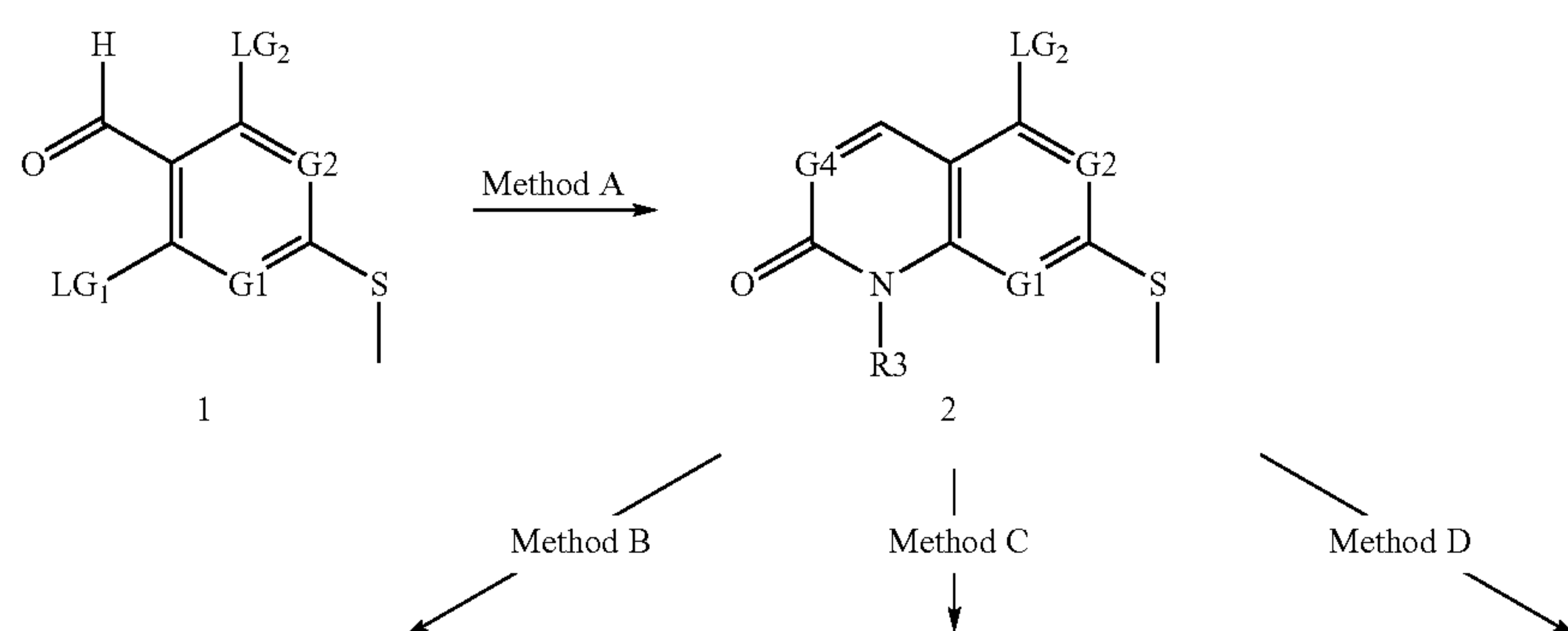
Scheme 5
