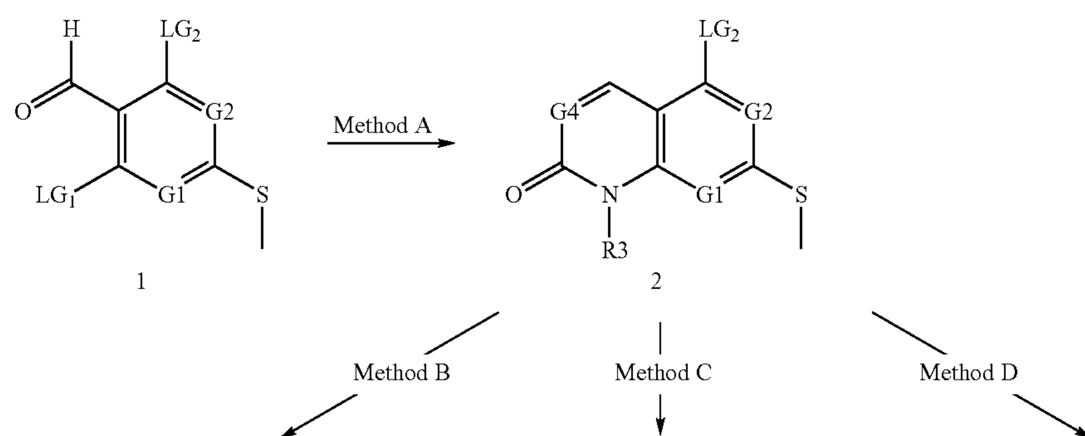
Scheme 4
