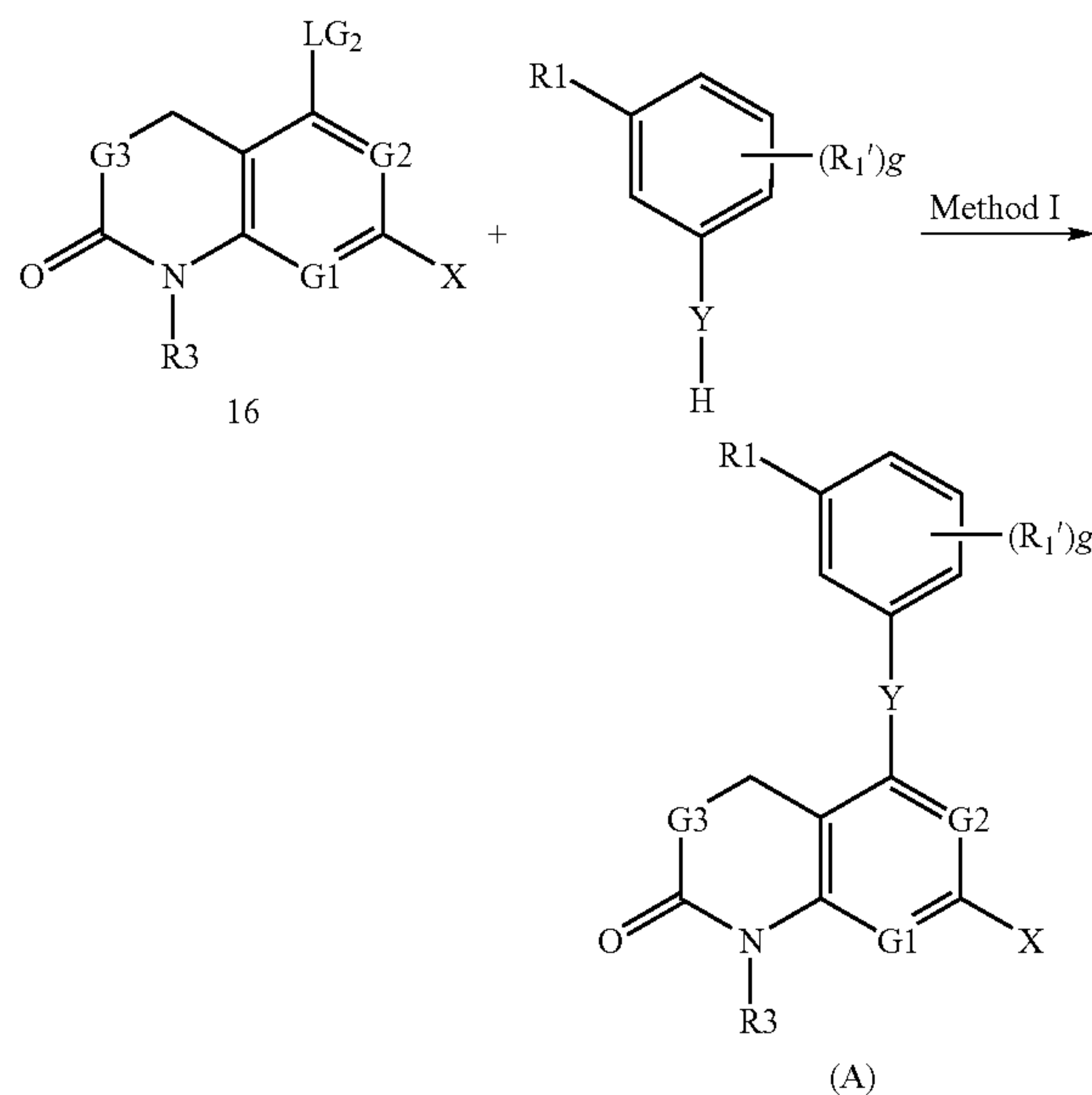
Scheme 9
