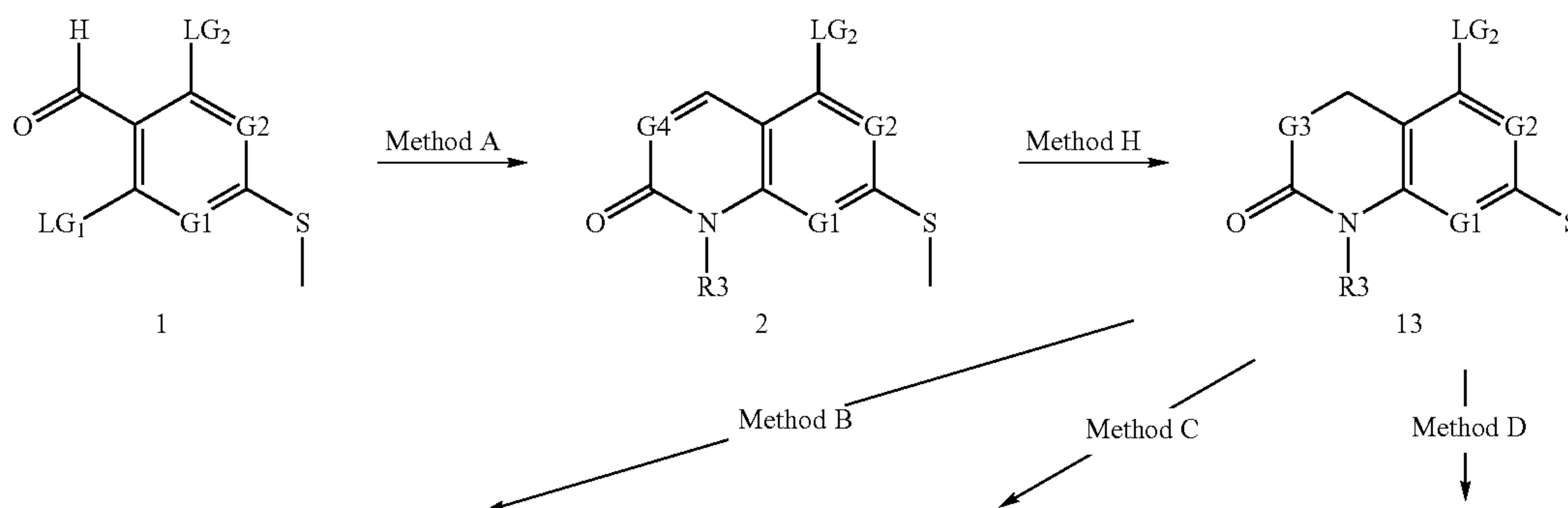
Scheme 3
