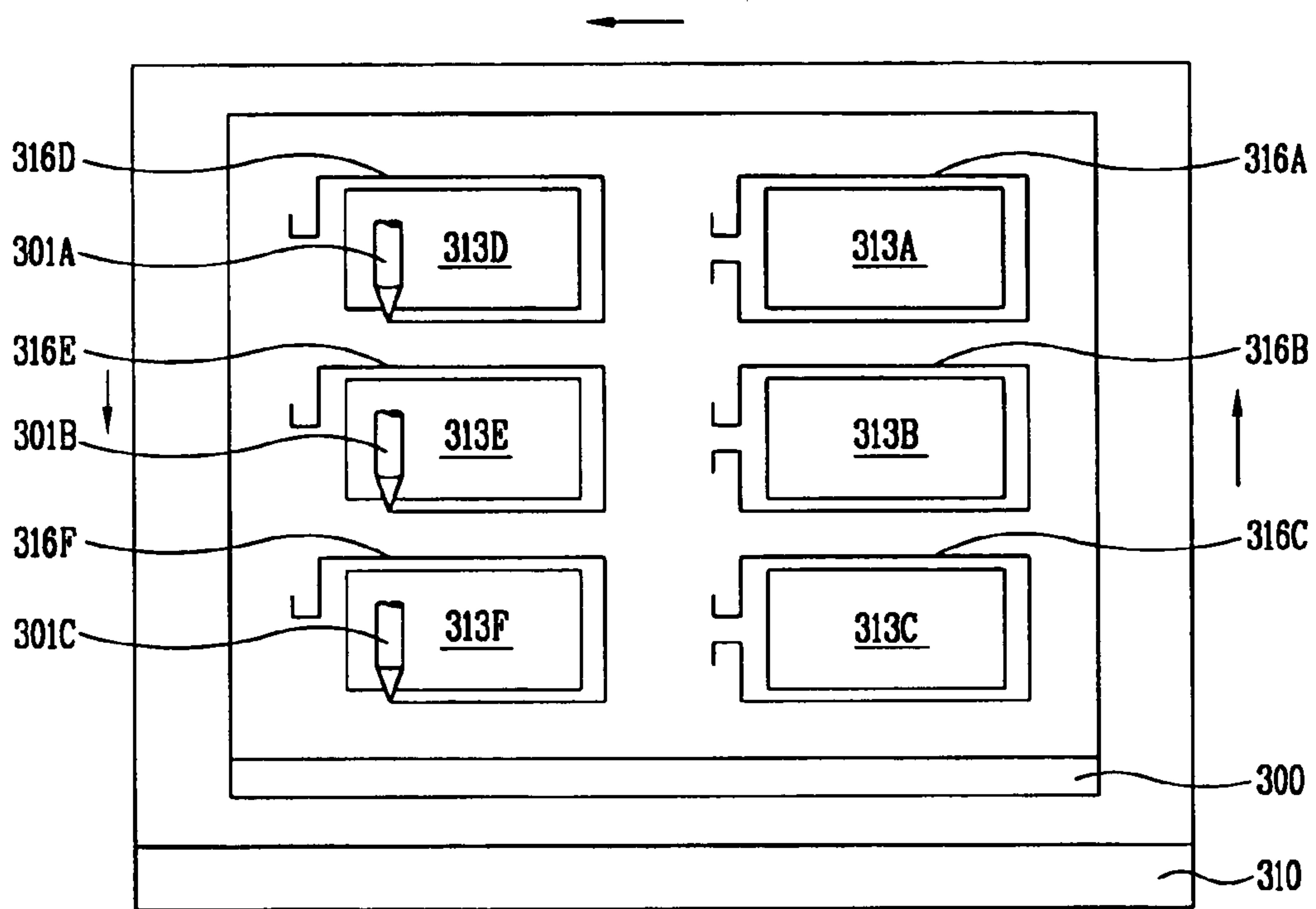
FIG. 3 RELATED ART
