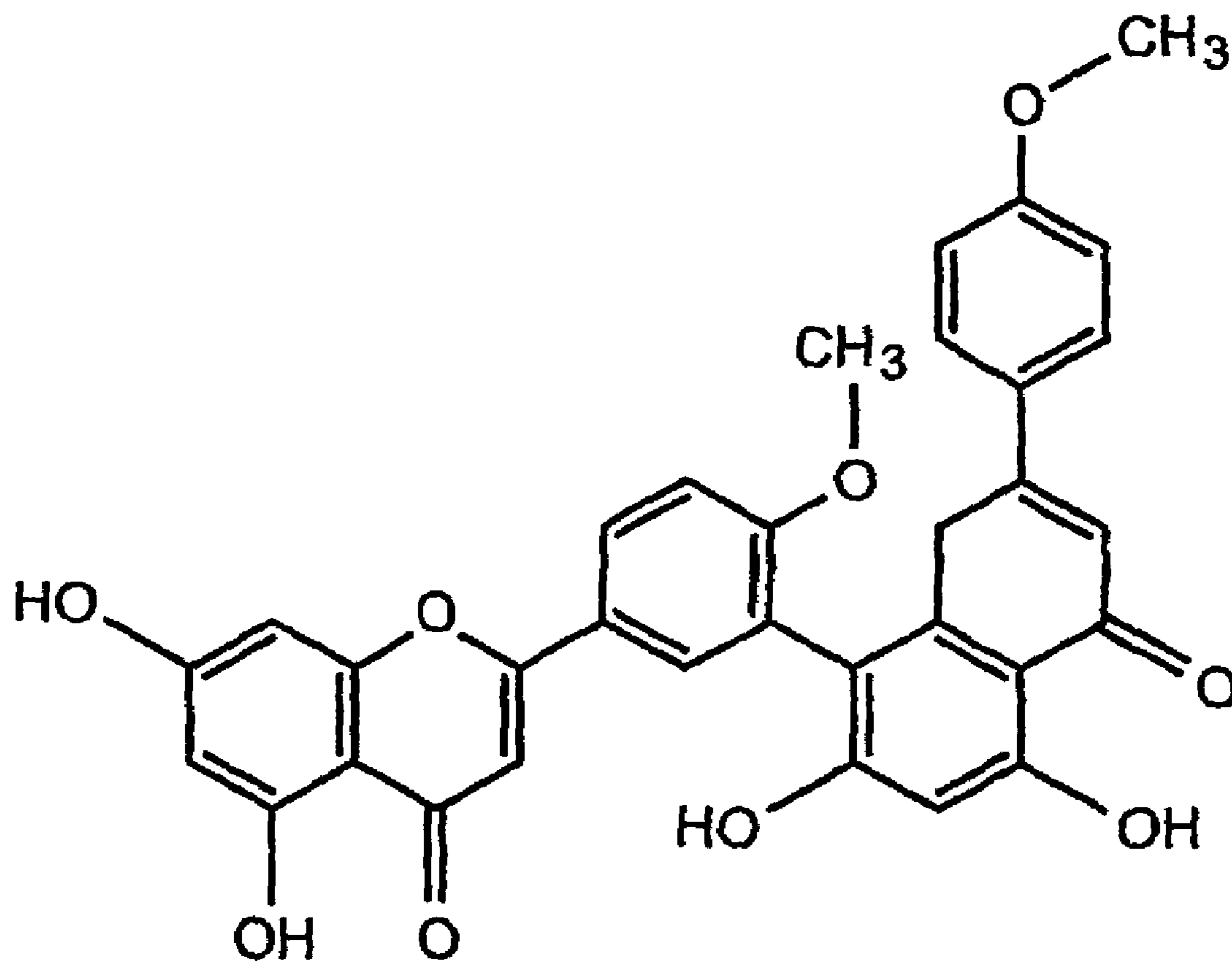
2-{3-[2,4-Dihydroxy-7-(4-methoxy-phenyl)-5-oxo-5,8-dihydro-naphthalen-1-yl]-4-methoxy-phenyl}-5,7-dihydroxy-chromen-4-one
