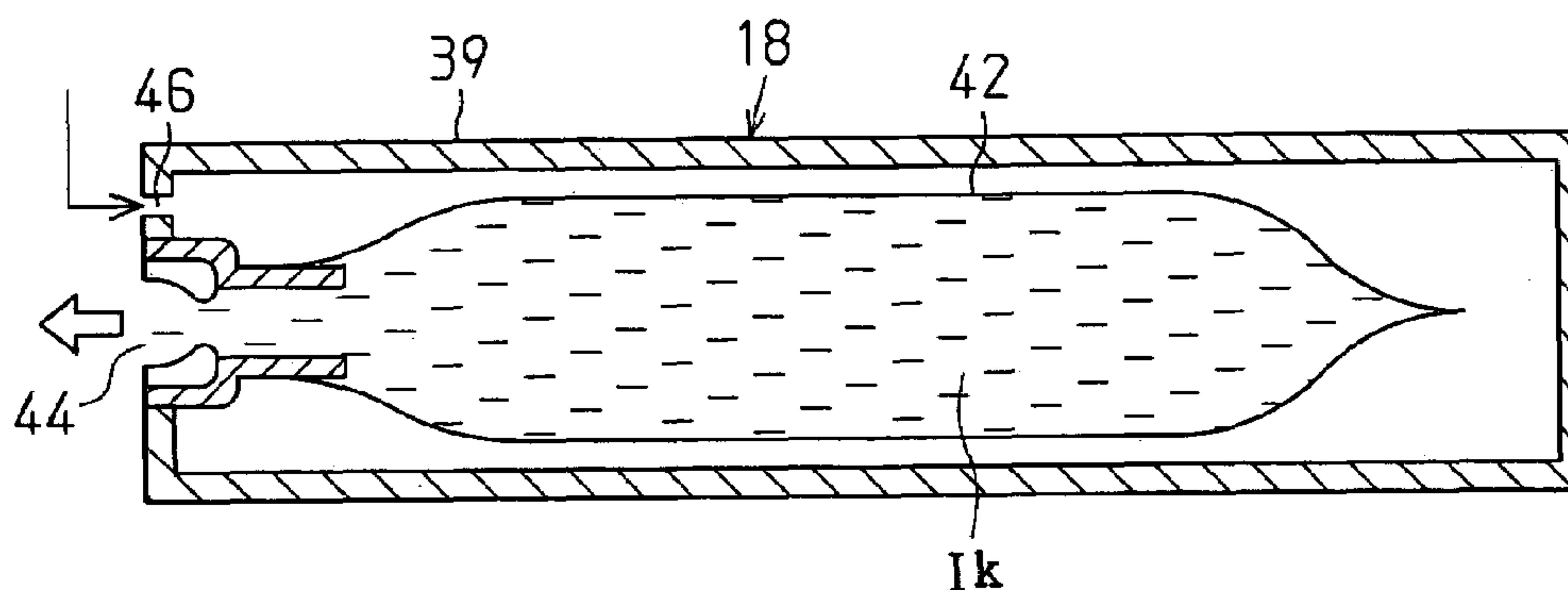
Fig.25 (Prior Art)
