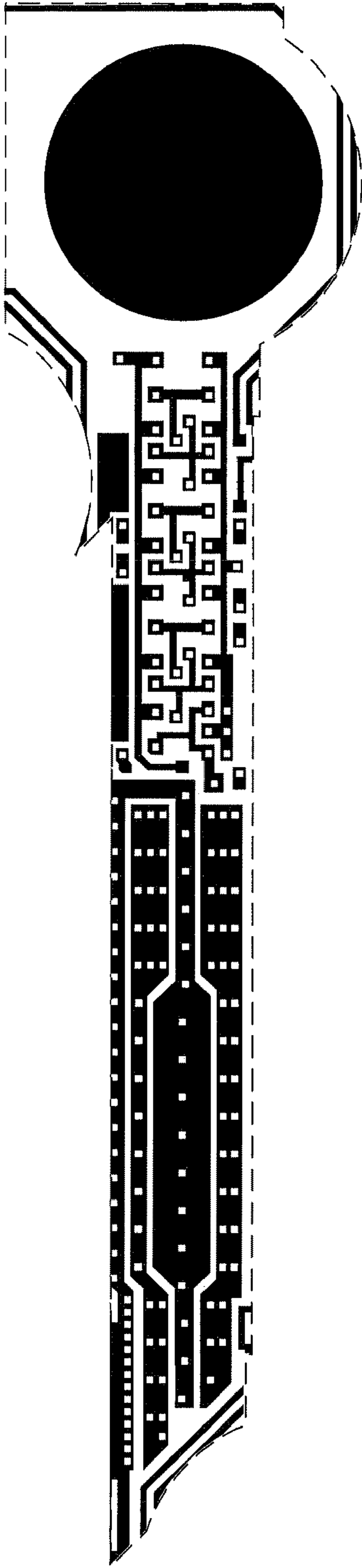
Metal 1 mask
