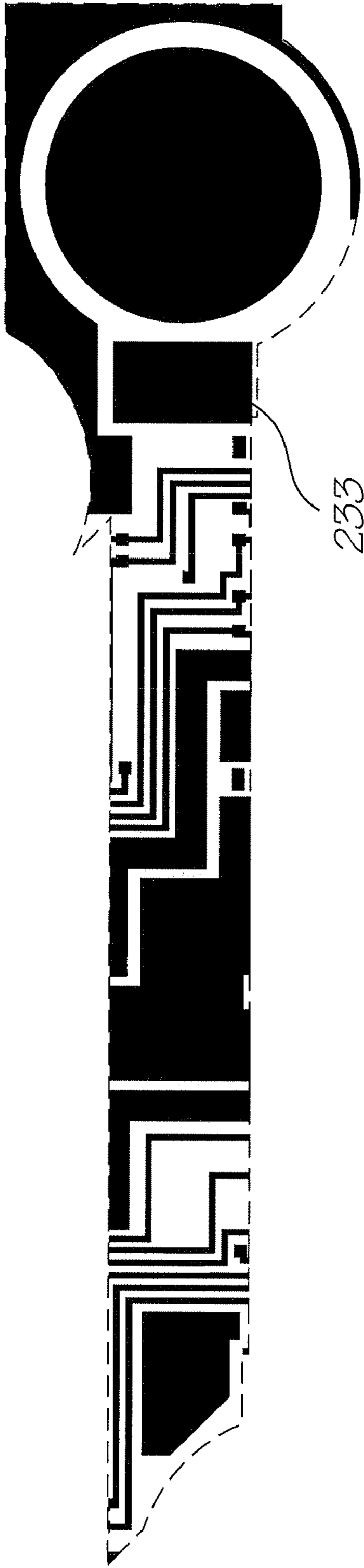
Metal 2 mask
