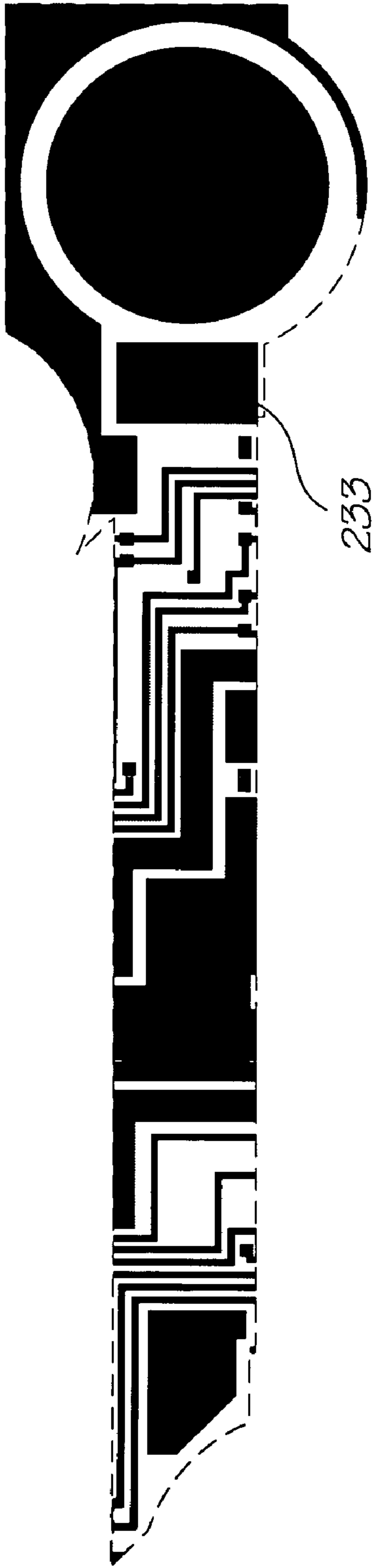
Metal 2 mask
